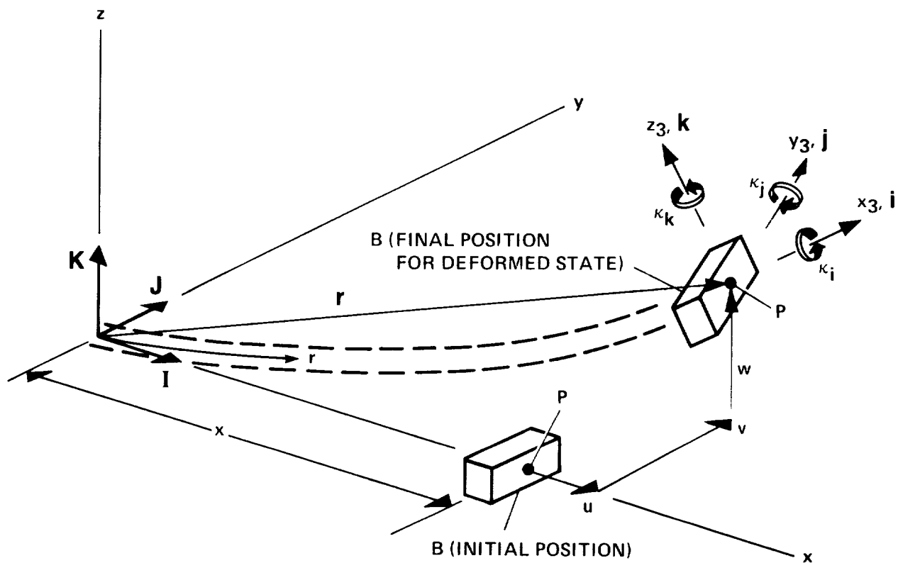
Figure 2.- Deformed-beam geometry.
