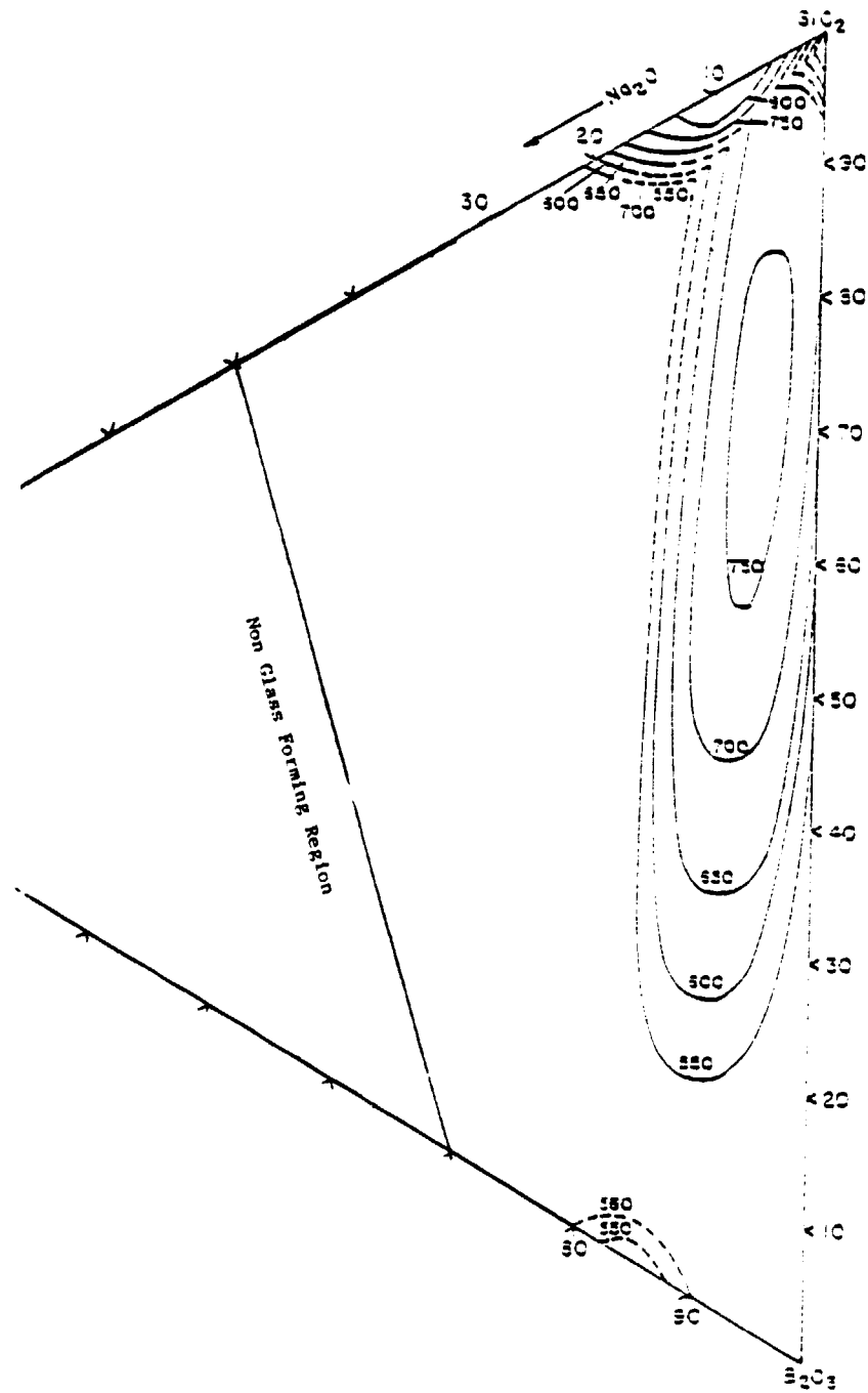
FIGURE 1. \text{Na}_2\text{O}-\text{B}_2\text{O}_3-\text{SiO}_2 TERNARY DIAGRAM SHOWING THE PROJECTION OF THE IMMISCIBILITY SURFACE AT DIFFERENT TEMPERATURES (11)
