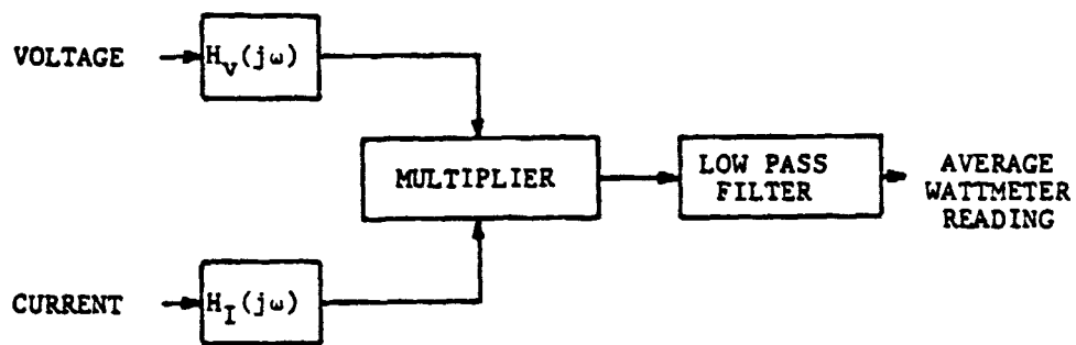
FIGURE 1. General block diagram of a wattmeter.
