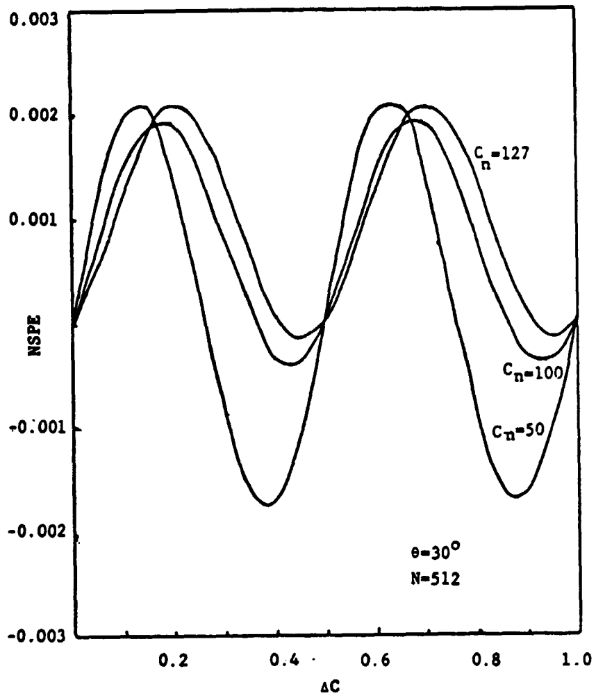
FIGURE 6. Normalized sampled power error versus scanning parameter ( C_n = 50, 100, \text{ and } 127 ).
