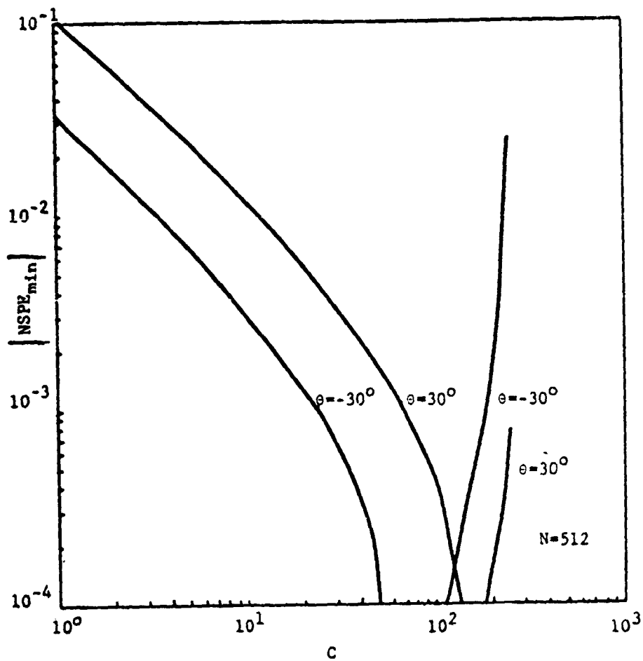
FIGURE 8. The magnitude of the minimum value of the normalized sampled power error versus periods of observation.
