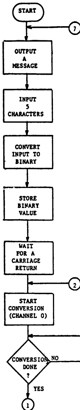
FIGURE 14-a. Flow chart for a microcomputer wattmeter.
