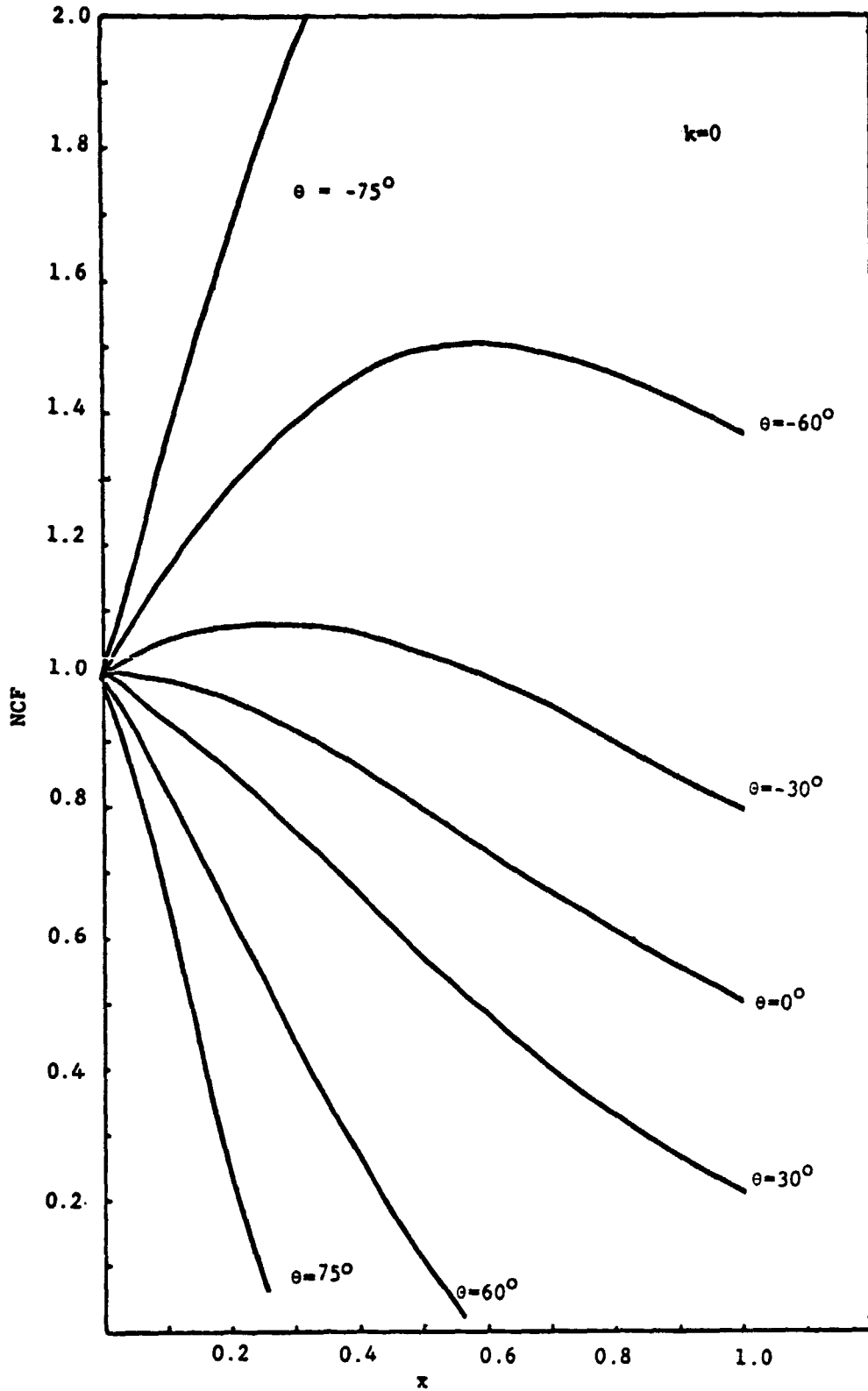
FIGURE 3 Normalized correction factor versus normalized frequency ( k=0 ).
