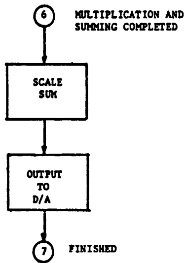
FIGURE 14-e. Flow chart for a microcomputer wattmeter (continued).
