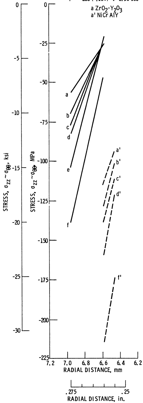
(a) LONGITUDINAL OR HOOP STRESS.
