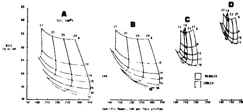
Figure 1 Cycle parametric effects on small engine performance
