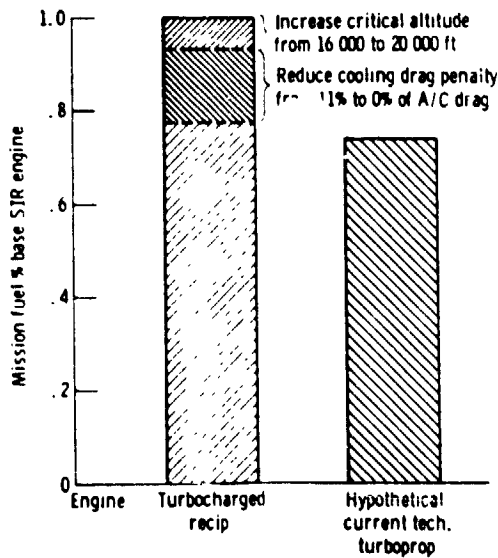
Figure 2 - Effect on mission fuel of increasing the critical altitude of a turbocharged spark ignition reciprocating engine and reducing the engine cooling drag Medium twin-engine airplane. Range - 1370 n. mi. 234 knots at 25 000 ft.
