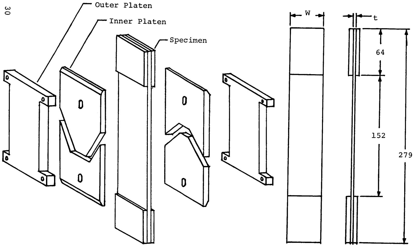
Figure 2.- Exploded view of face-supported fixture with specimen and sketch of specimen.
