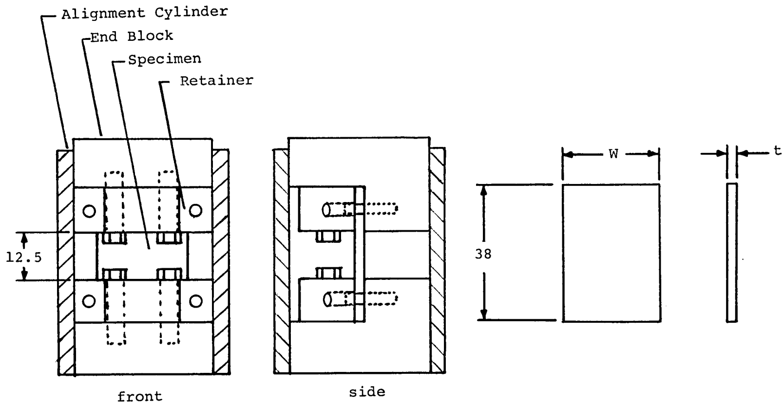
Figure 3.- Sketch of end-loaded-coupon fixture and specimen.
