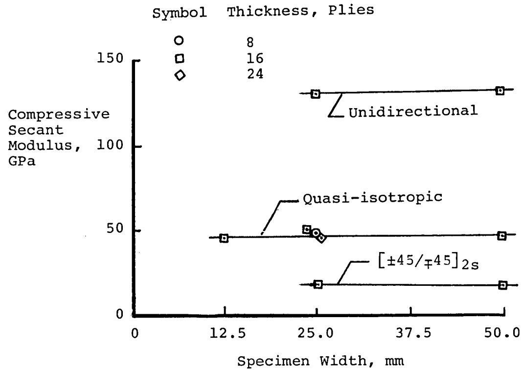
Figure 11(b).- Secant modulus at .004 strain of Gr/Ep composite material as a function of specimen width and thickness for specimens tested with the face-supported fixture.
