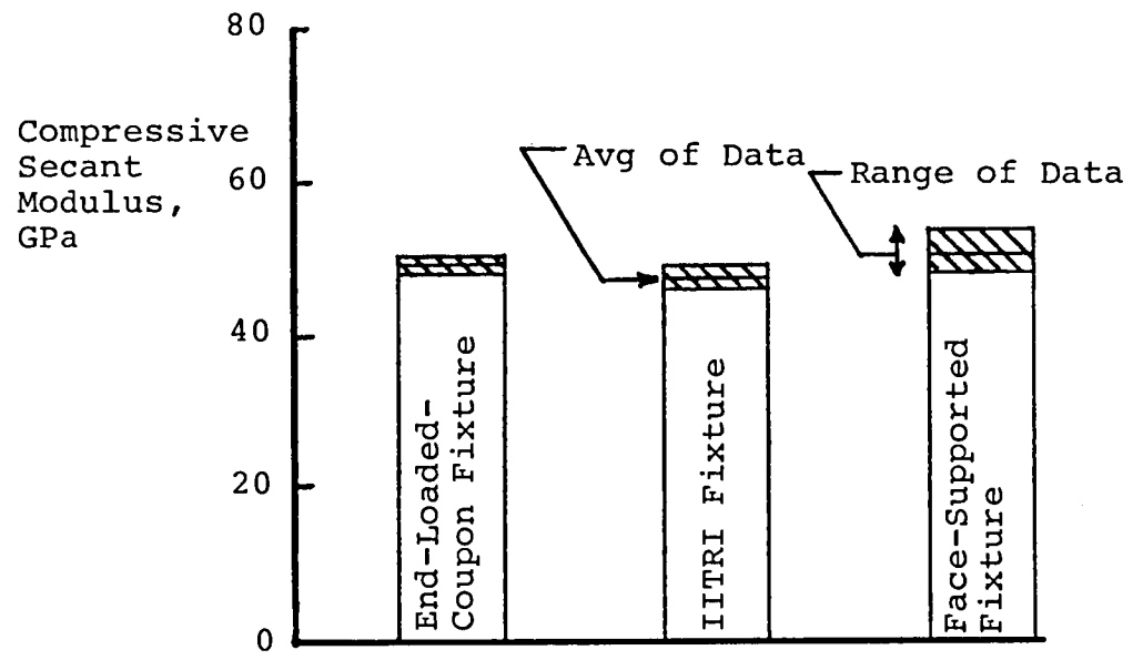
Figure 12.- Secant modulus at .004 strain of 25-mm wide 16-ply thick quasi-isotropic Gr/Ep specimens tested with the end-loaded, IITRI, and face-supported fixtures.
