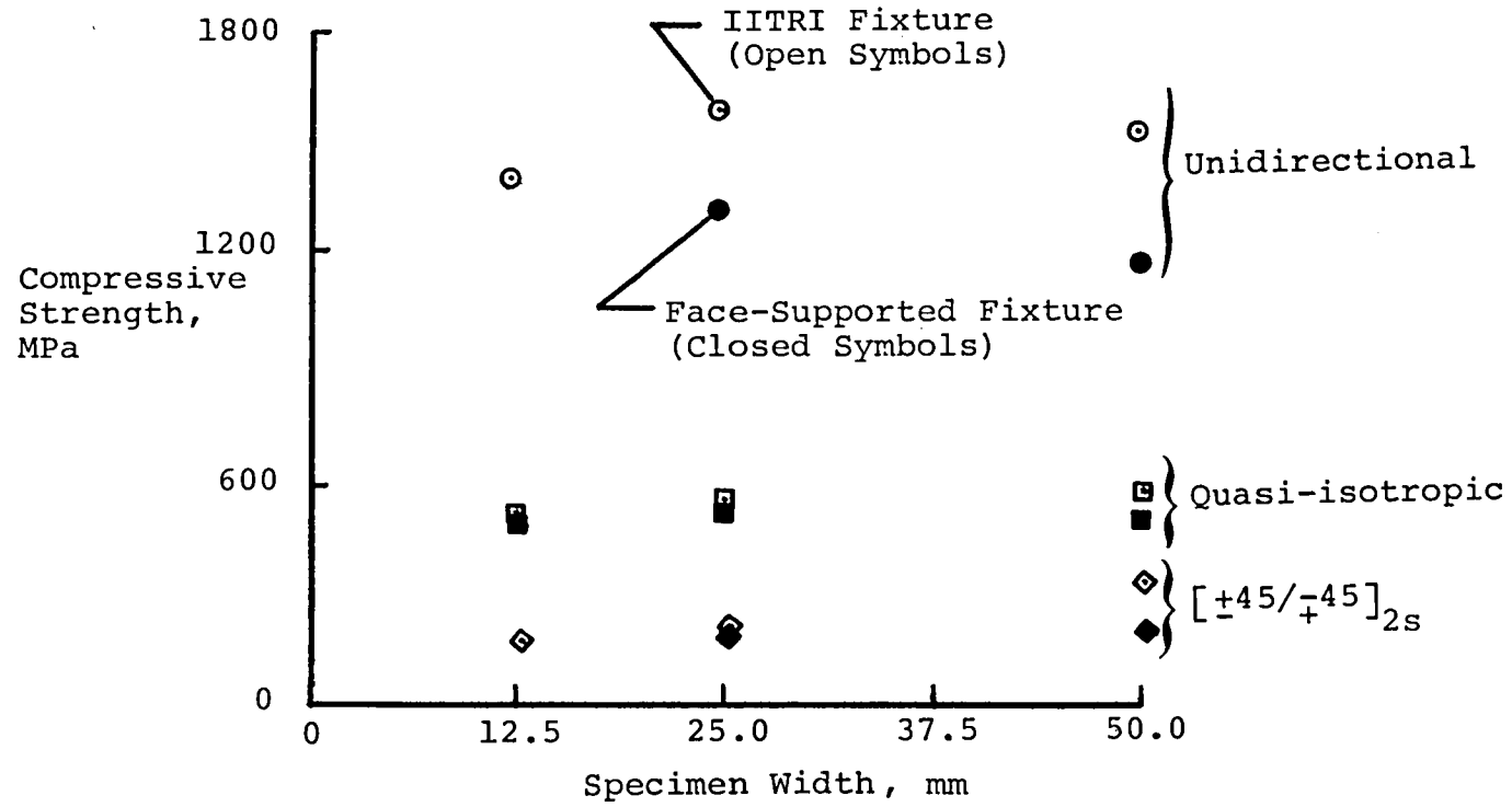
Figure 8.- Average compressive strength of 16-ply Gr/Ep composite material as a function of specimen width.
