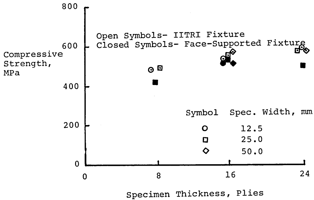
Figure 9.- Average compressive strength of quasi-isotropic Gr/Ep composite material as a function of specimen thickness.
