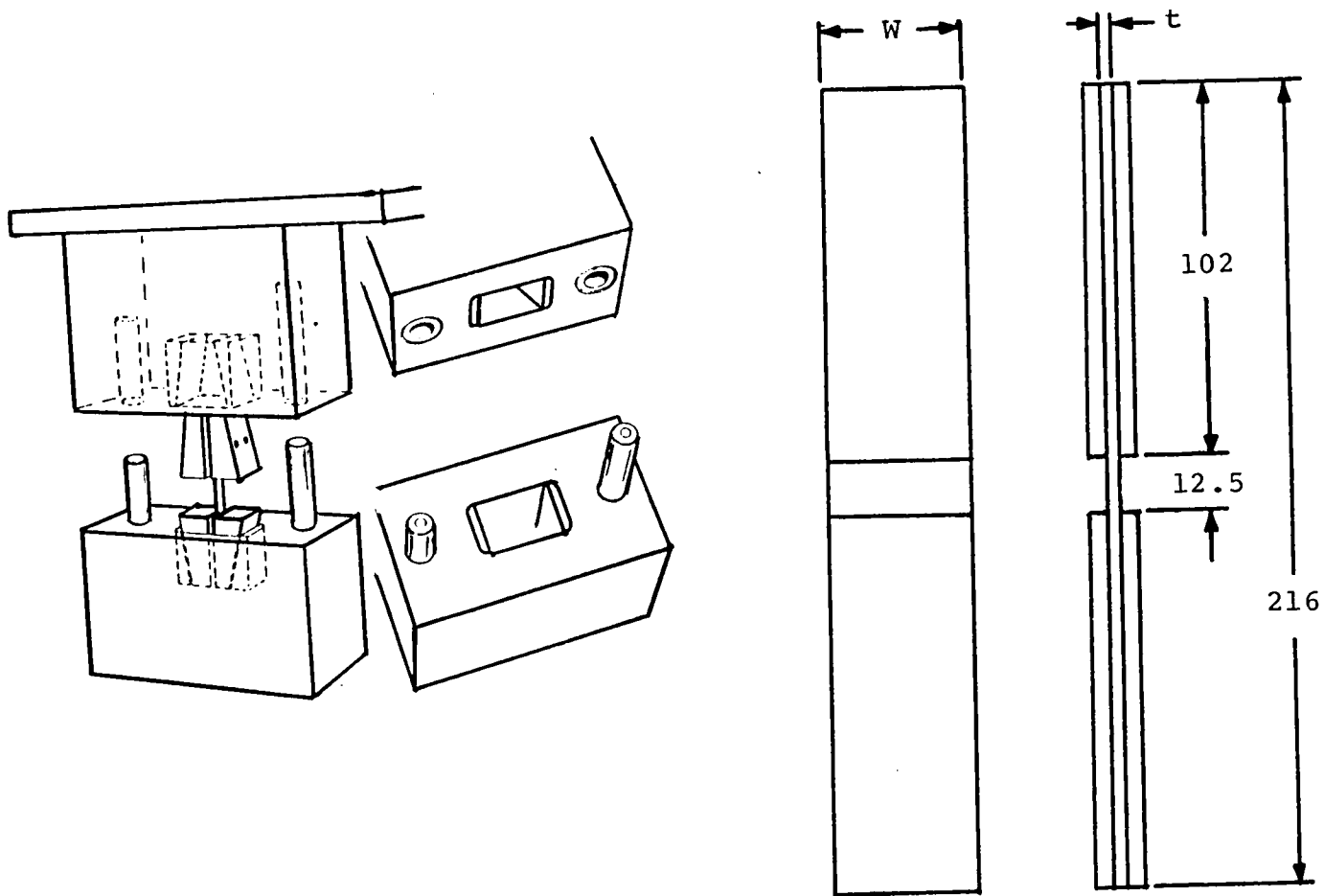
Figure 1.- Schematic of IITRI fixture and sketch of specimen.
