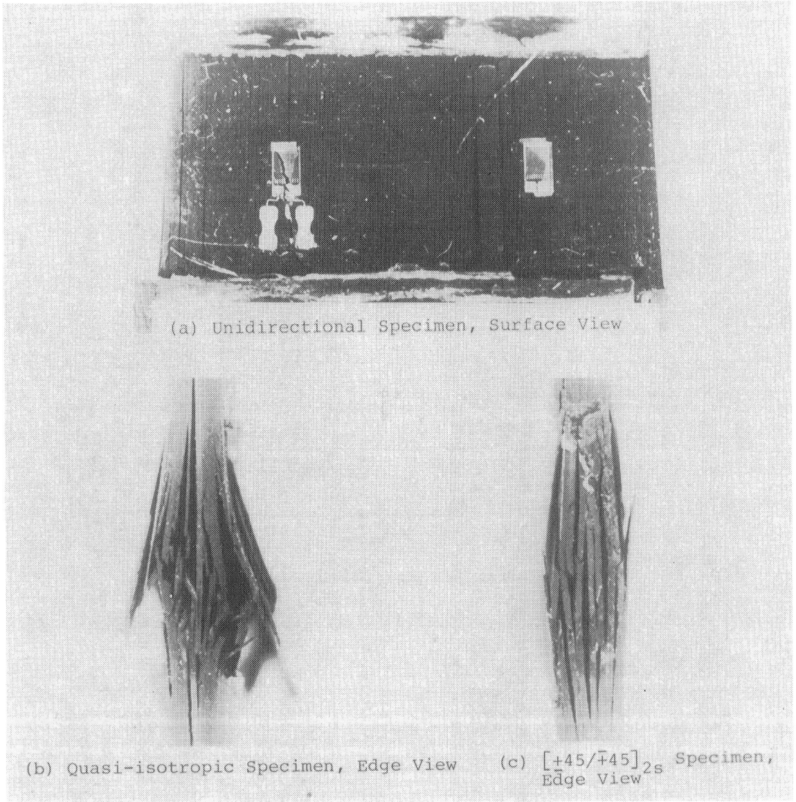
Figure 13.- Photographs of failed 16-ply 25-mm-wide specimens tested in IITRI fixture.
