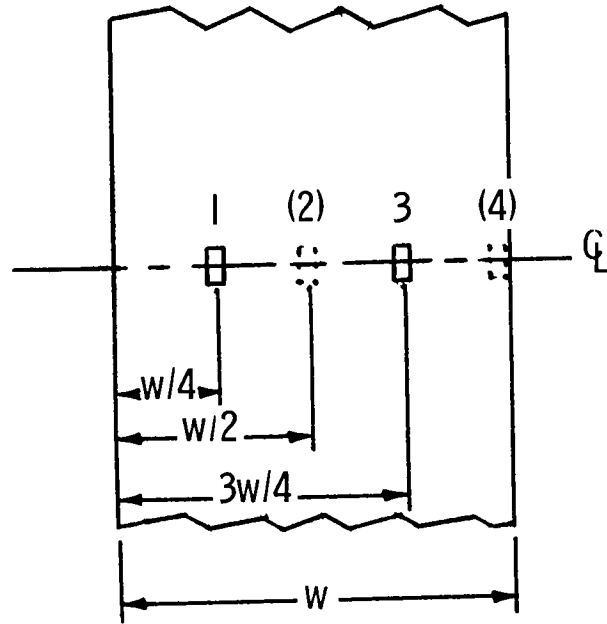
Figure 4.- Location of strain gages on specimen.
