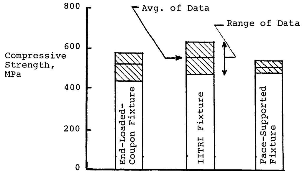
Figure 10.- Compressive strength of 25-mm wide 16-ply quasi-isotropic Gr/Ep specimens tested with the end-loaded, IITRI, and face-supported fixtures.
