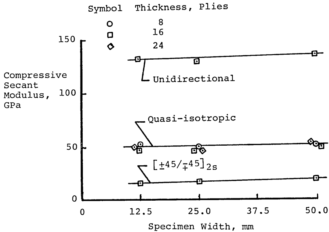
Figure 11(a).- Secant modulus at .004 strain of Gr/Ep composite material as a function of specimen width and thickness for specimens tested with the IITRI fixture.
