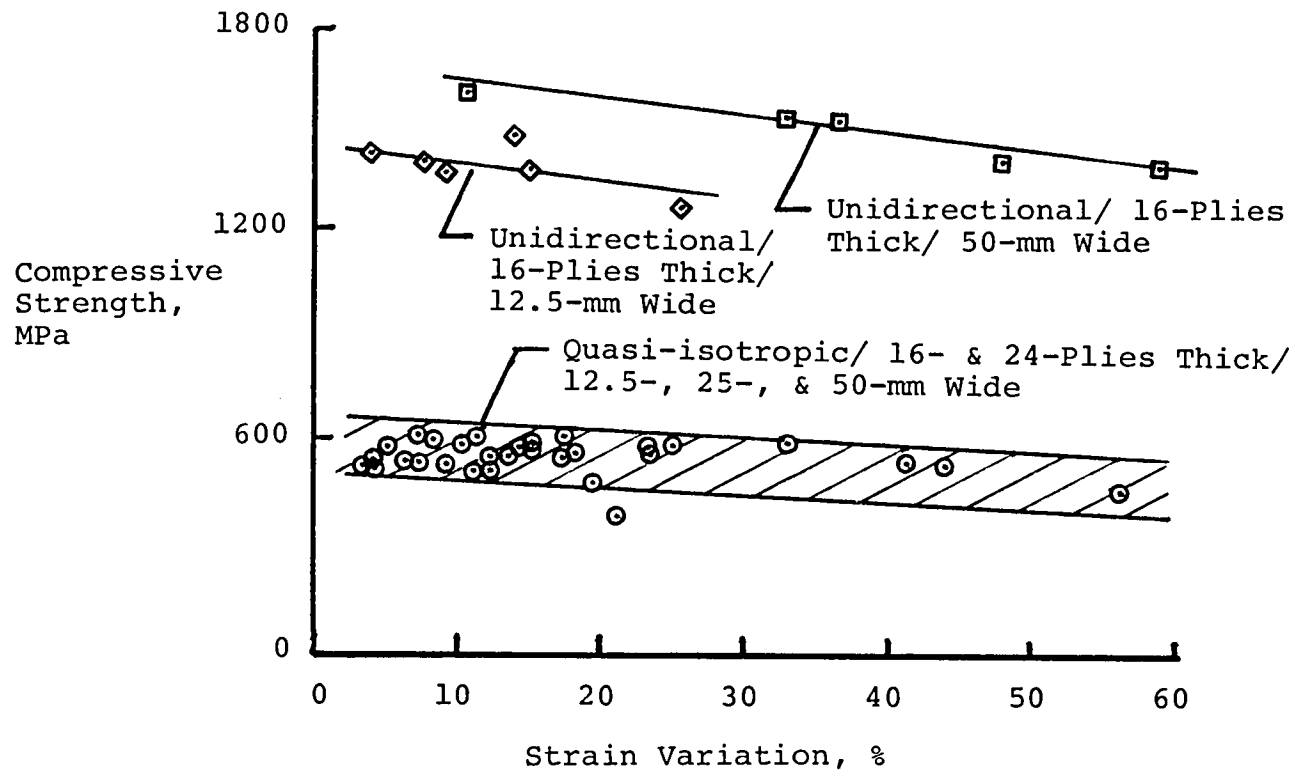
Figure 7.- Effect of strain variation on compressive strength of Gr/Ep specimens tested with the IITRI fixture.
