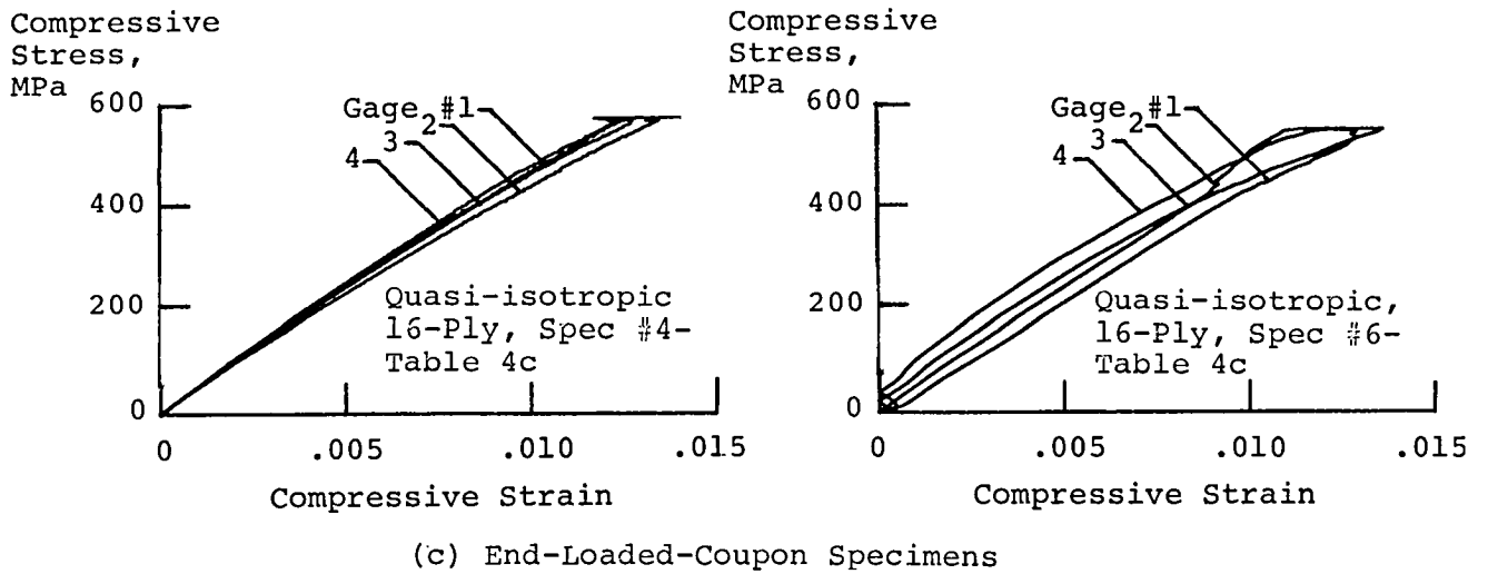
Figure 6.- Representative best and worst compressive stress-strain curves for Gr/Ep composite material specimens.
