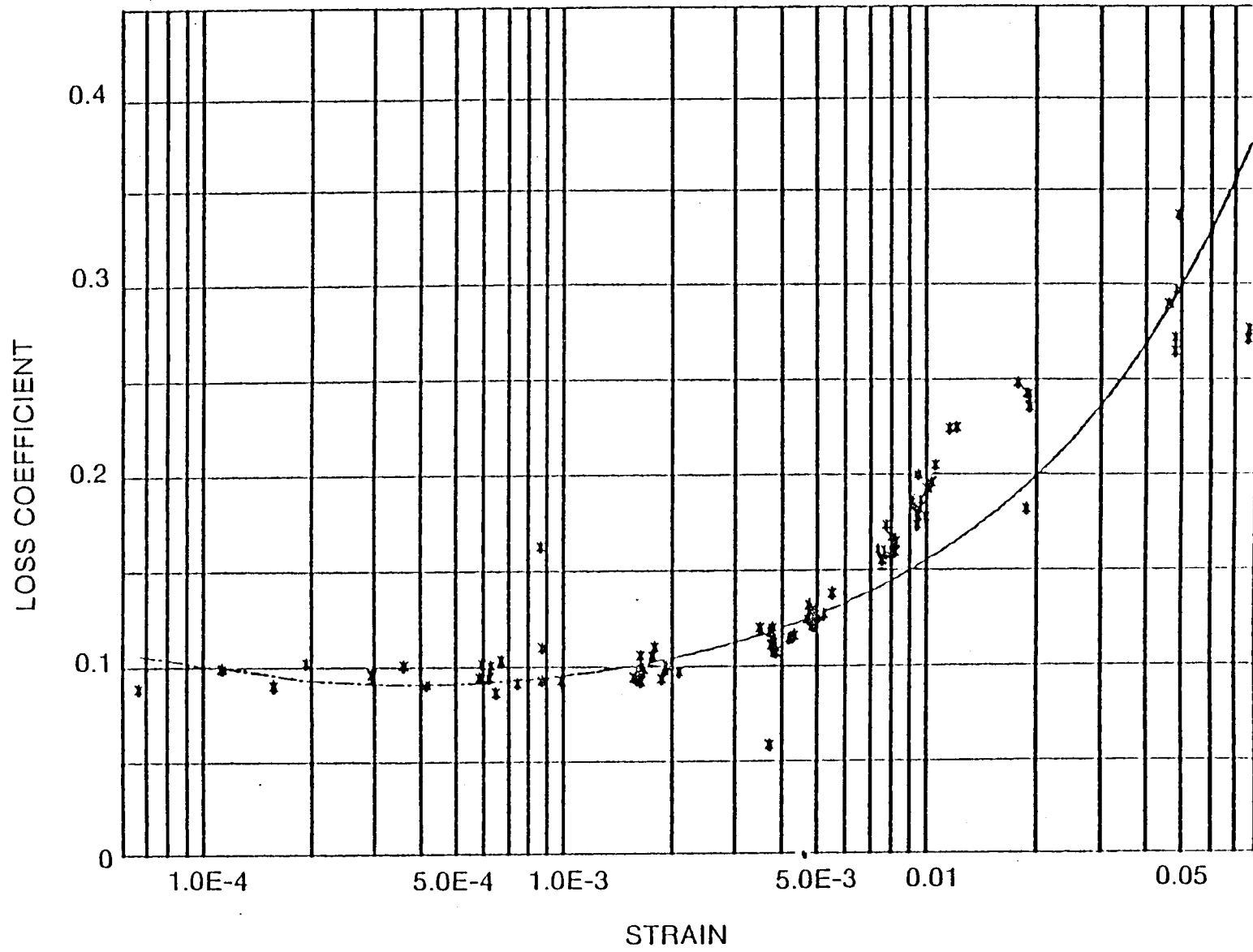
Figure 54 Shear Specimen Data EPDM at 66°C
