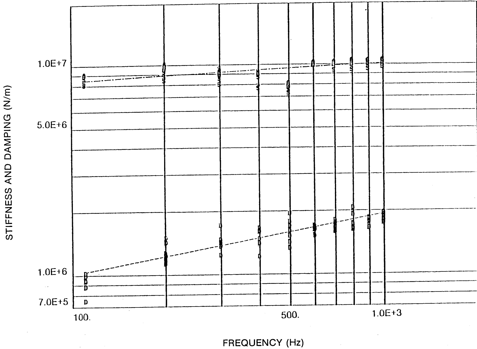
Figure 79 Shear Specimen Data Viton-70 at 80°C
