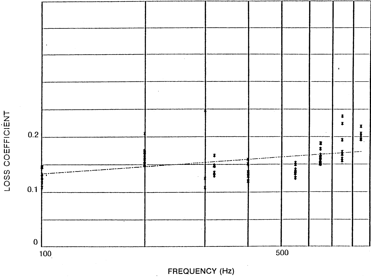
Figure 64 Shear Specimen Data Buna-N at 66°C
