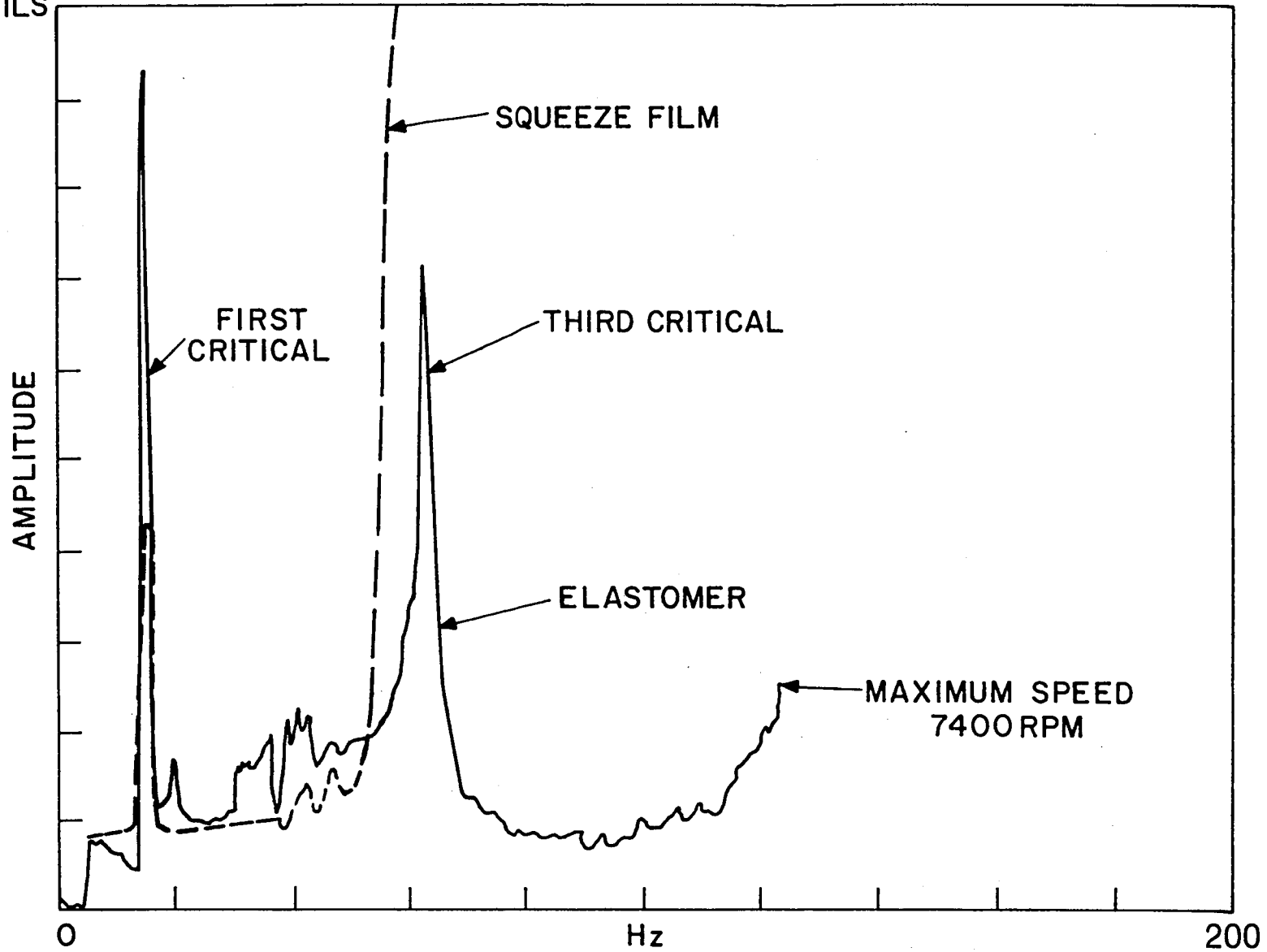
Figure 28 Synchronous Response Comparison, Probe #3
