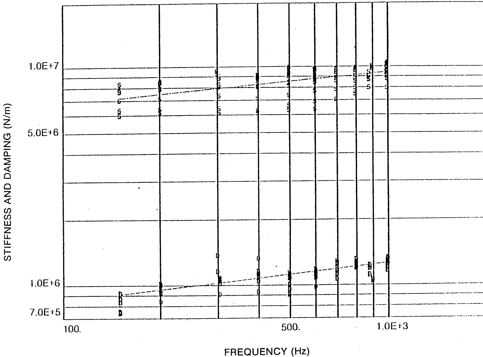
Figure 91 Shear Specimen Data Neoprene at 80°C
