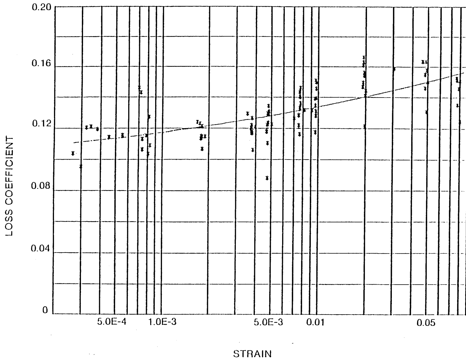
Figure 94 Shear Specimen Data Neoprene at 80°C
