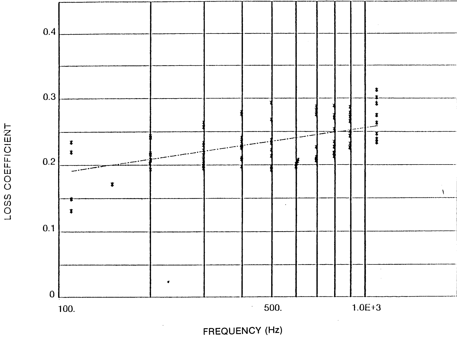
Figure 84 Shear Specimen Data Neoprene at 32°C
