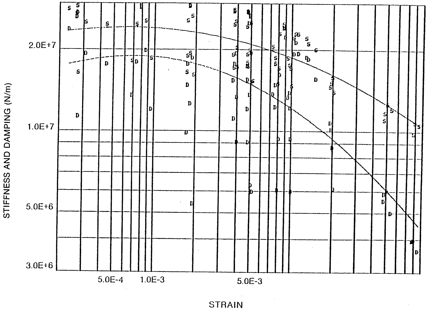
Figure 73 Shear Specimen Data Viton-70 at 32°C
