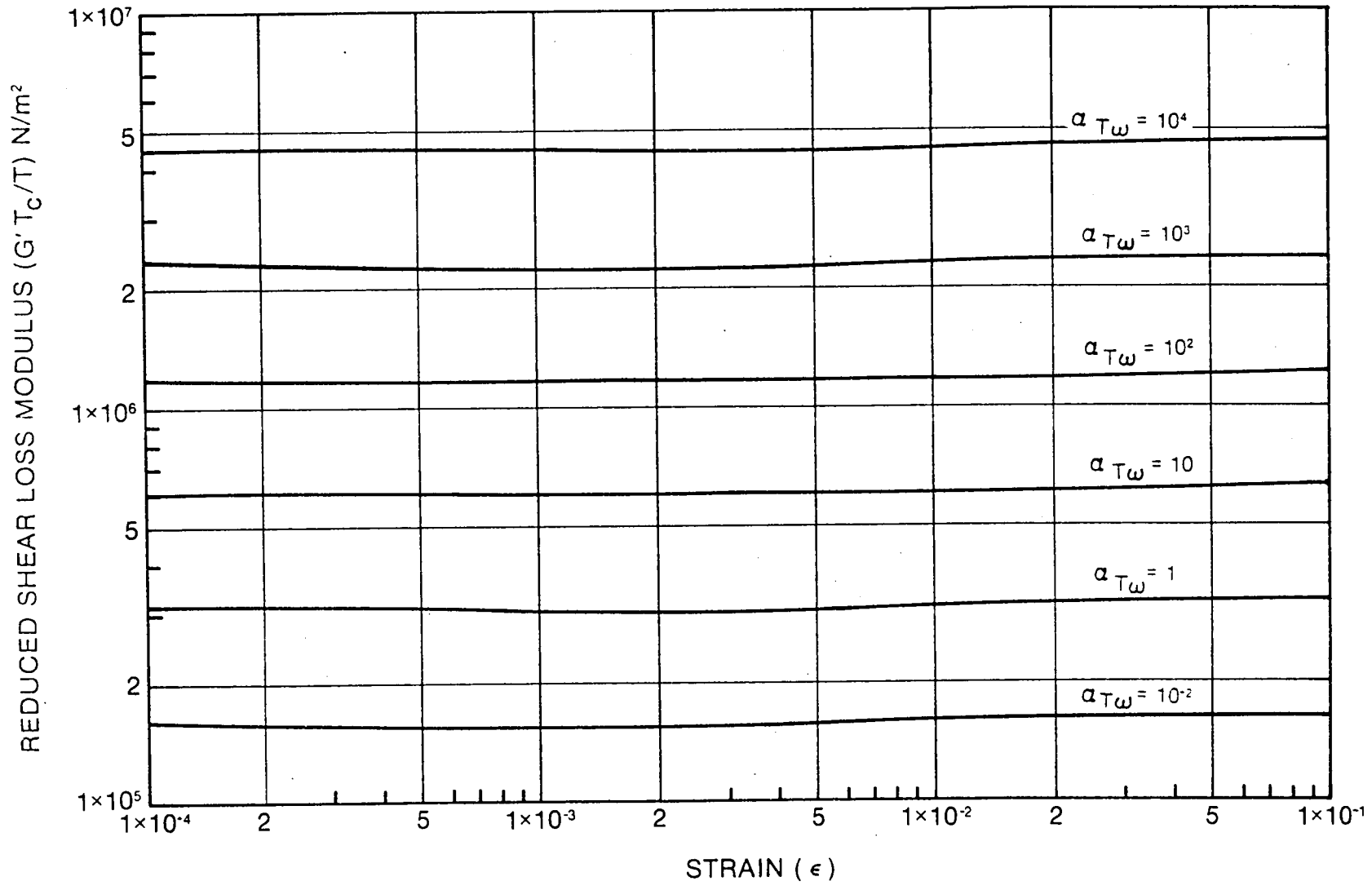
Figure 107 Buna-N Design Curves
