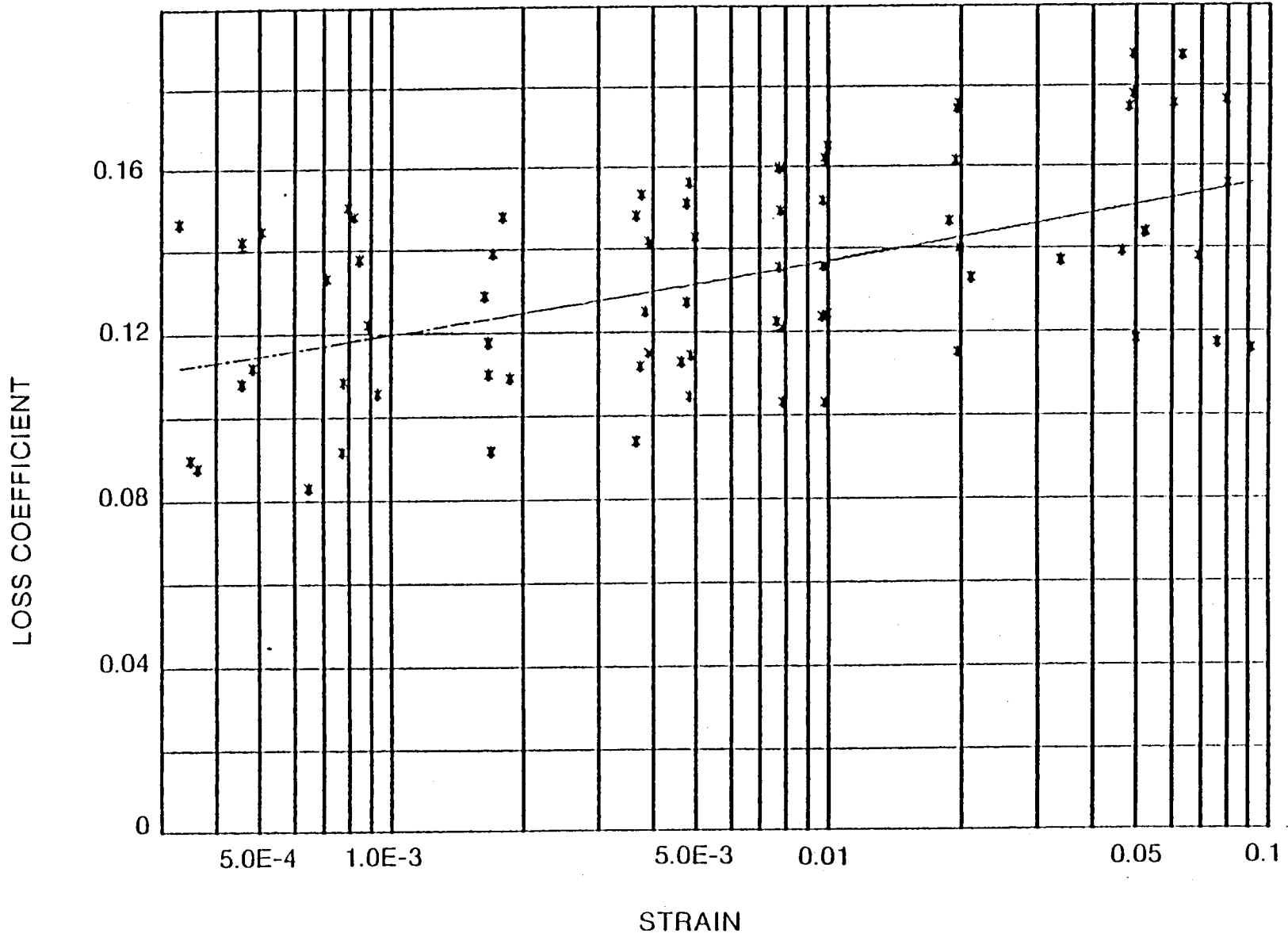
Figure 70 Shear Specimen Data Buna-N at 80°C
