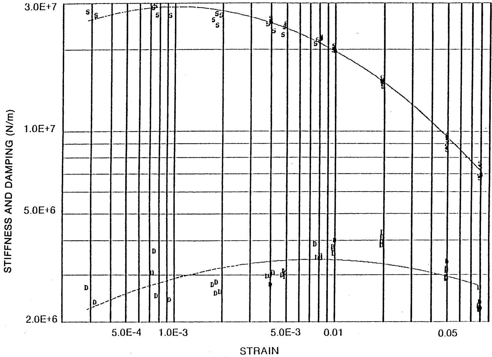
Figure 50 Shear Specimen Data EPDM at 32°C
