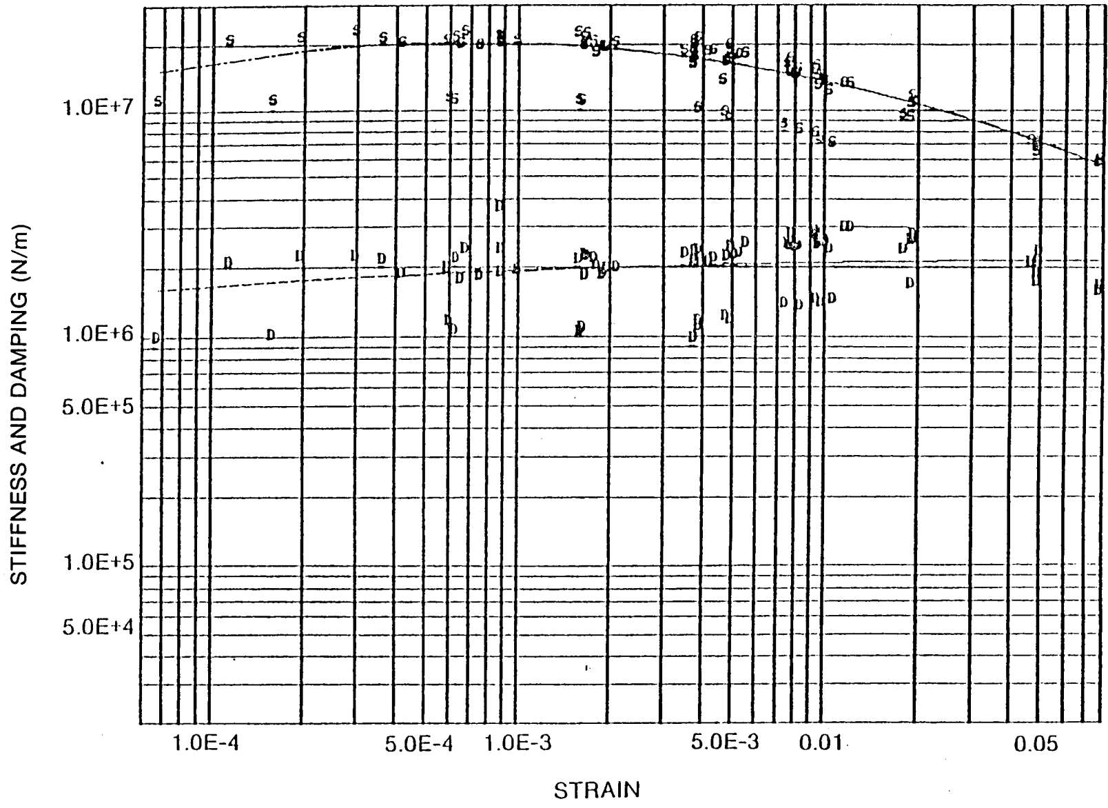
Figure 52 Shear Specimen Data EPDM at 66°C
