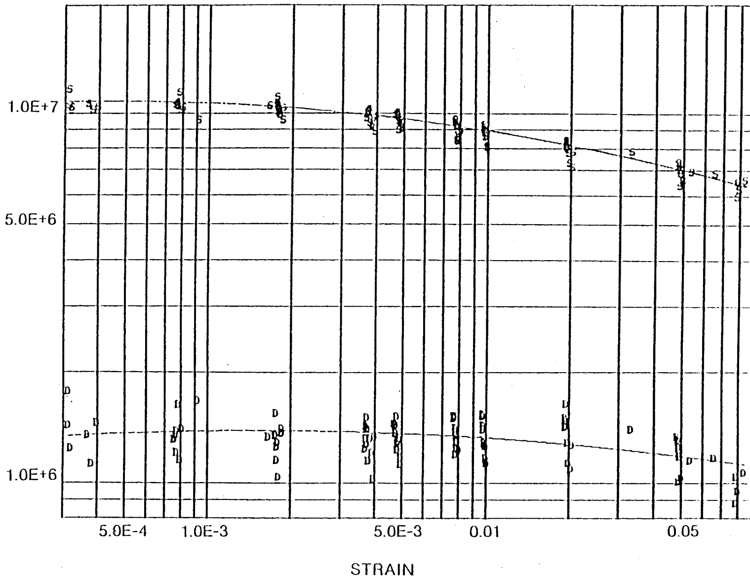
Figure 89 Shear Specimen Data Neoprene at 66°C
