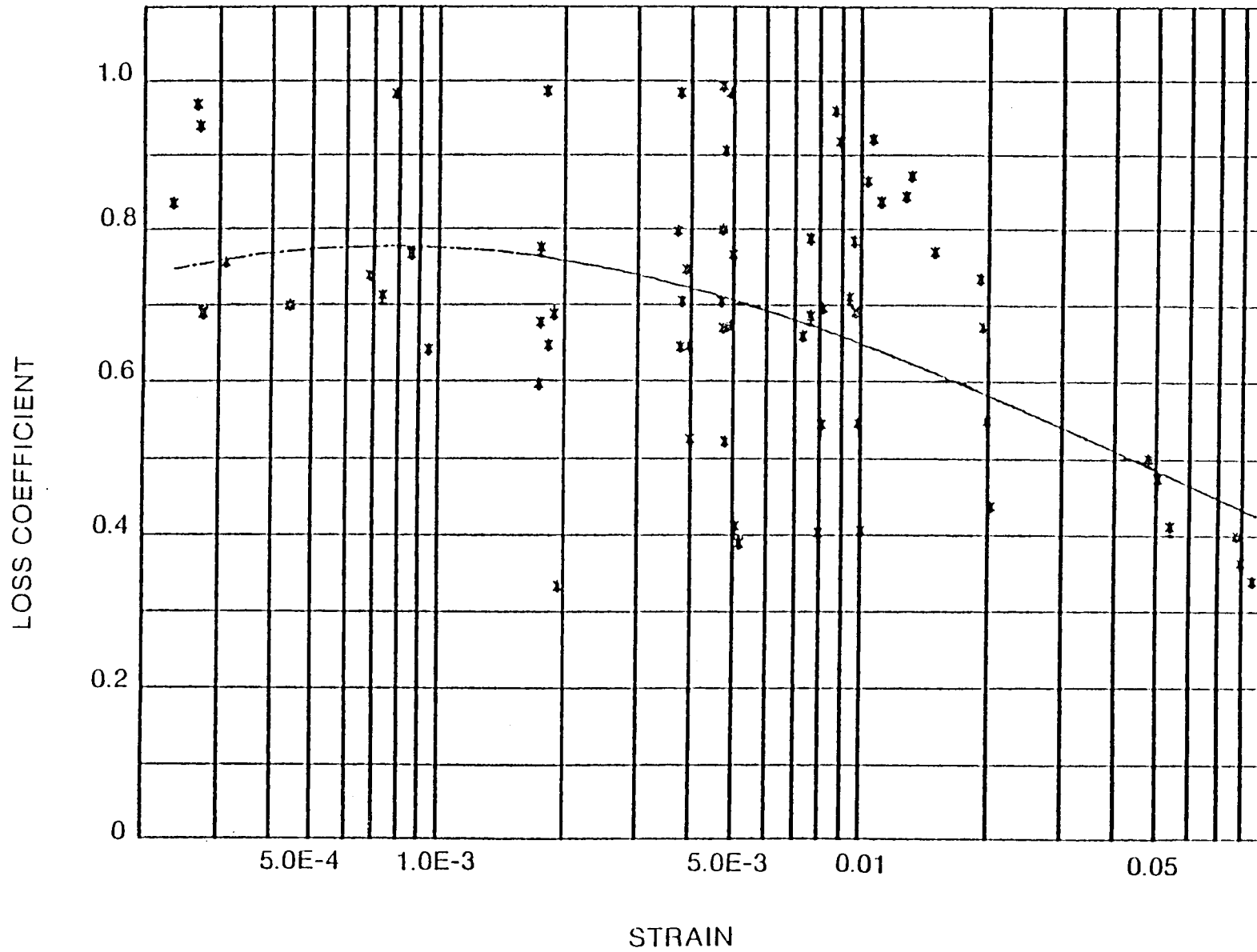
Figure 74 Shear Specimen Data Viton-70 at 32°C
