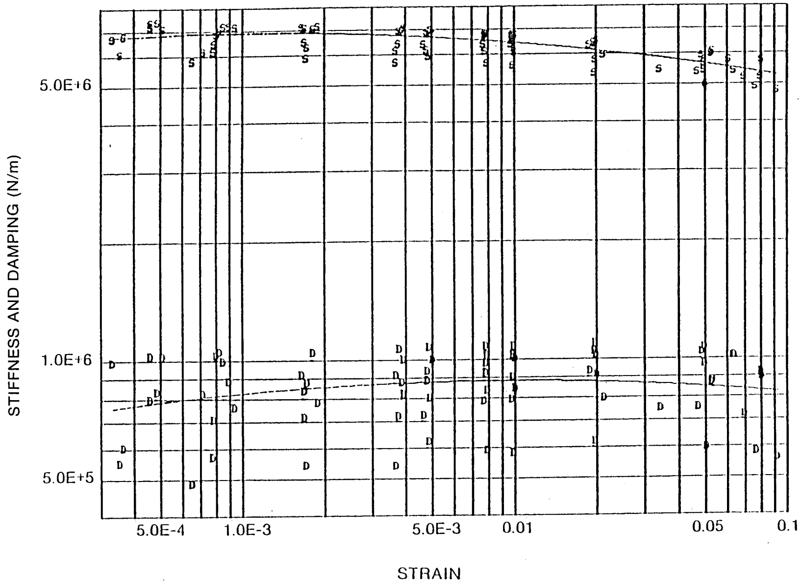
Figure 69 Shear Specimen Data Buna-N at 80°C
