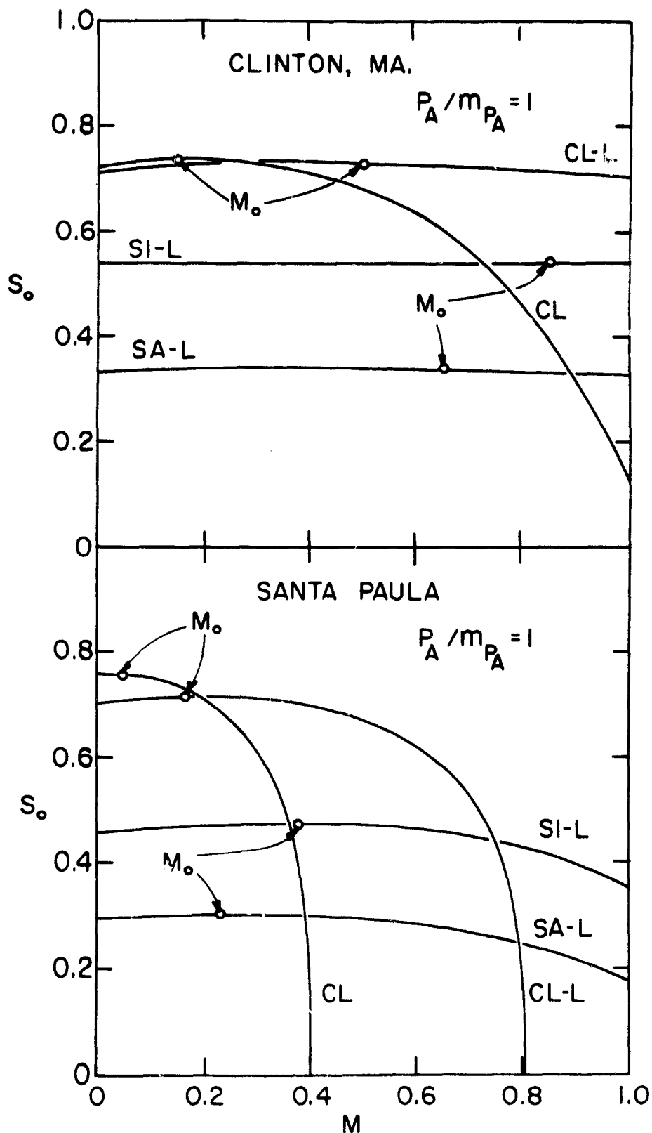
SENSITIVITY OF MEAN ANNUAL SOIL MOISTURE TO VEGETAL CANOPY DENSITY FOR TYPICAL SOILS ( k_v = 1 AND w/\bar{e}_p \ll 1 )
