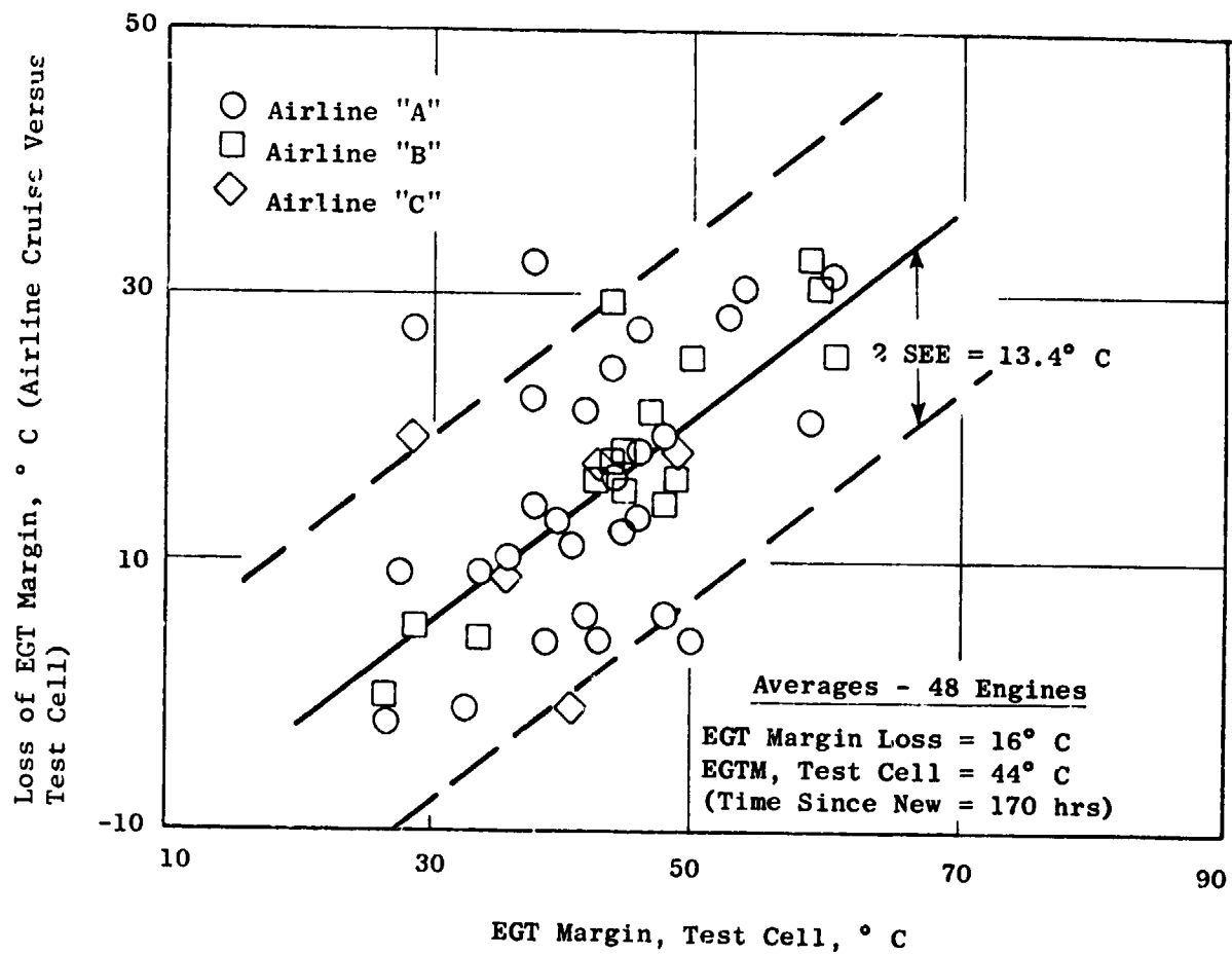
Figure 4-4. Early Revenue Service EGT Cruise Losses.
