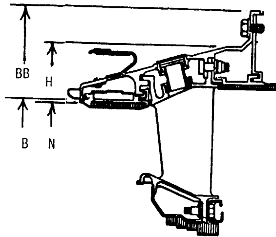
Figure B-18. Stage 2 Nozzle Support - Locations of Dimensional Inspections.
