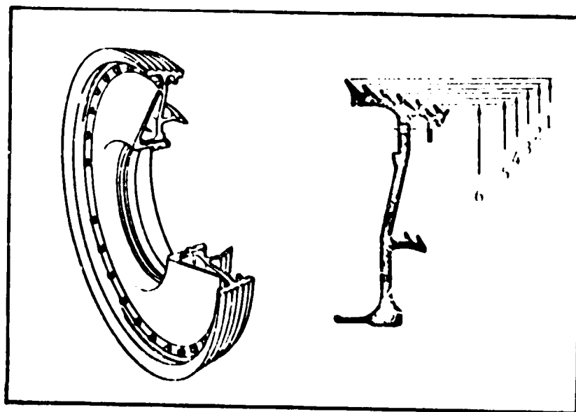
Figure B-5. Forward CDP Seal, Rotating.
