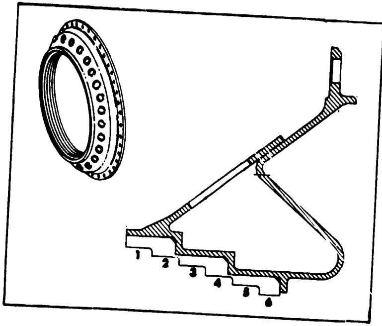
Figure B-8. Forward CDP Seal, Stationary.
