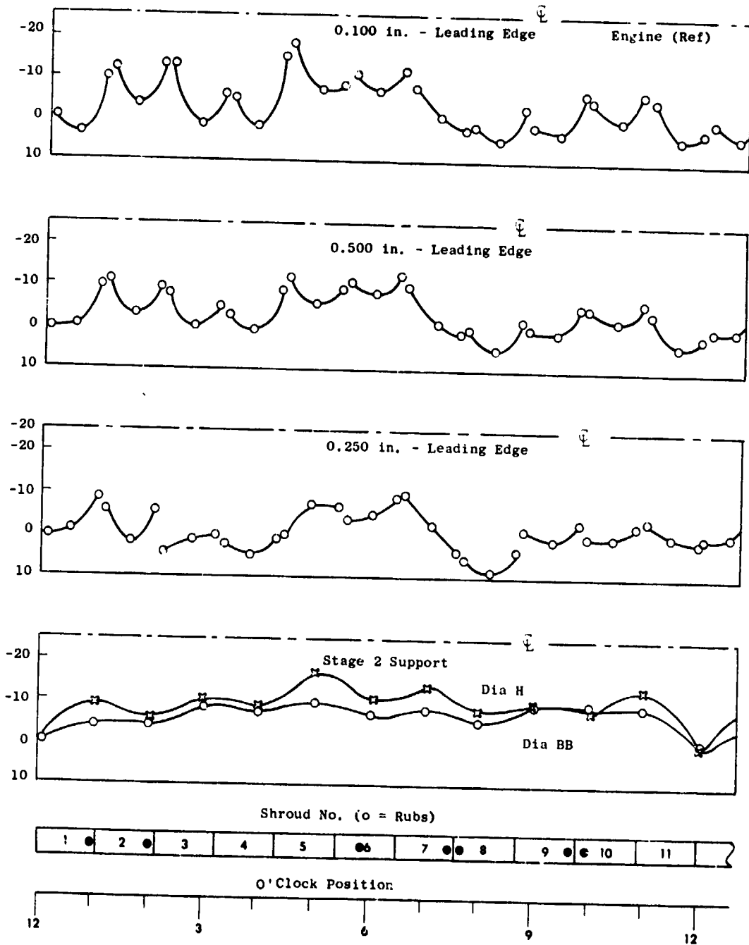
Figure B-19. Stage 2 HPTN Support and Stage 2 Shroud Runouts.
