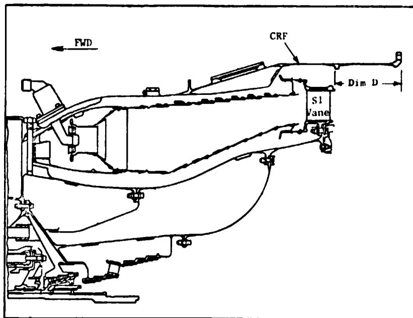
Figure B-12. Dimension "D" - Drop from CRF to Stage 1 HPTN Vane.
