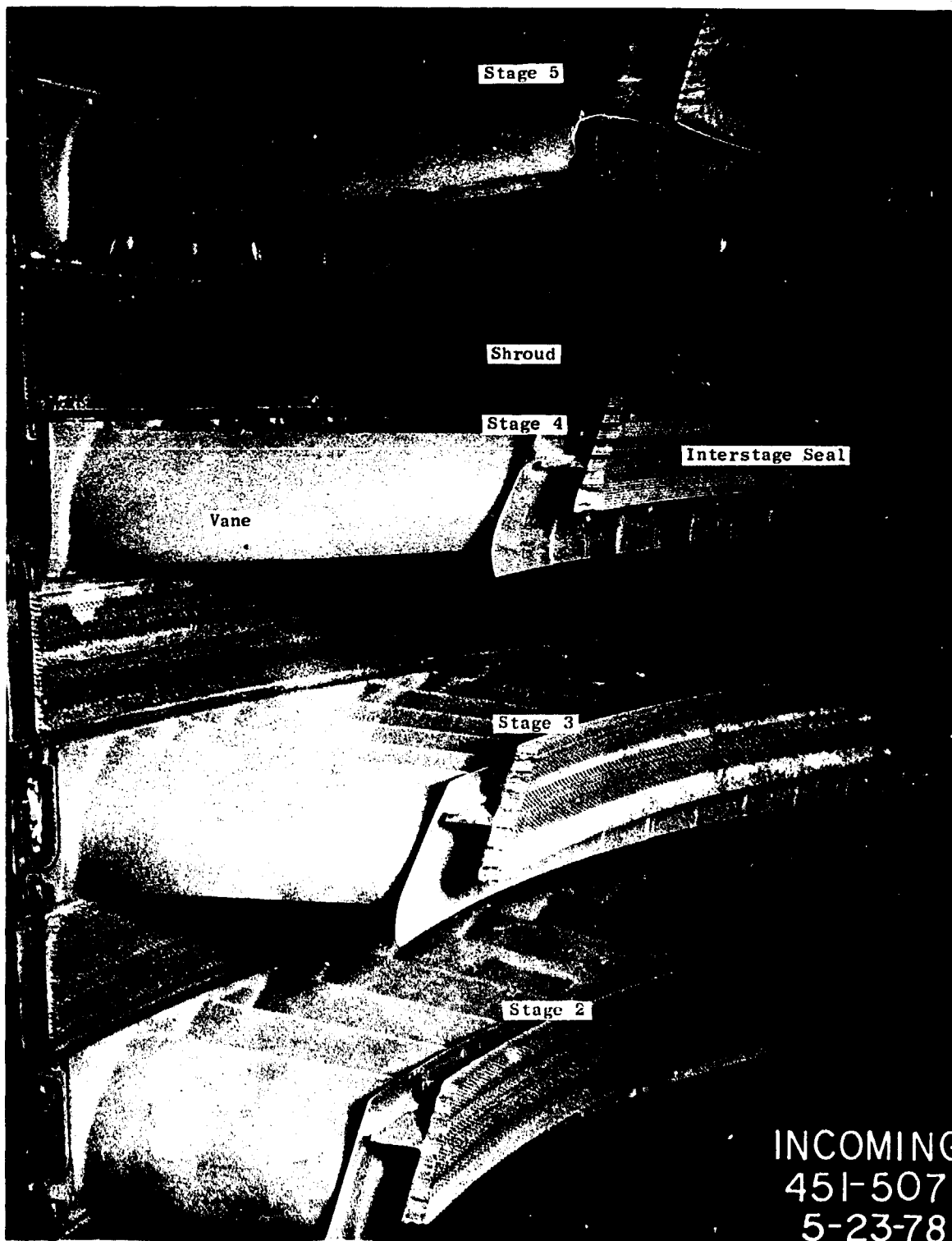
Figure B-32. Low Pressure Turbine Stator Assembly - View of Shroud and Seal Rubs.
