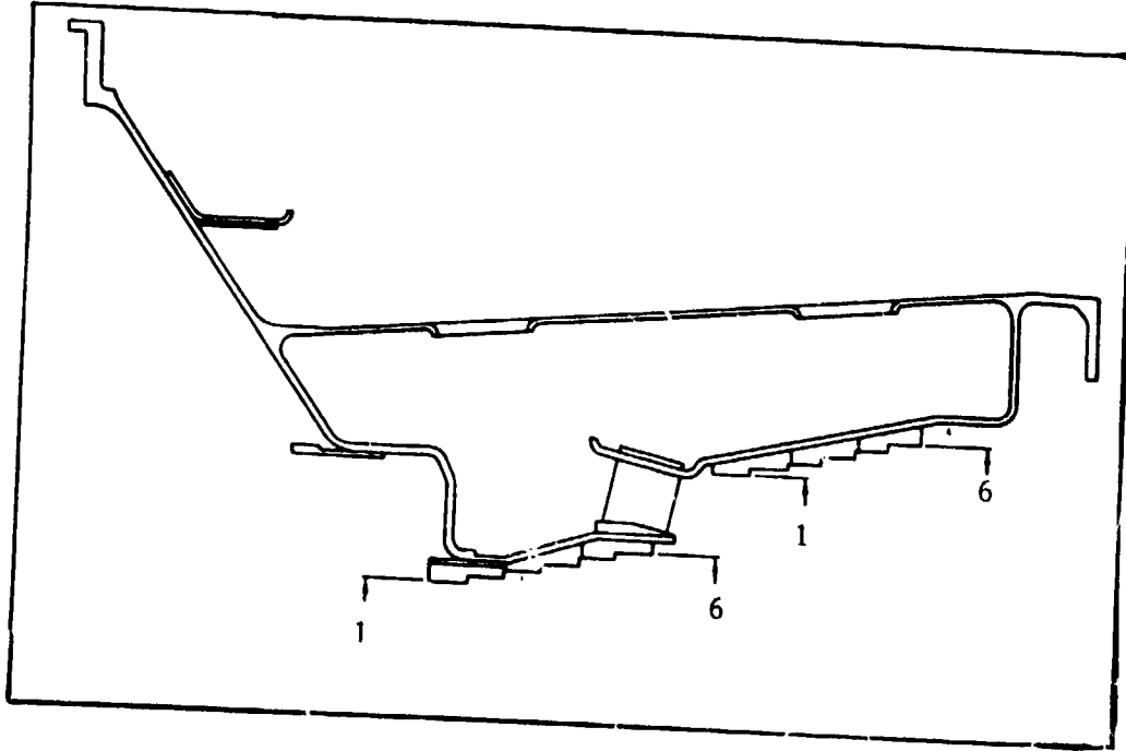
Figure B-9. No. 4B Pressure Balance Seal (Mini-Nozzle).
