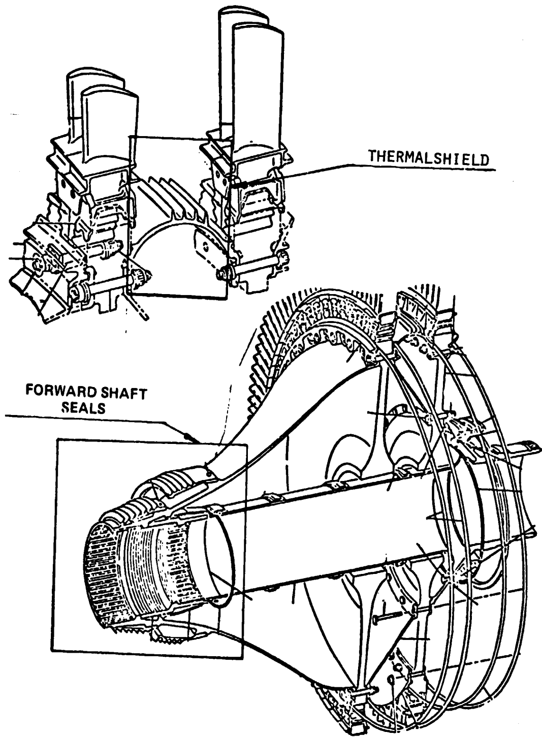
Figure B-27. HP Turbine Rotor Forward Shaft Seals and Thermal Shield.
