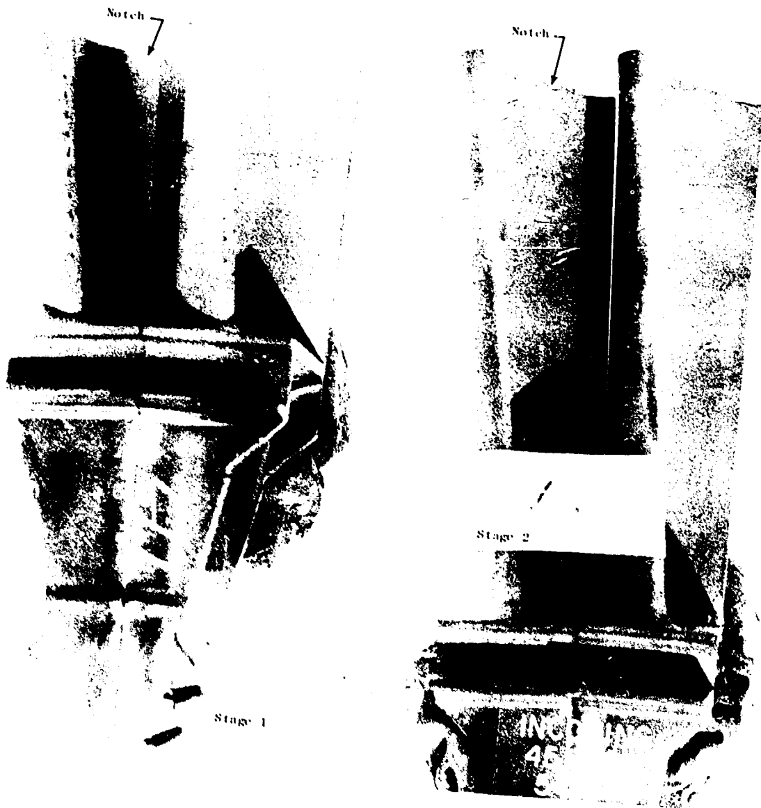
Figure B-24. High Pressure Turbine Notched Blades at Teardown.
