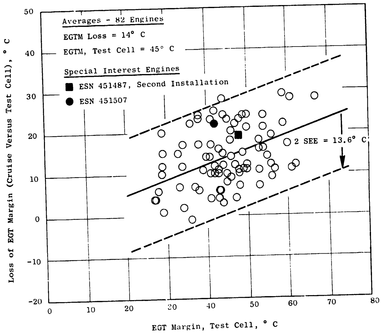
Figure 4-2. Short-Term EGTM Cruise Losses - First Checkout Flight.
