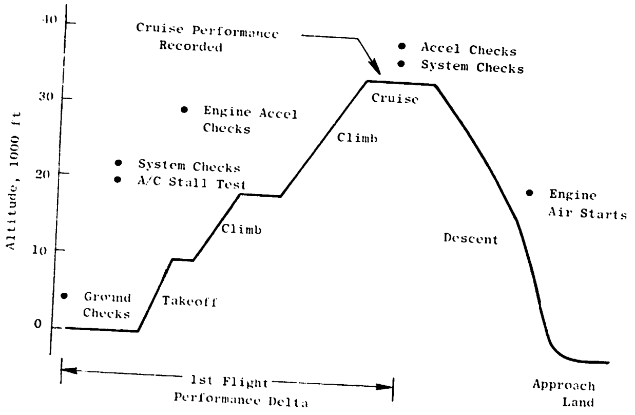
Figure 3-13. Schematic of DC-10-10 Initial Acceptance Test Flight.
