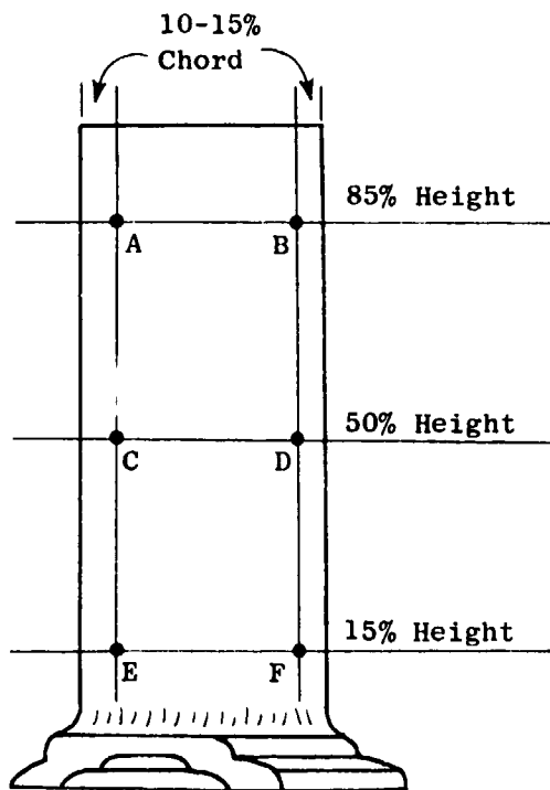
Typical Concave/Convex
