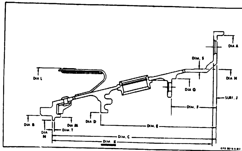
Figure B-16. Dim. "K" - Stage 2 HP Turbine Nozzle Support Measurement.
