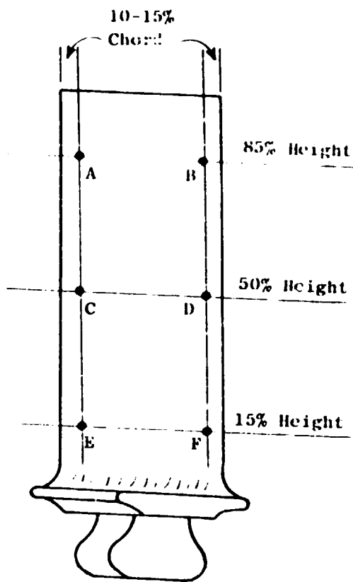
Figure B-4. Location of Surface Finish Measurements - HP Compressor Rotor Blade.
