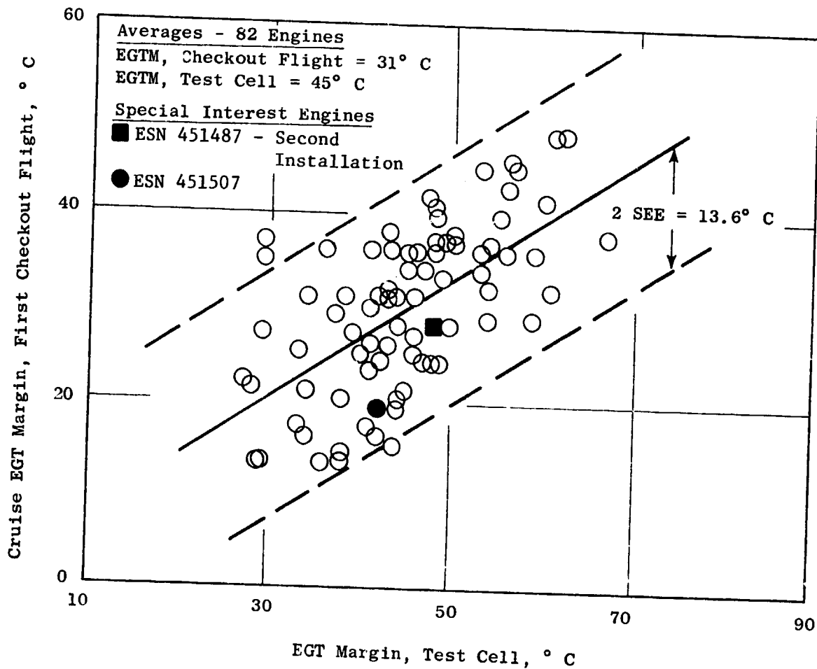
Figure 4-1. EGT Cruise Margin, - First Airplane/Engine Checkout Flight.
