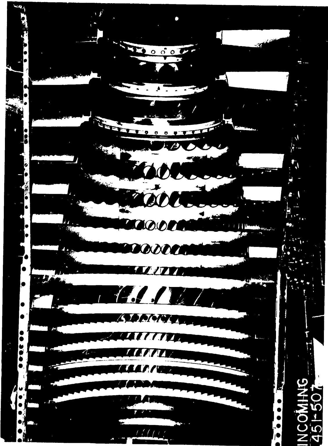
Figure B-6. High Pressure Compressor Stator Assembly - Rubs and Chipped Coating.
