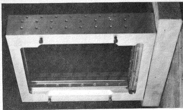
Fig. 1b Large Test Panel Support Fixture
