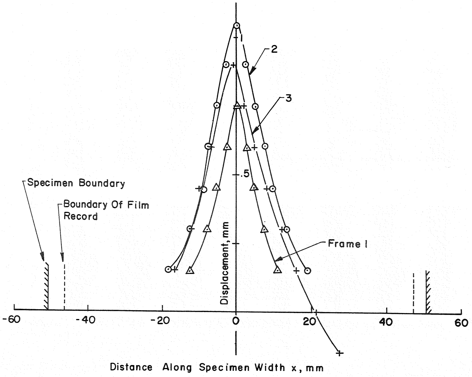
FIG. 17 TEST PANEL B-9 OUT OF PLANE DISPLACEMENT ALONG SPECIMEN WIDTH (time interval between frames - 50.25 \mu s)
