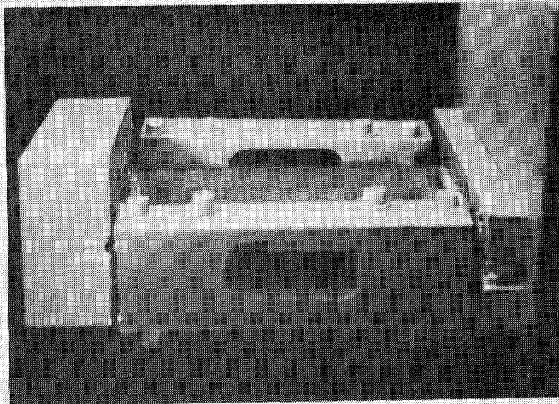
Fig. 1c Partially Free Sided Test Panel Support Fixture
