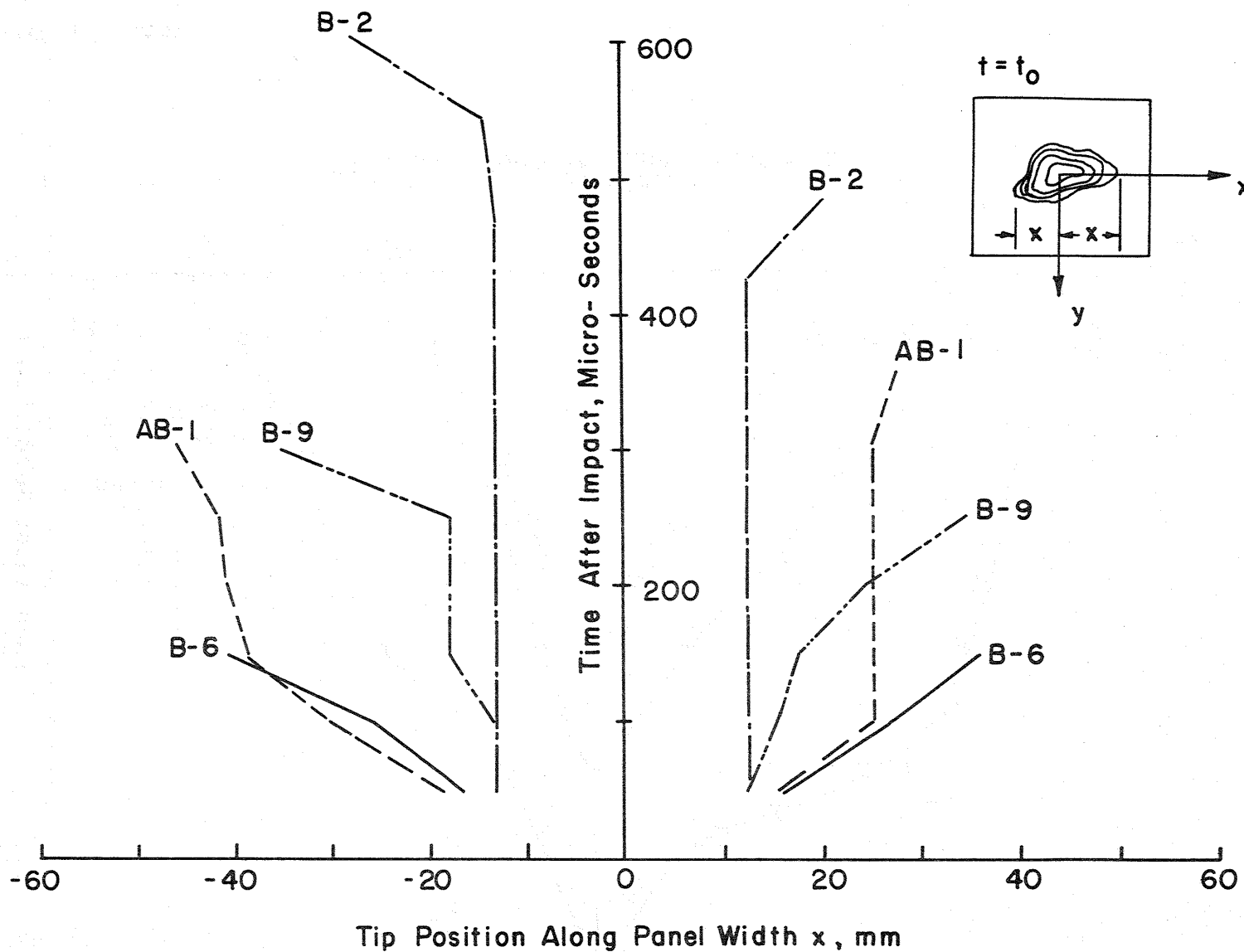
FIG.18 DELAMINATION TIP POSITION ALONG PANEL WIDTH AS FUNCTION OF TIME
