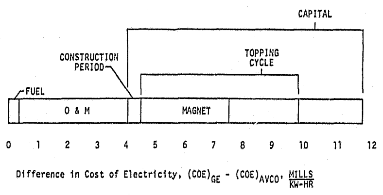
Figure 2. - Difference in Cost of Electricity between G.E. Case 3.4 and Avco Case III-1.
