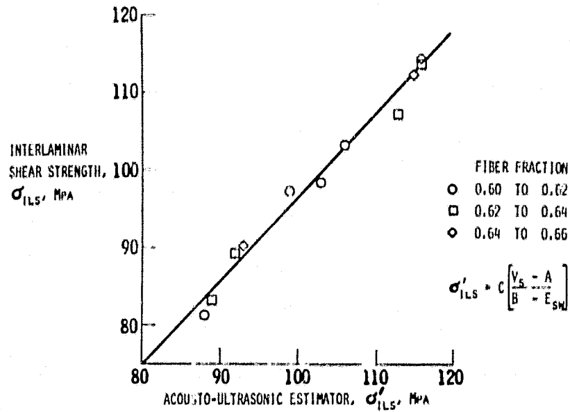
Fig. 11. Correlation of graphite/polyimide fiber composite interlaminar shear strength with acousto-ultrasonic estimator. The estimator is derived from stress wave factor and velocity measurements, E_{SW} and V_S , respectively. A, B, and C are experimental constants (Vary and Bowles, 1977).
