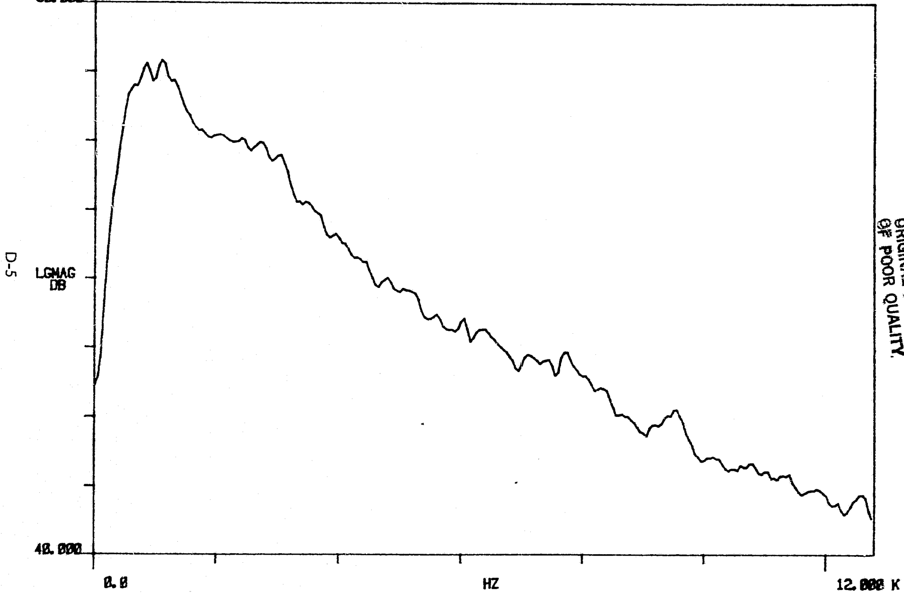
Fig. 3D - A-Weighted Source Contribution Analysis : Gizzard Machine CENTRAL SOYA PLANT (pt. 6B, ch.2)
