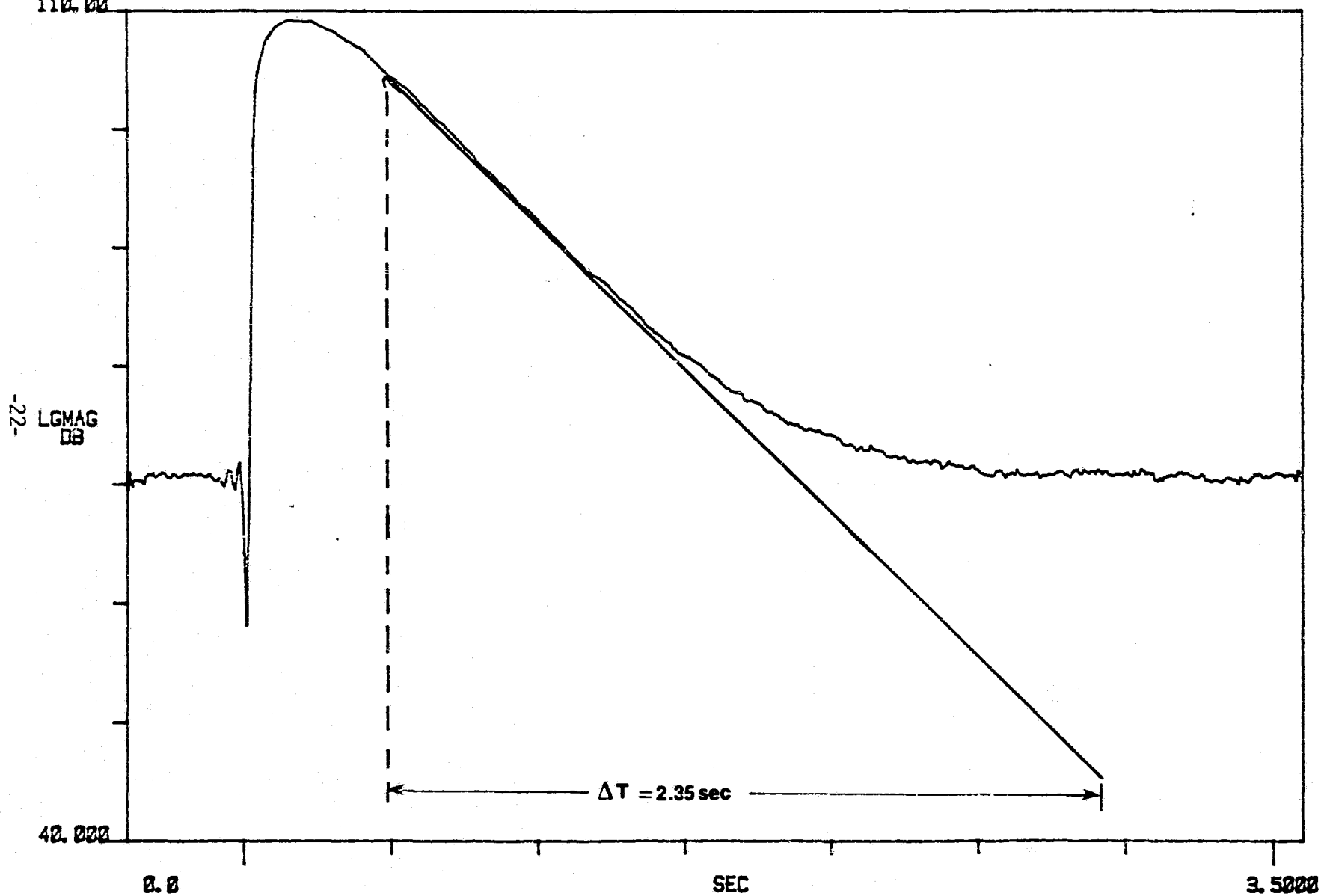
Fig. 12 Time History of Reverberant Noise Field Decay TIP TOP PLANT
