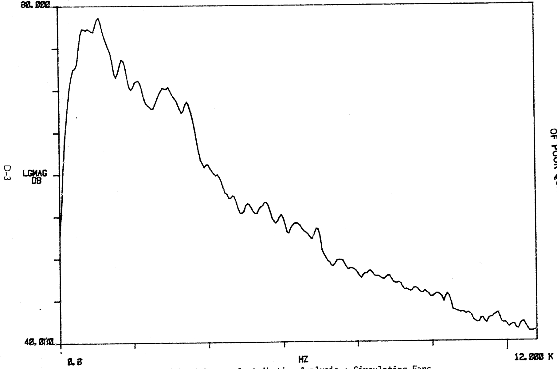
Fig. 1D - A-Weighted Source Contribution Analysis : Circulating Fans CENTRAL SOYA PLANT (pt. 6B, ch.2)
