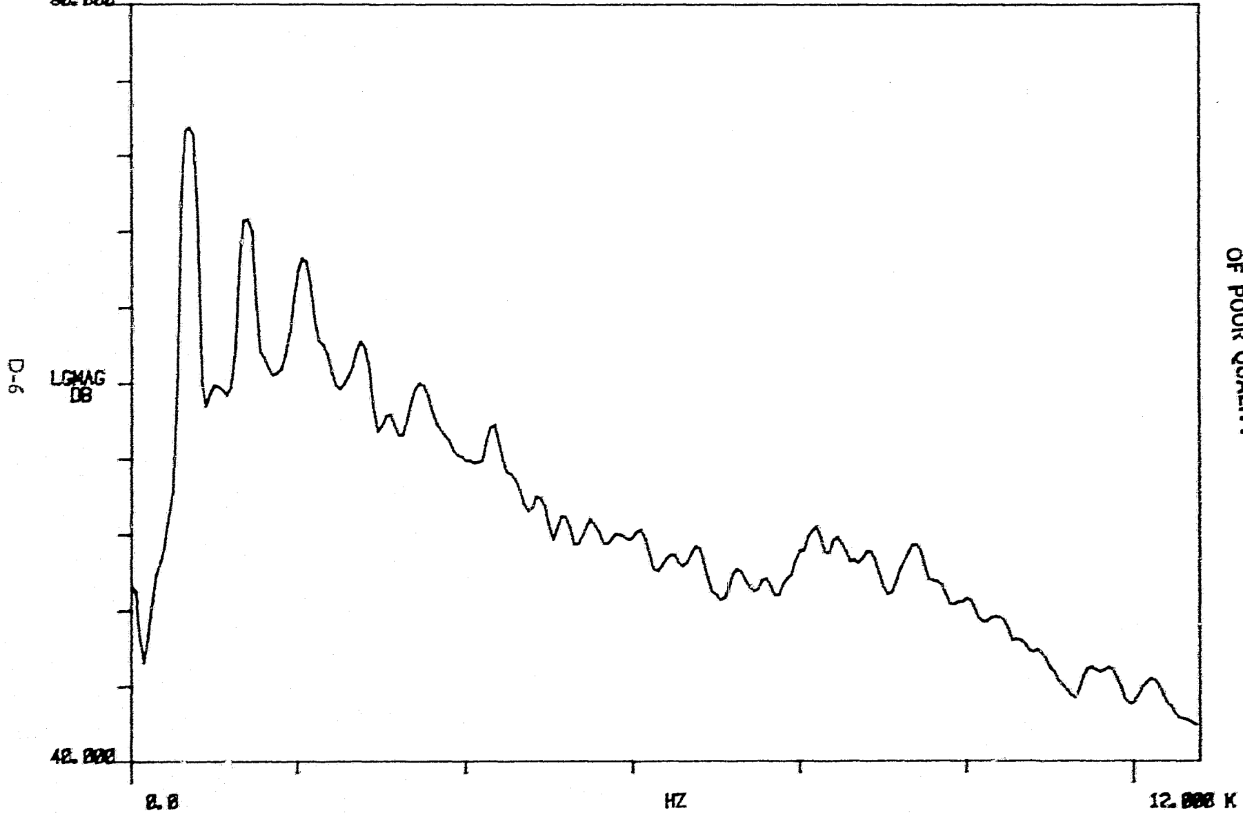
Fig. 4D - A-Weighted Source Contribution Analysis : Spray Washer CENTRAL SOYA PLANT (pt. 6B, ch.2)
