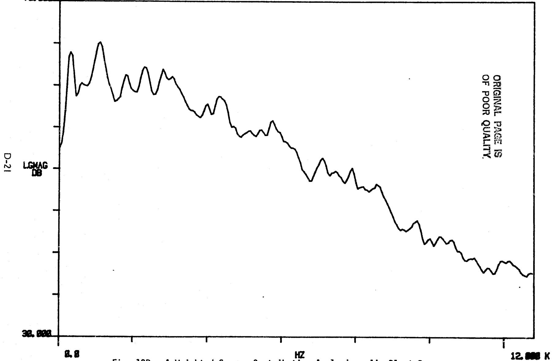
Fig. 19D - A-Weighted Source Contribution Analysis : Air Blast Dryer TIP TOP PLANT (pt. 53, ch.2)
