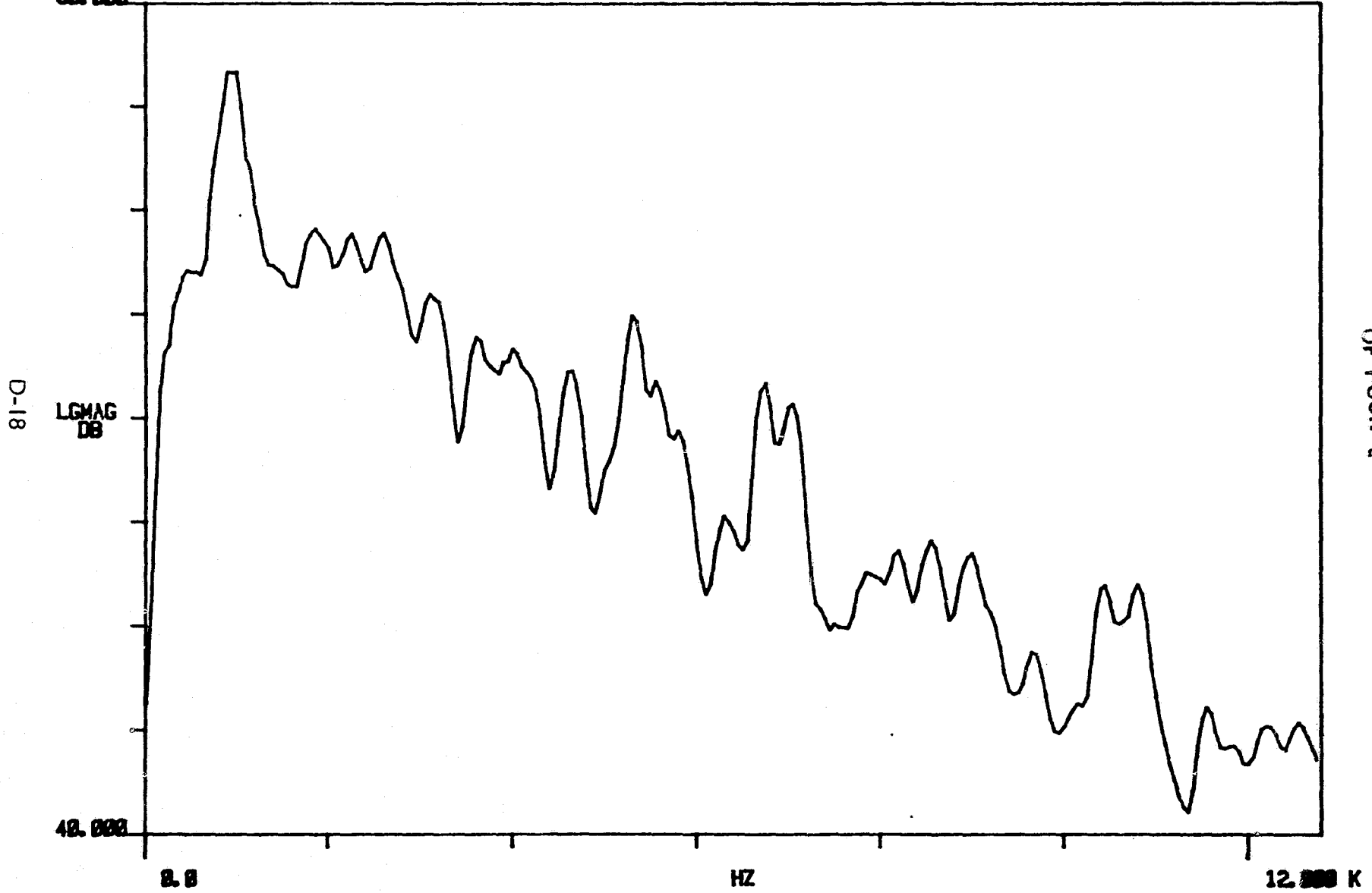
Fig. 16D - A-Weighted Source Contribution Analysis : Gizzard Machine TIP TOP PLANT (pt. 53, ch.2)
