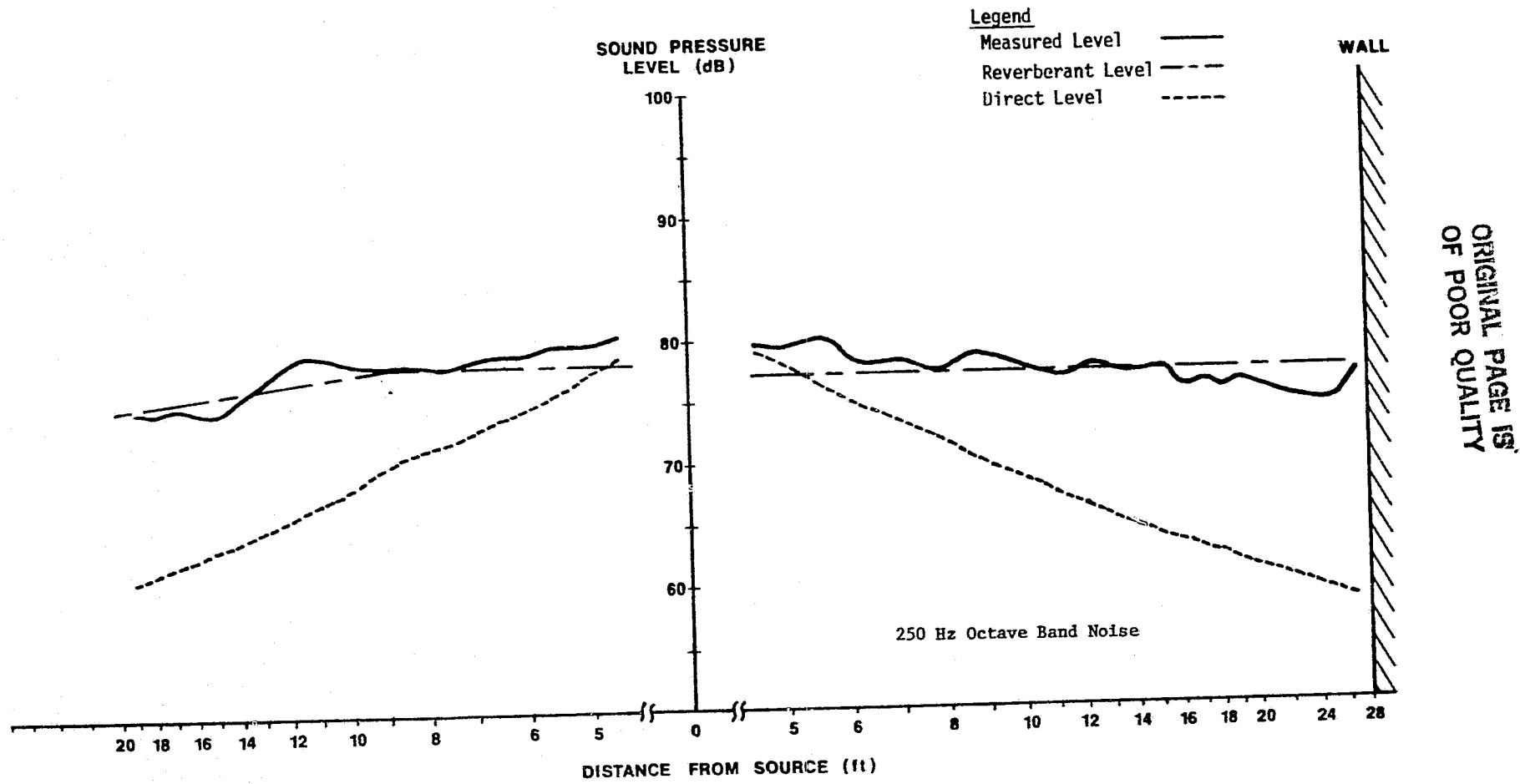
Fig. 6C Direct/Reverberant Noise Fields for Test Speaker CENTRAL SOYA PLANT
