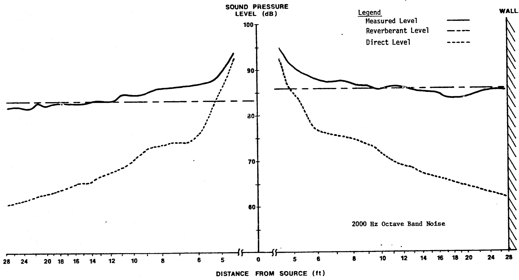
Fig. 4C Direct/Reverberant Noise Fields for Test Speaker TIP TOP PLANT
