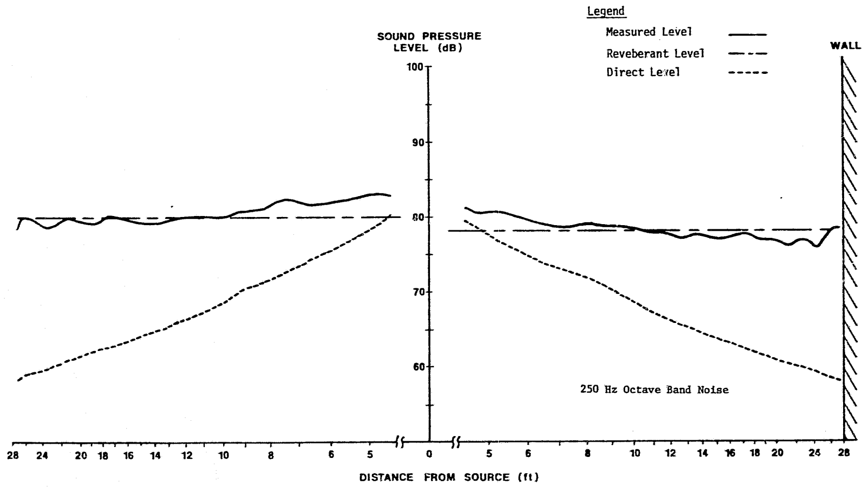
Fig. 1C Direct/Reverberant Noise Fields for Test Speaker TIP TOP PLANT
