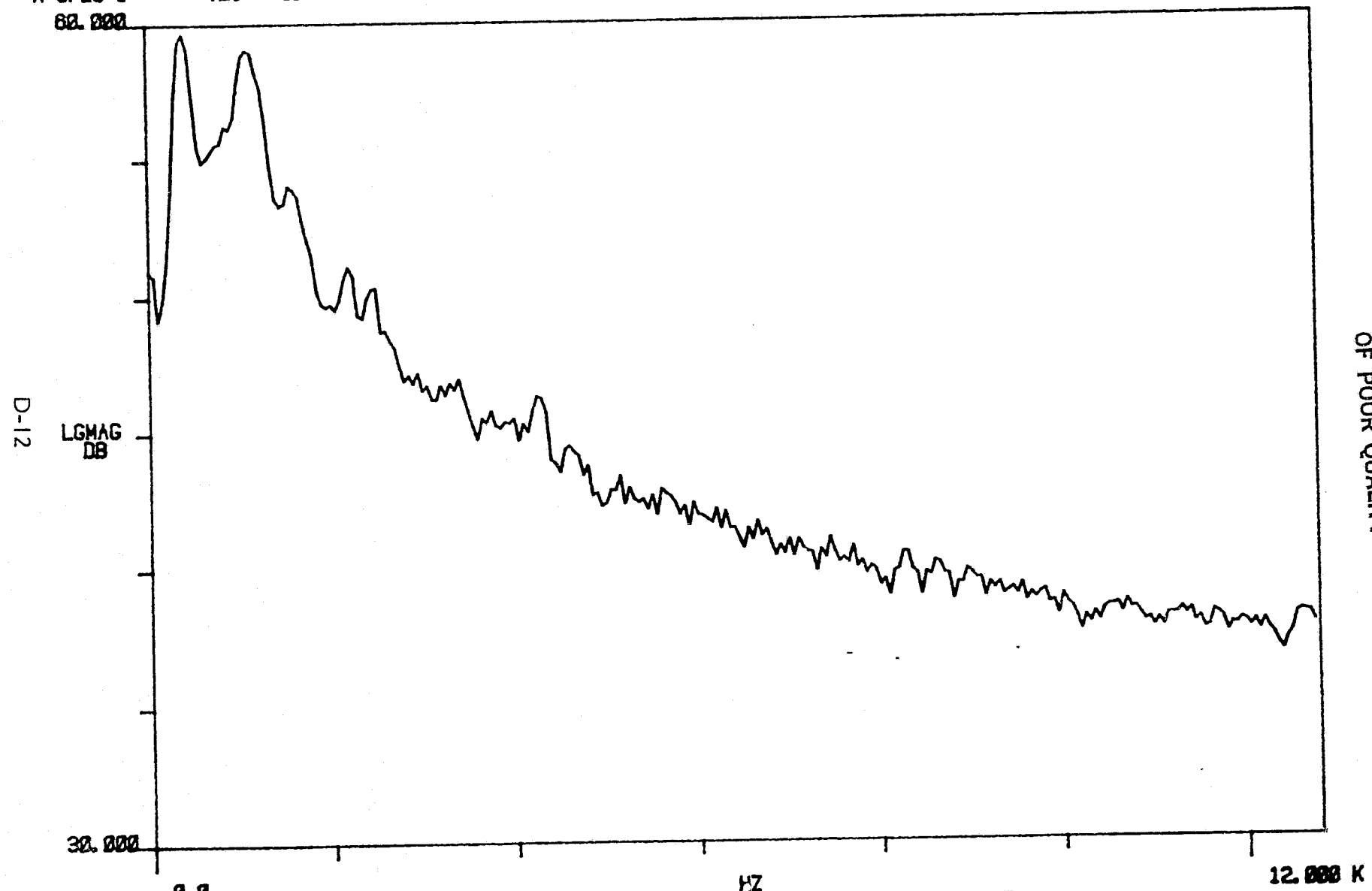
Fig. 10D - A-Weighted Source Contribution Analysis : Exhaust Fans CENTRAL SOYA PLANT (pt. 6B, ch.2)
