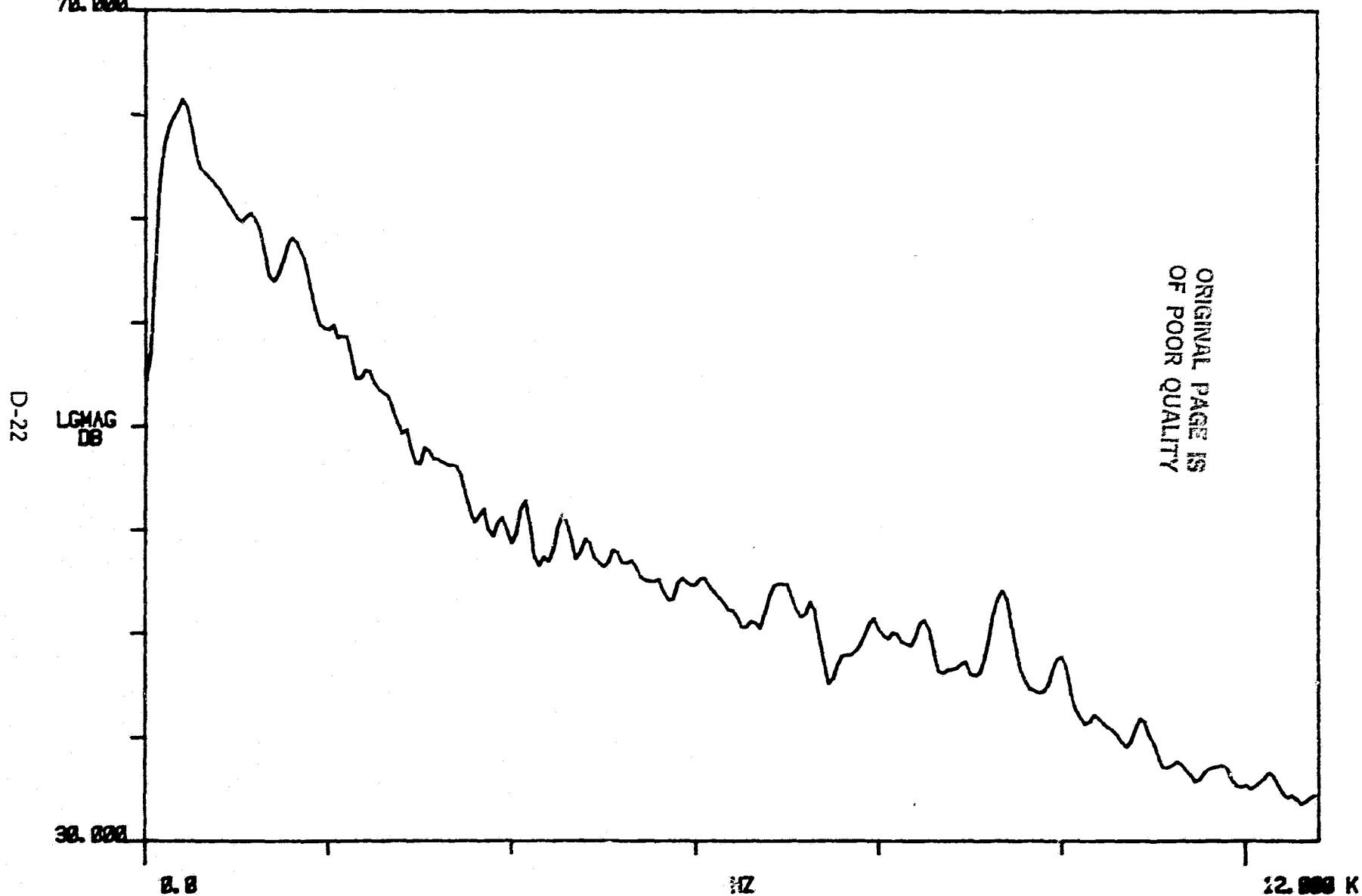
Fig. 20D - A-Weighted Source Contribution Analysis : Shackle Line Foot Remover TIP TOP PLANT (pt. 53, ch.2)
