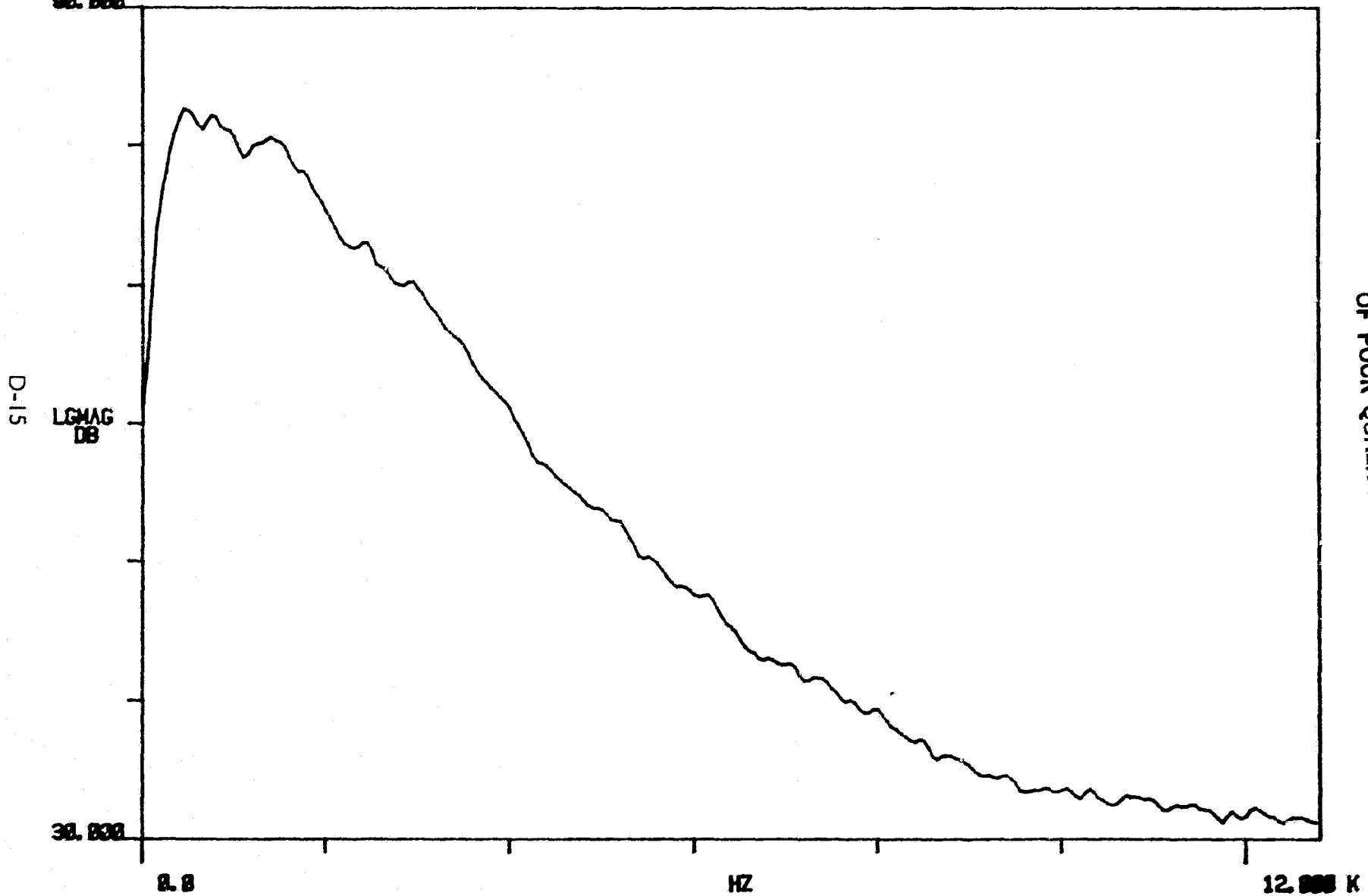
Fig. 13D - A-Weighted Source Contribution Analysis : Chillers TIP TOP PLANT (pt. 53, ch.2)
