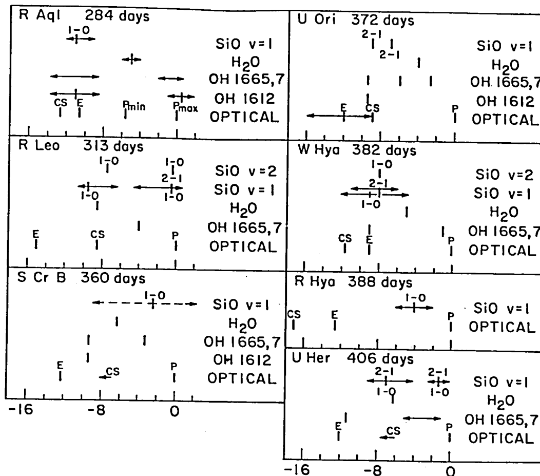
Fig. 8 - Radial velocities of various optical and radio lines plotted relative to the velocity obtained from high-excitation absorption lines (labeled P for "photospheric") for 7 well-studied Mira variables. Characteristic velocities of optical emission (E) and circumstellar (CS) lines are plotted as well as the velocities of radio lines of SiO, H 2 O, and OH. From Wallerstein (1975).
