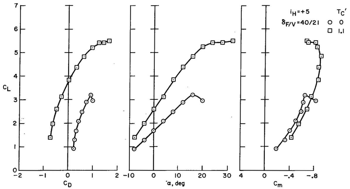
(b) i_H = +5 .
