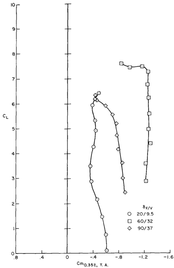
(f) Superposition of tail-off data for a range of flap settings, T'_C = 2.4 .
