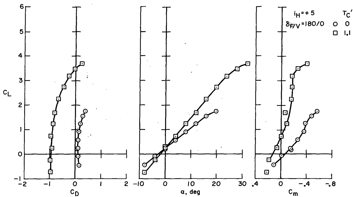
Figure 11.— Basic longitudinal data, \delta_{F/V} = 180/0 (flap stored); i_H = +5 .
