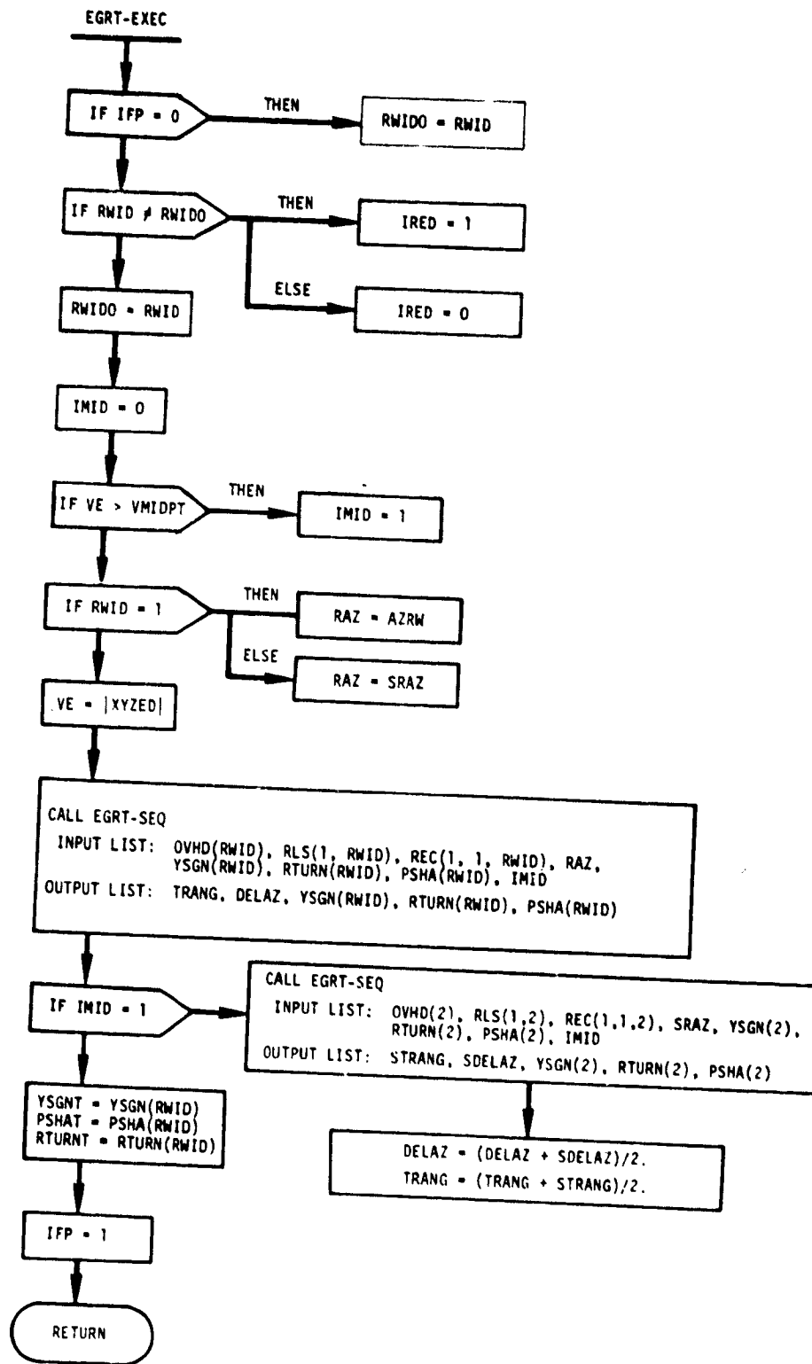
Figure C-1.- EGR-EXEC, targeting executive logic.
