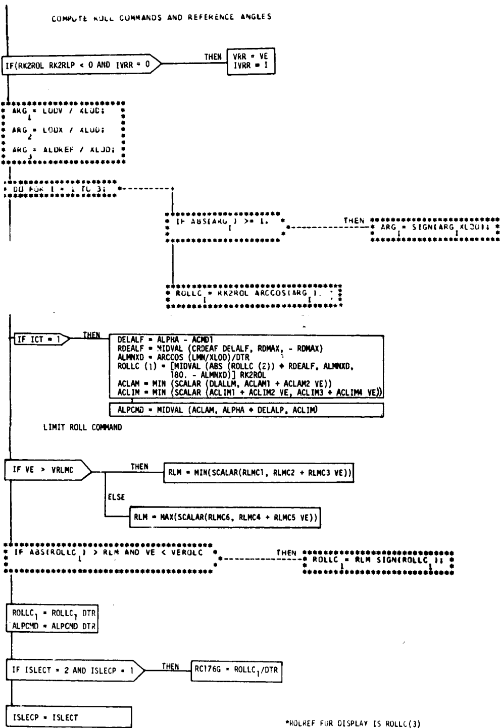
Figure A-13.- EGPOLCMD, roll command.
