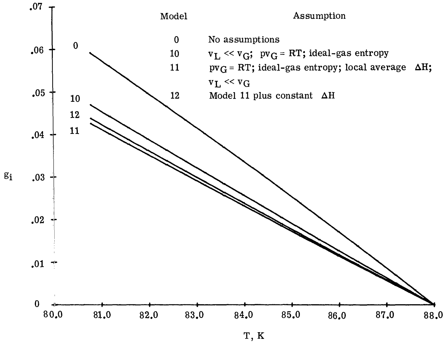
Figure 8.- Isentropic liquid mass fractions g_i for no-assumption and multiple-assumption models. T_C = 88.0 K; p_C = 2.99 atm; T_F = 80.8 K; p_F = 1.47 atm.
