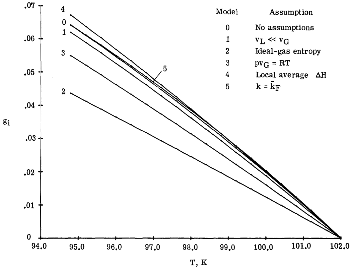
Figure 3.- Isentropic liquid mass fractions g_i for no-assumption and one-assumption models. T_C = 102.0 K; p_C = 8.81 atm; T_F = 94.8 K; p_F = 5.26 atm.
