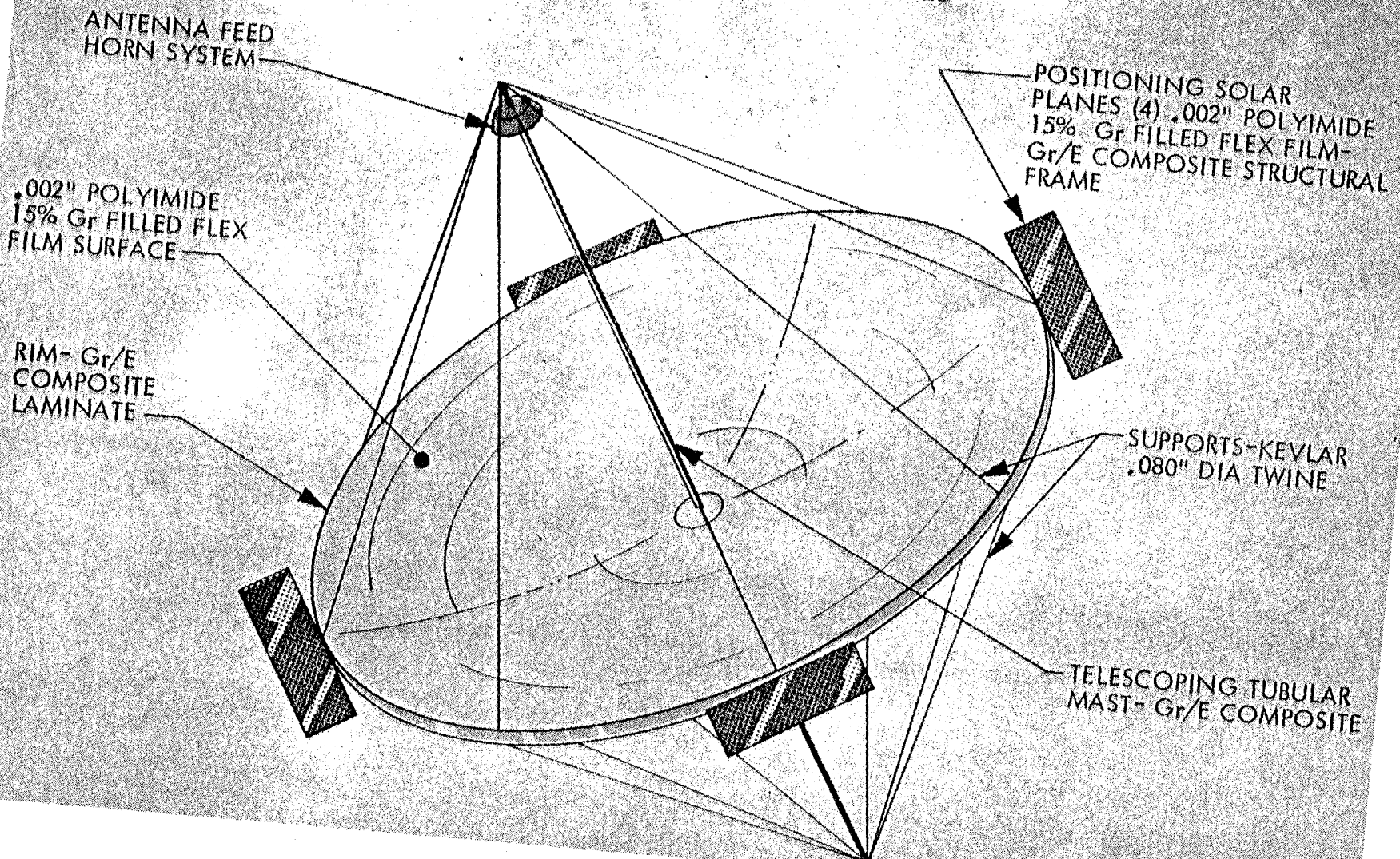
Figure 48. Parabolic Reflector
