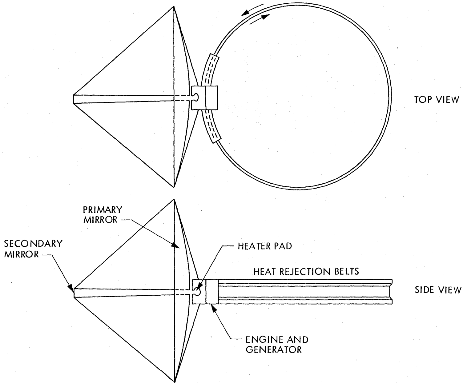
Figure 66. Solar Thermal Space Power Unit
