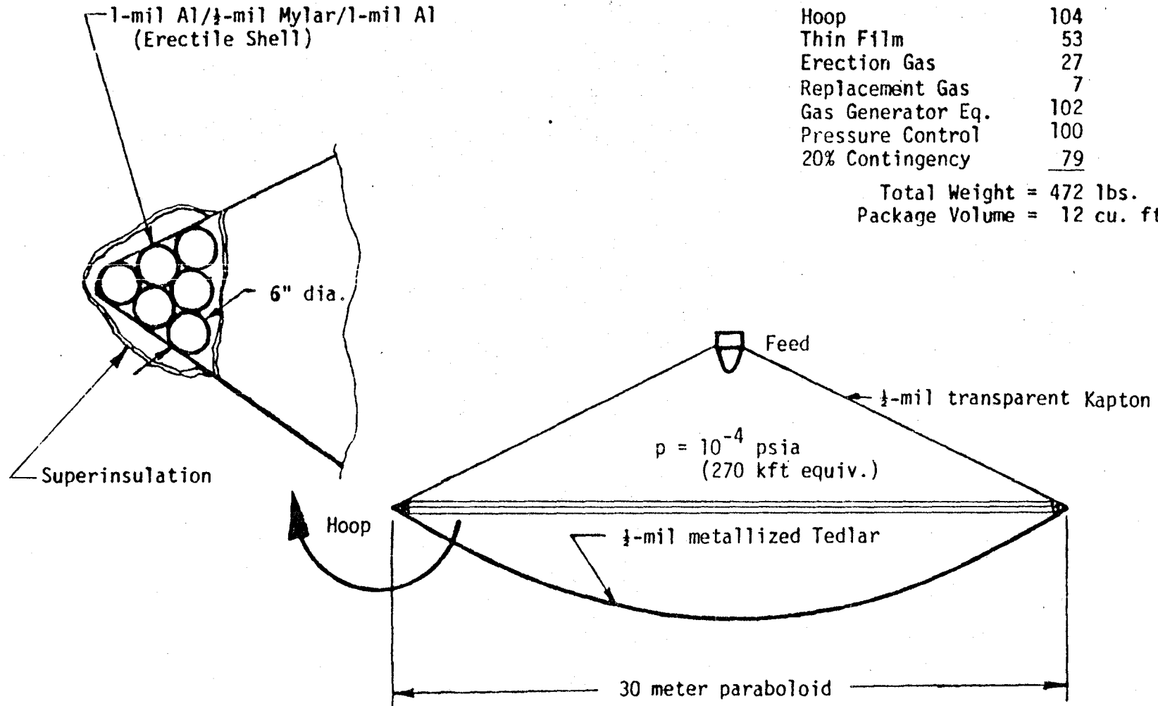
Figure 59. Hybrid Concept
