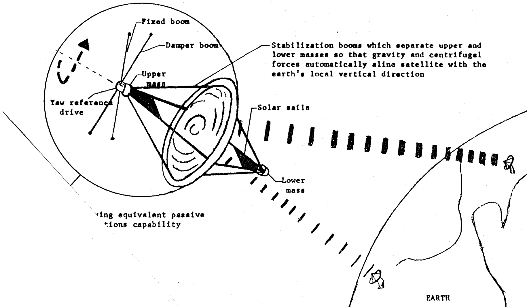
e 24. Gravity-Gradient Stabilized Station-Kept Lenticular Satellite
