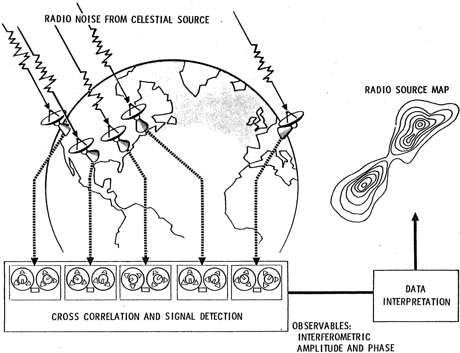
Figure 68. VLBI: High-Resolution Mapping of Celestial Radio Sources
