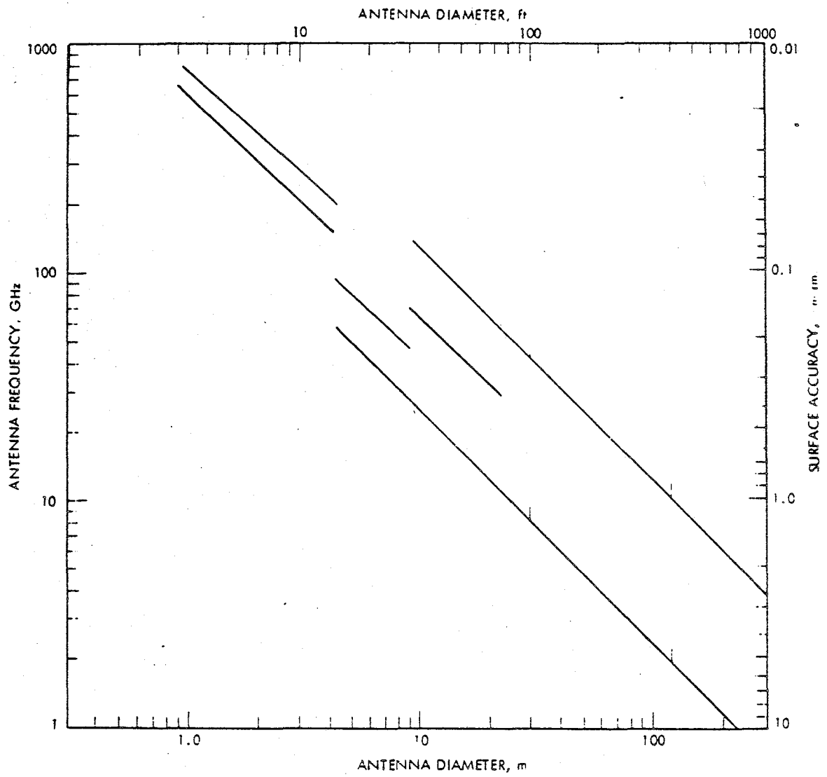
Figure 36. Antenna Surface Precision vs. Size
