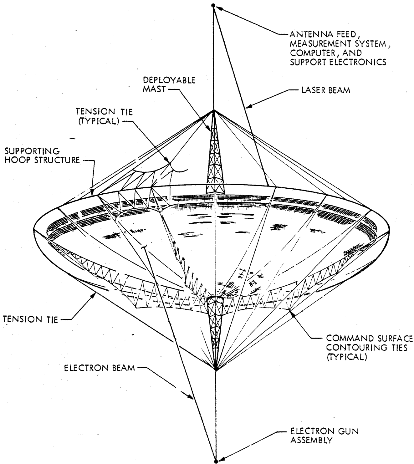
Figure 44. Electrostatically Supported Reflector Surface
