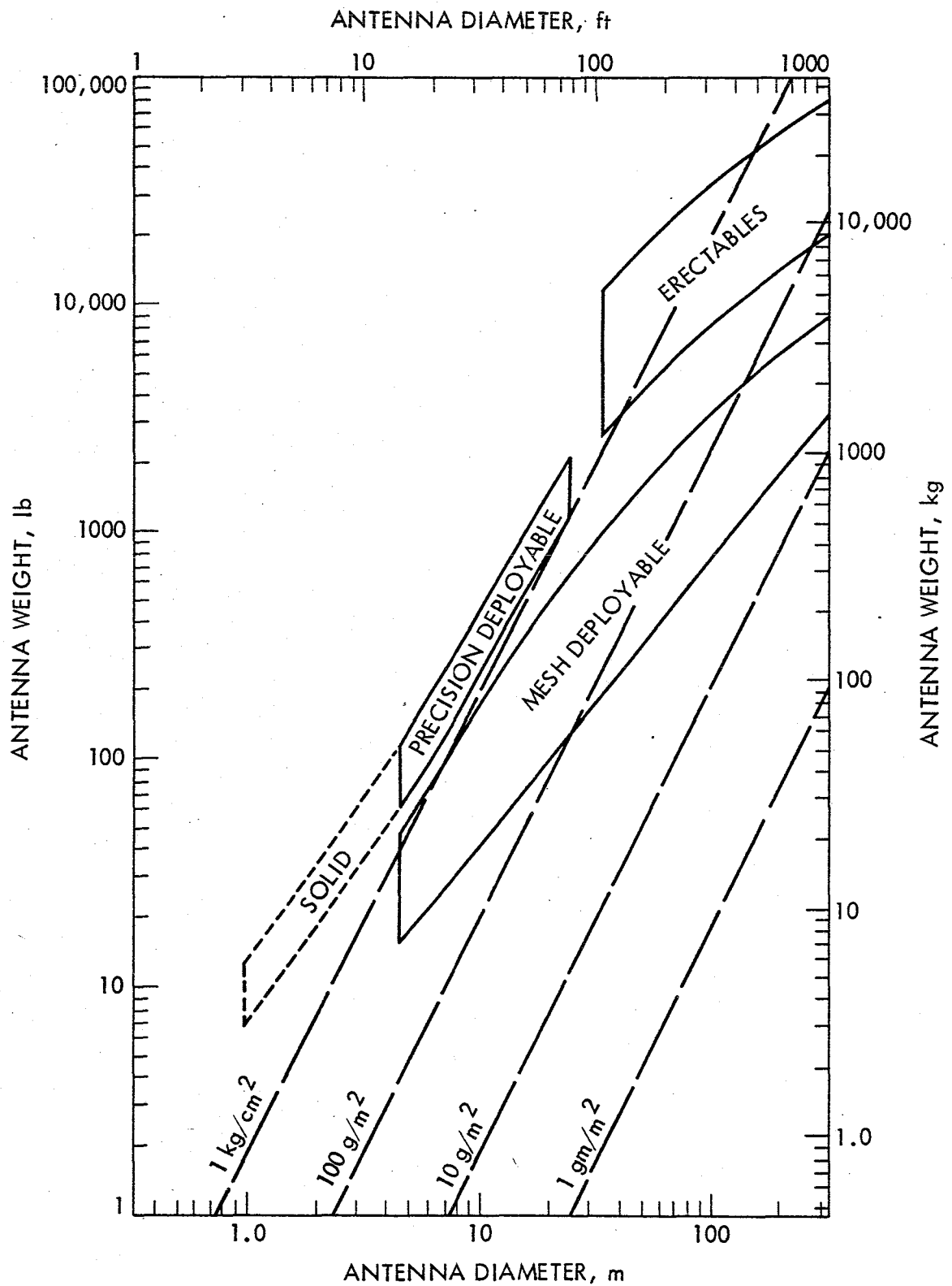
Figure 35. Antenna Weight vs. Antenna Size
