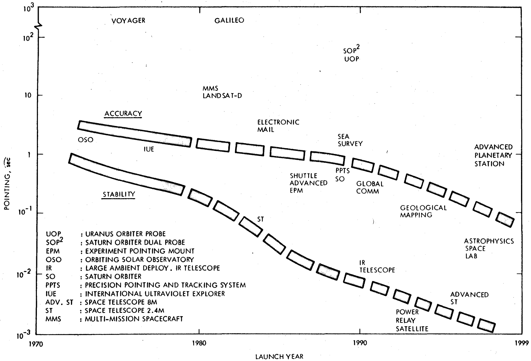
Figure 33. Instrument Pointing Trends
