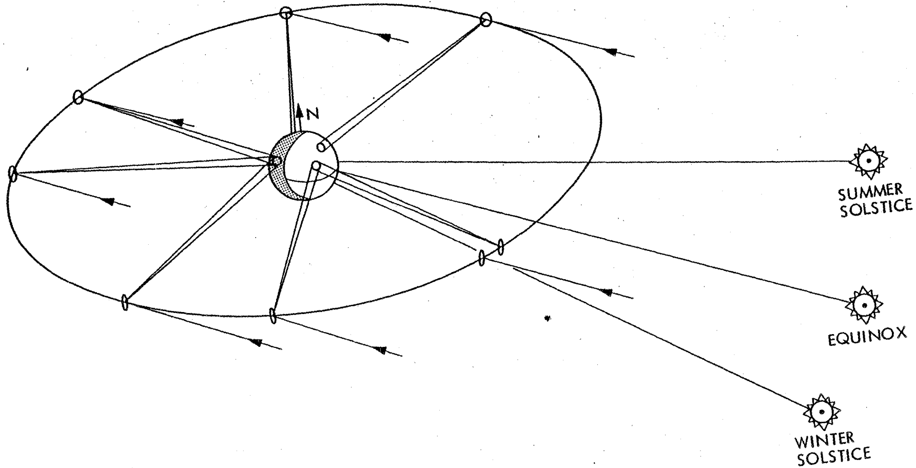
Figure 61. Geostationary System
