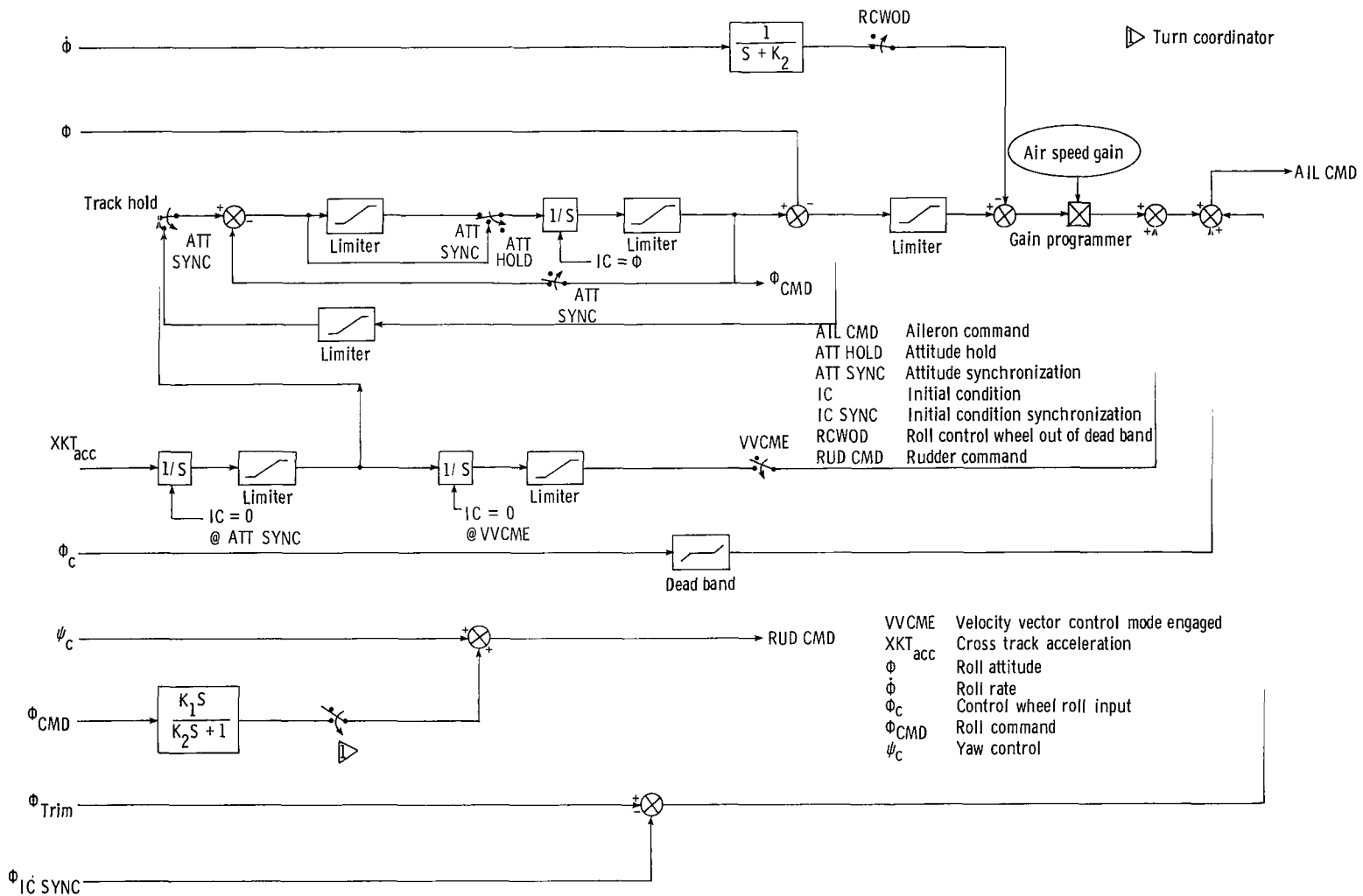
Figure 4.- Block diagram of lateral control system.
