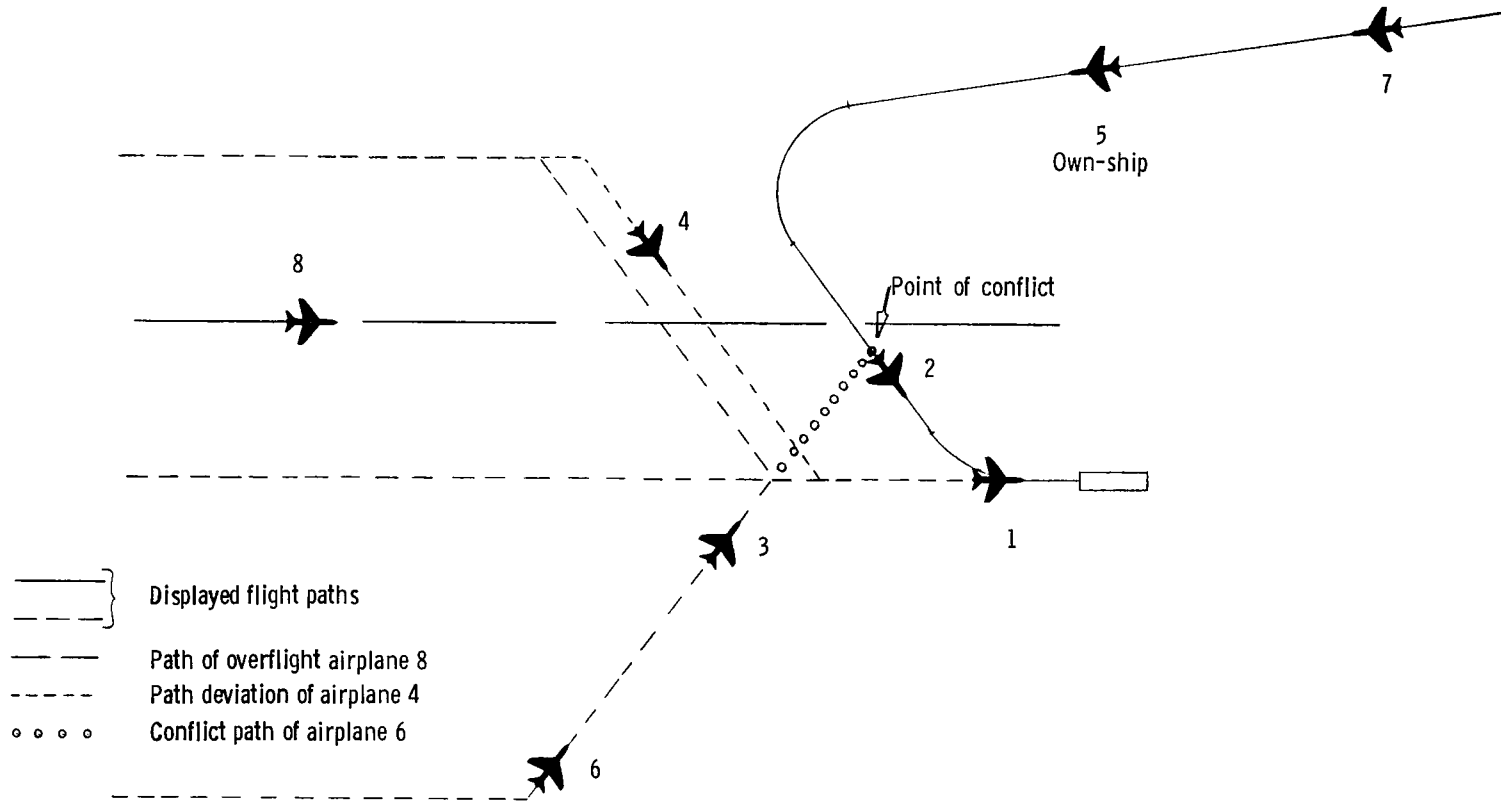
Figure 12.- Traffic scenario C.
