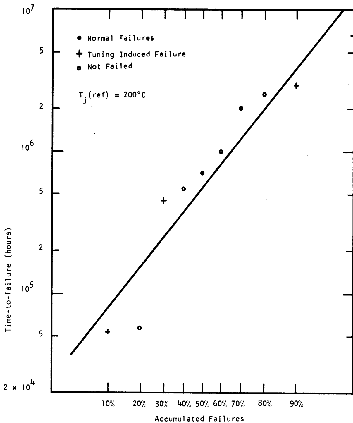
Figure 38 Results of Rf Bias-Temperature Stress Life Test
