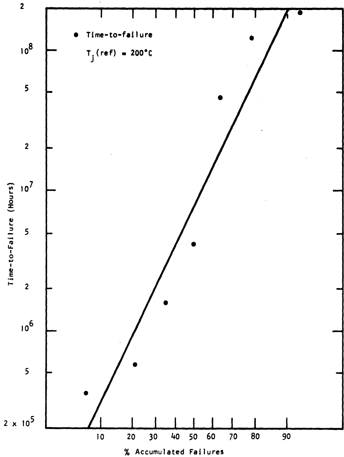
Figure 36 Results of Bias-Temperature Stress Under Non-Oscillating Conditions
