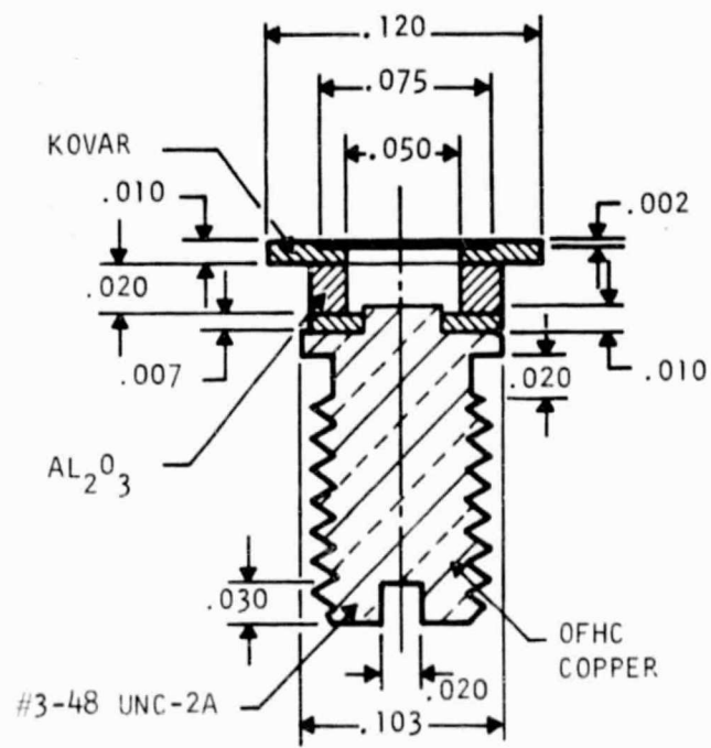
Figure 13 Detail of Package Used for Testing in Waveguide Hat Circuit
