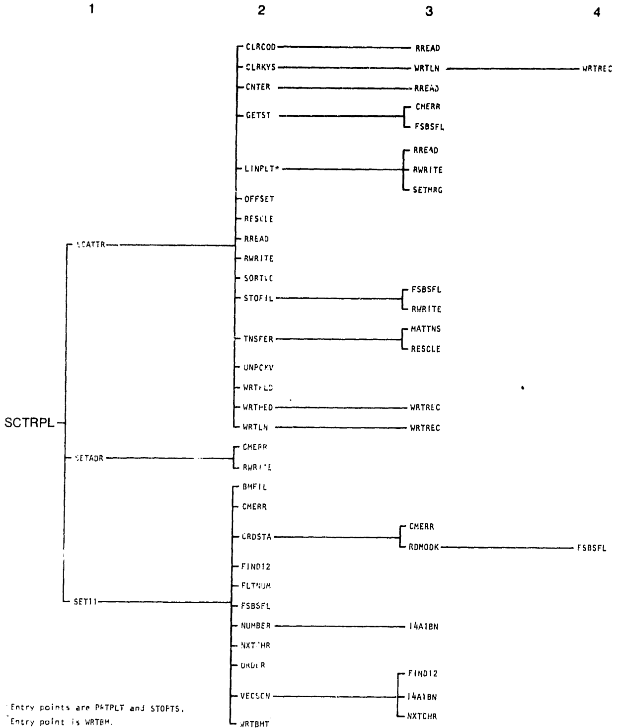
Figure 16-1.— Linkage diagram for the SCTRPL processor.
