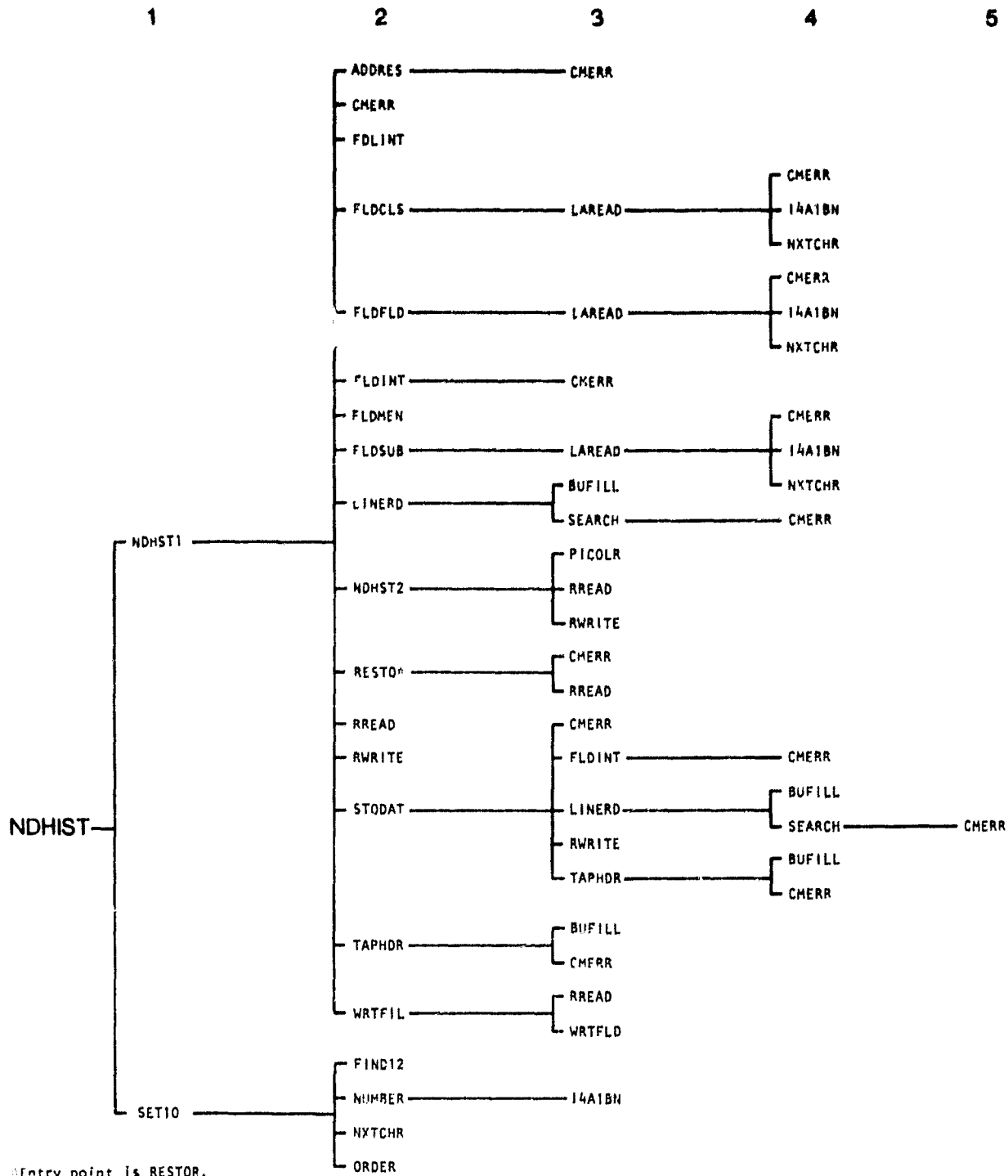
Figure 15-1.— Linkage diagram for the NDHIST processor.
