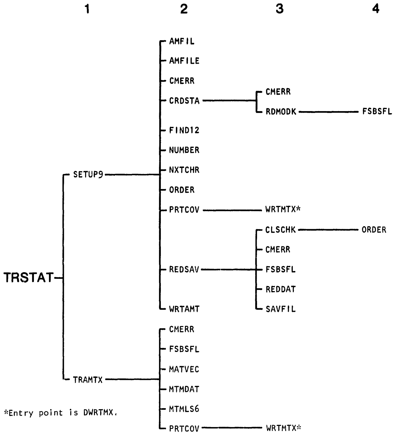
Figure 14-1.-- Linkage diagram for the TRSTAT processor.
