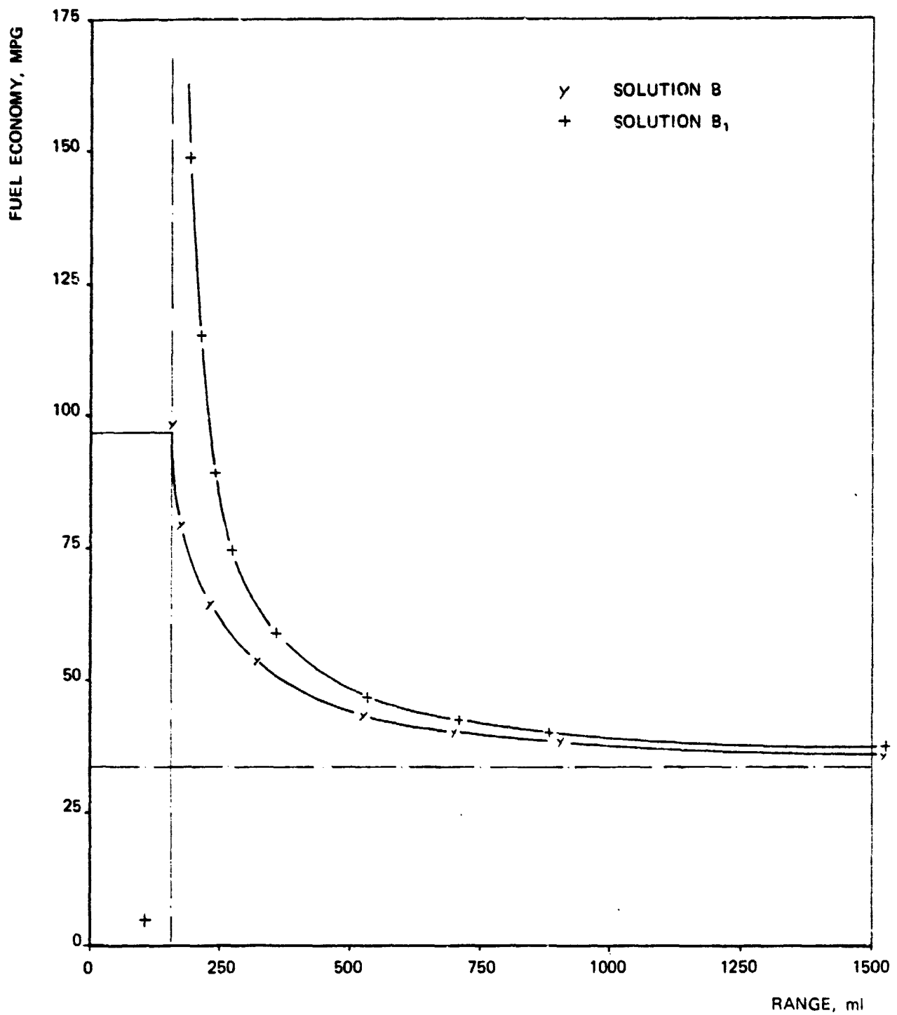
FIG. 6.3-9 - FUEL ECONOMY VS RANGE COMPARISON ON THE FUDC
