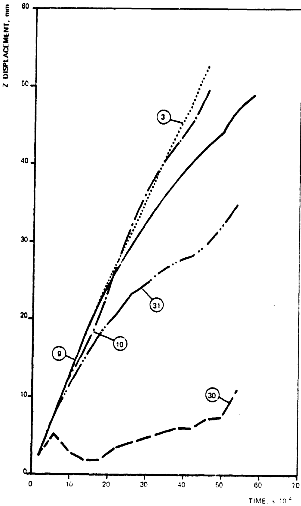
FIG. 7.1-21 - SELECTED VEHICLE NODES (9) DISPLACEMENT DURING CRASH WITH BATTERY
