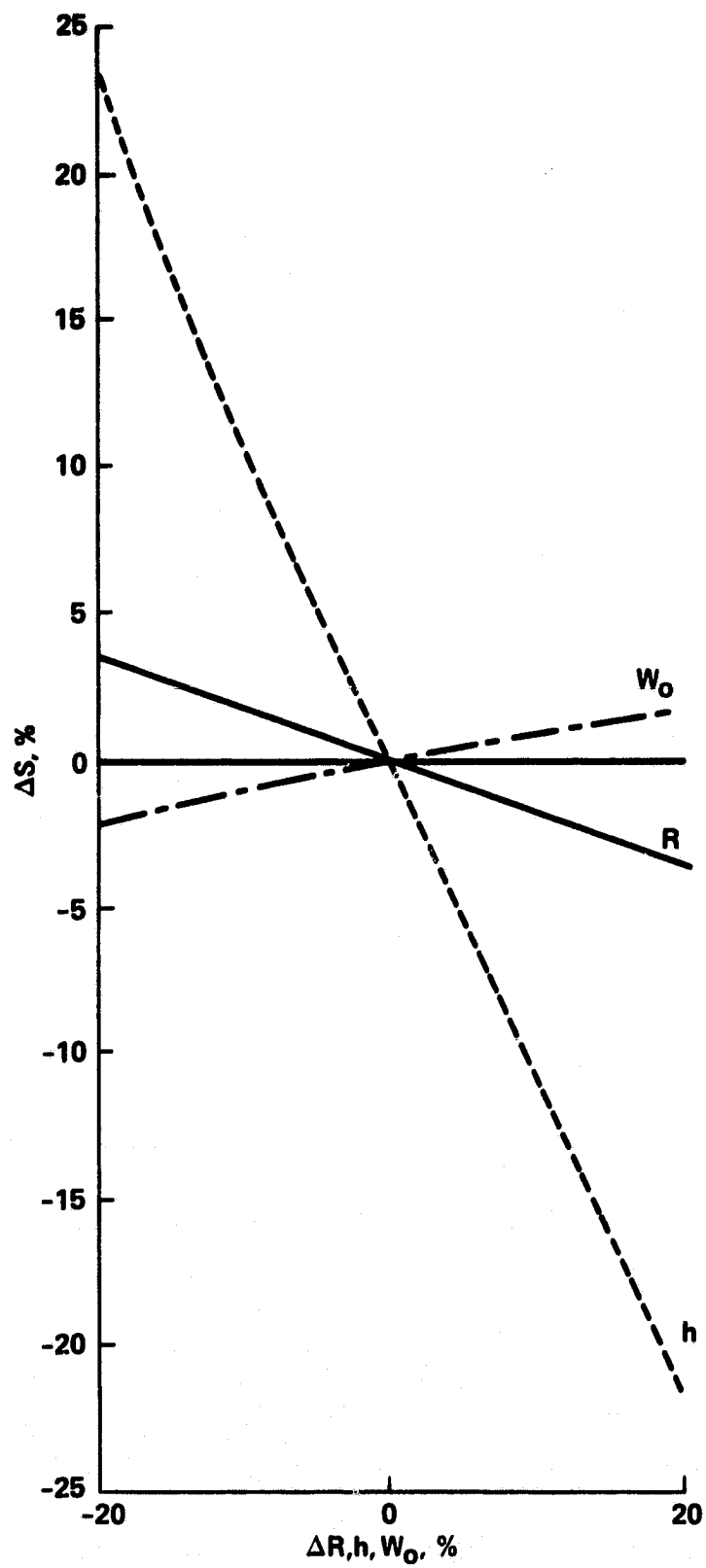
Figure 11.- Sensitivity data for EBBbase for transcontinental mission.
