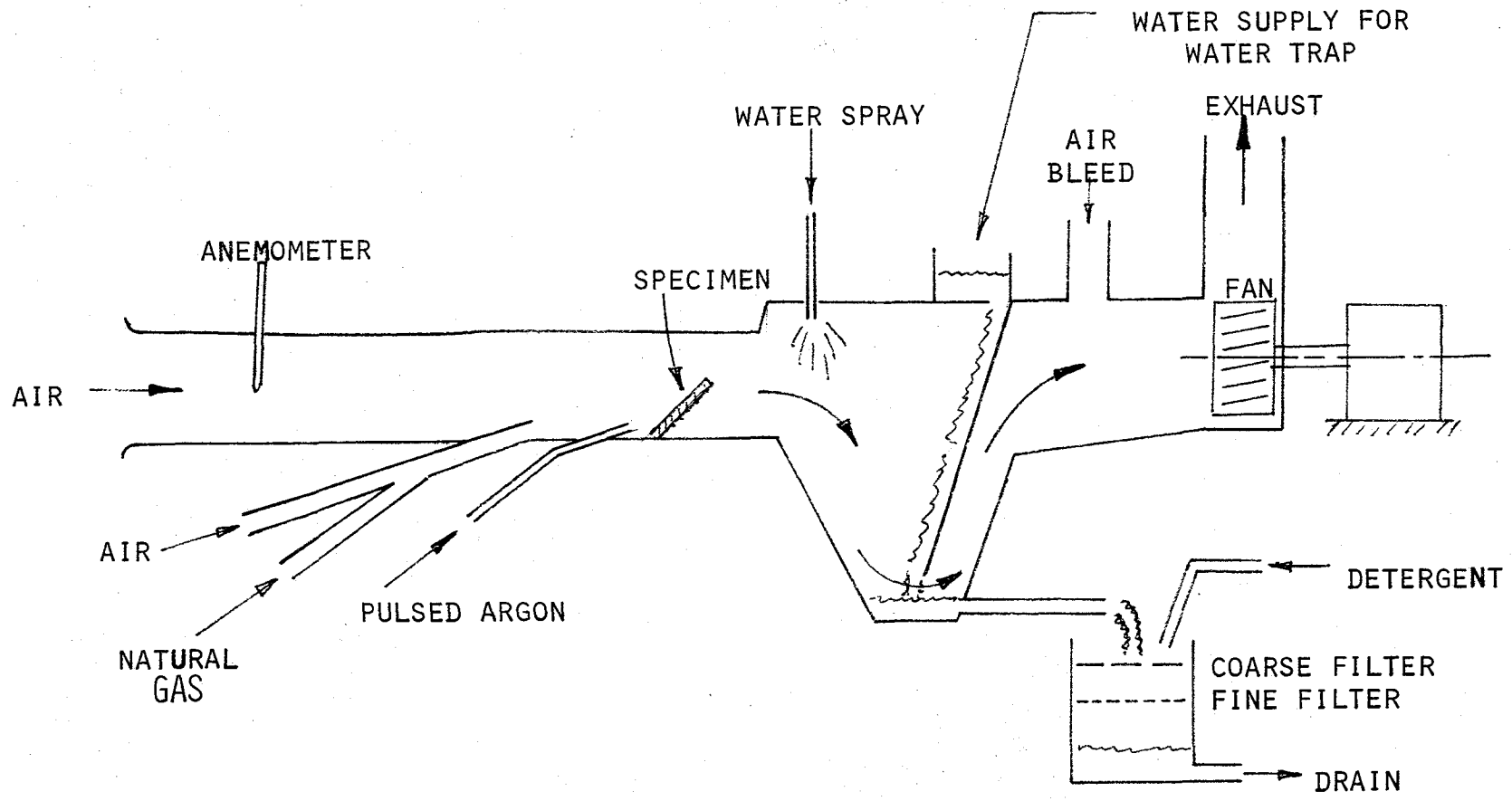
Figure 2. Facility Schematic
