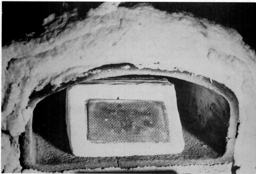
b. Fibers placed in firebrick cavity
