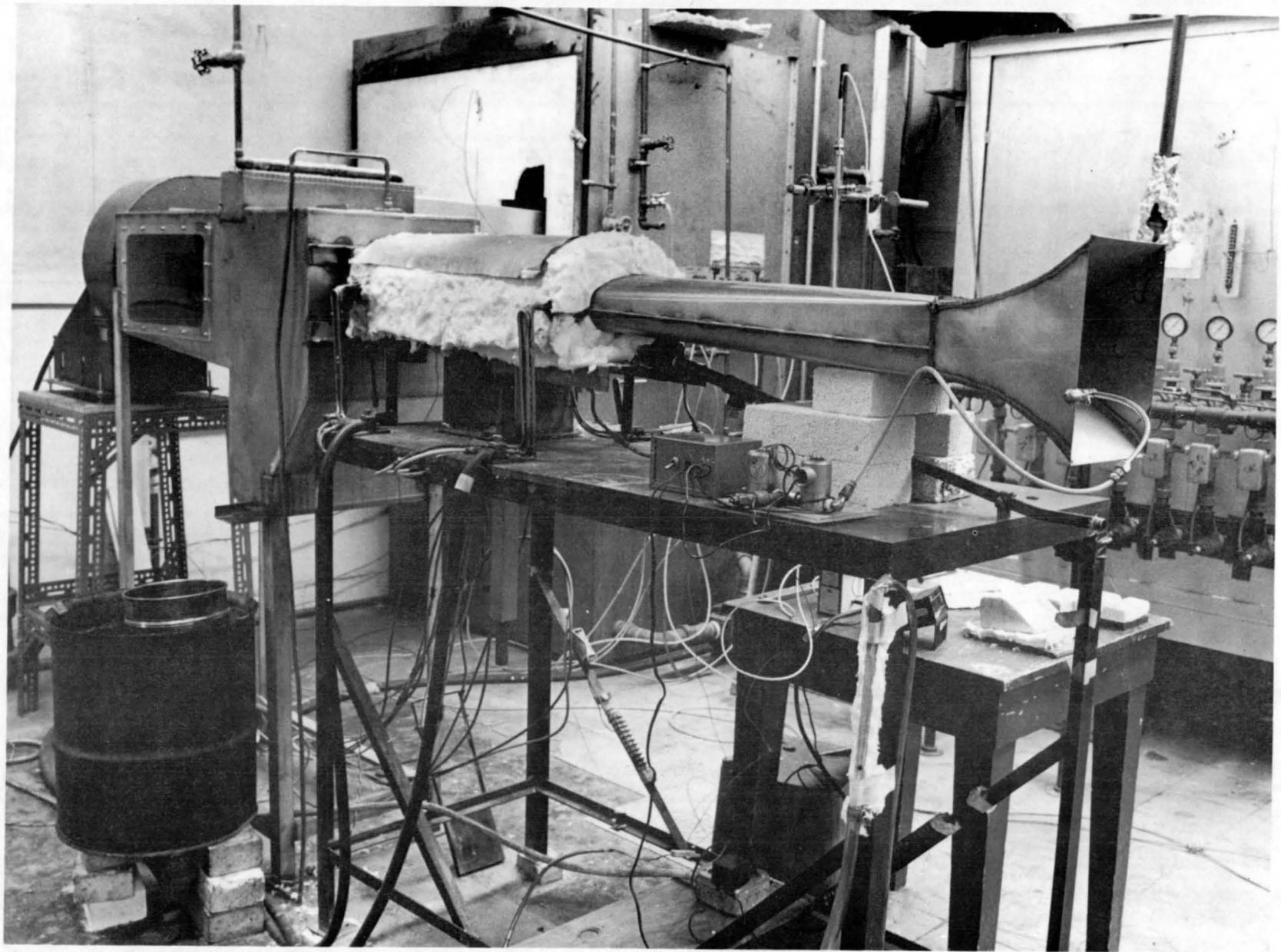
Figure 3. Modified Model 25 Facility
