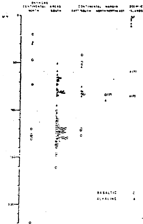
Fig. 10 — Age and regional distribution of the Mesozoic-Cenozoic volcanism in Brazil. Data from Hennes and Hasui (1965); Cordani and Hasui (1968); Cordani and Elazekovic (1970); Hasui and others (1973); Donusceno (1966); Cordani (1970); Amiral and others (1967); Vandroos and others (1966); Ribeiro and Cordani (1966). (After Asmus, 1973).
