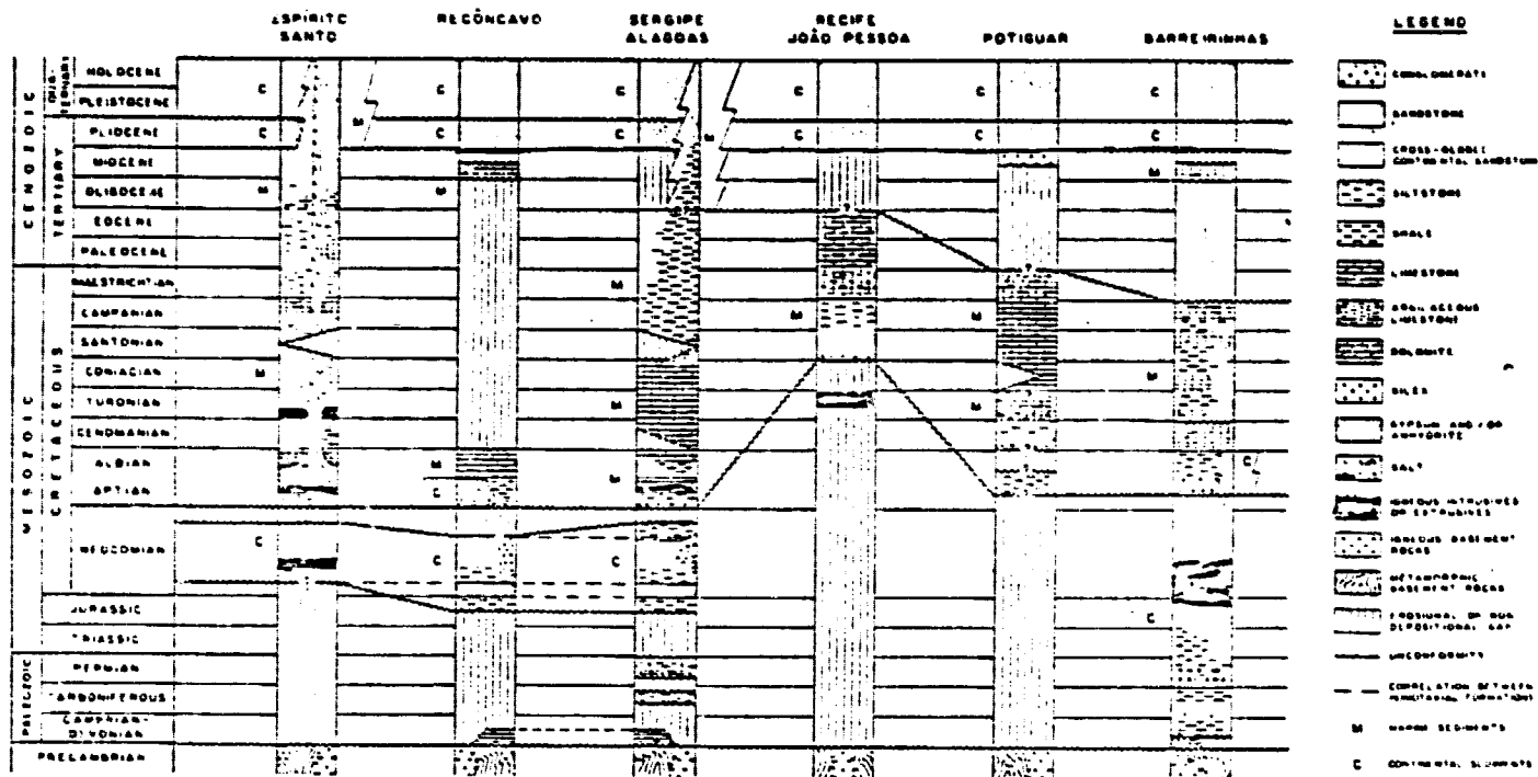
Fig. 2. Stratigraphic correlation chart from Barreirinhas basin to Espírito Santo basin.
