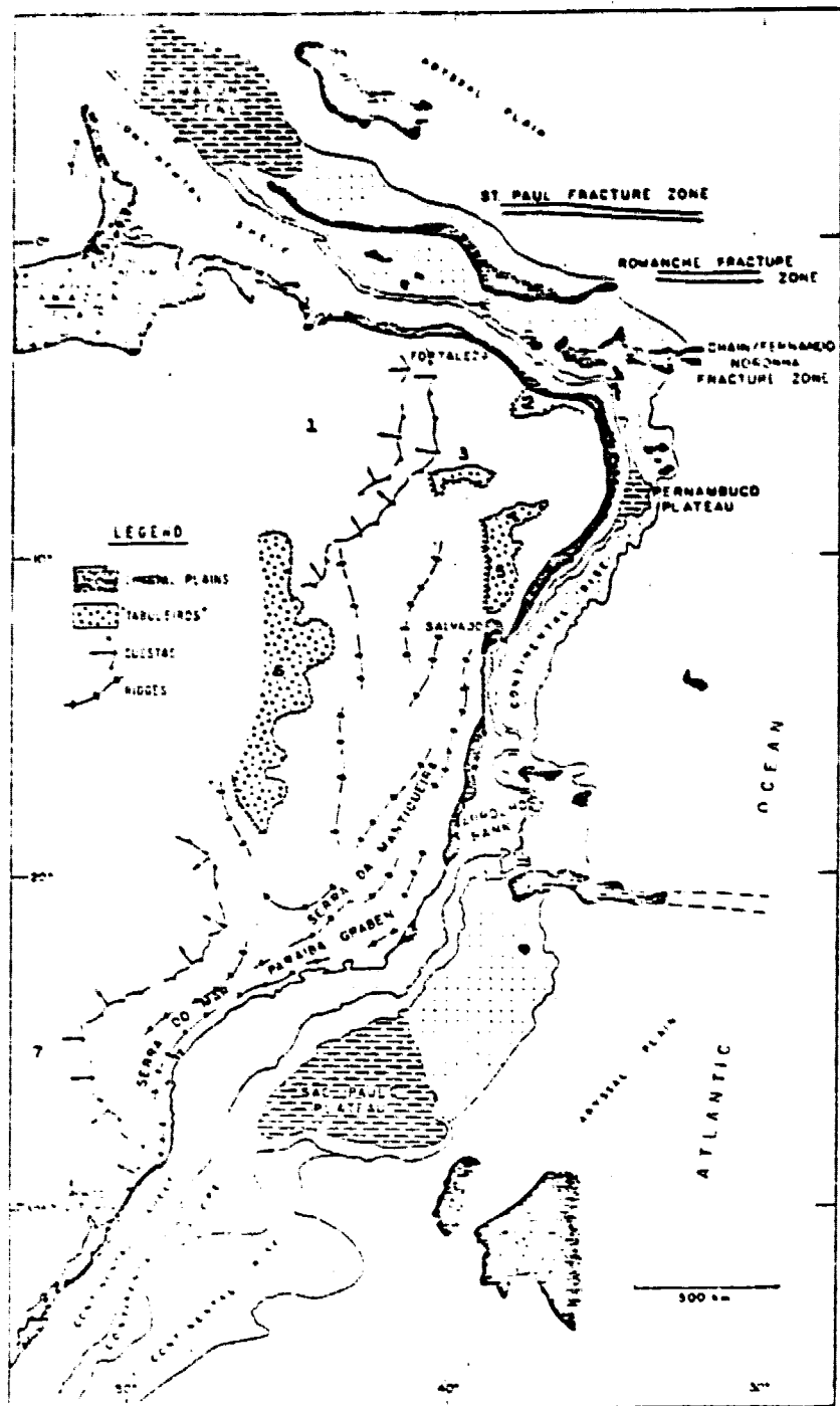
Fig 6 — Physiographic map of the Brazilian continental margin. 1 — Maranhão sedimentary basin; 2 — "Chapada" Apodi; 3 — "Chapada" Araripe; 4 — "Tabuleiros" Jataí; 5 — "Tabuleiros" Tucano; 6 — "Chapadões" Urucua; 7 — Parana basin. (Modified from Asmus, 1973).
