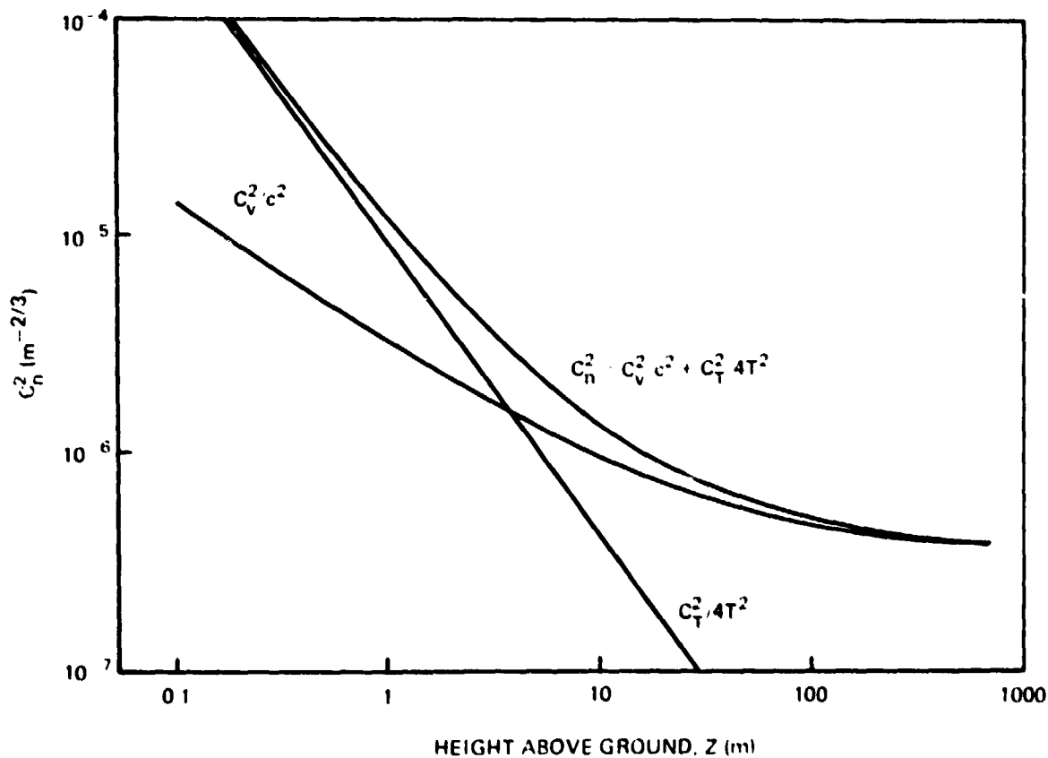
Figure 4.-Typical variation of structure parameters with height above ground. Calculated according to eqs. 18 and 19. T = 283K.
