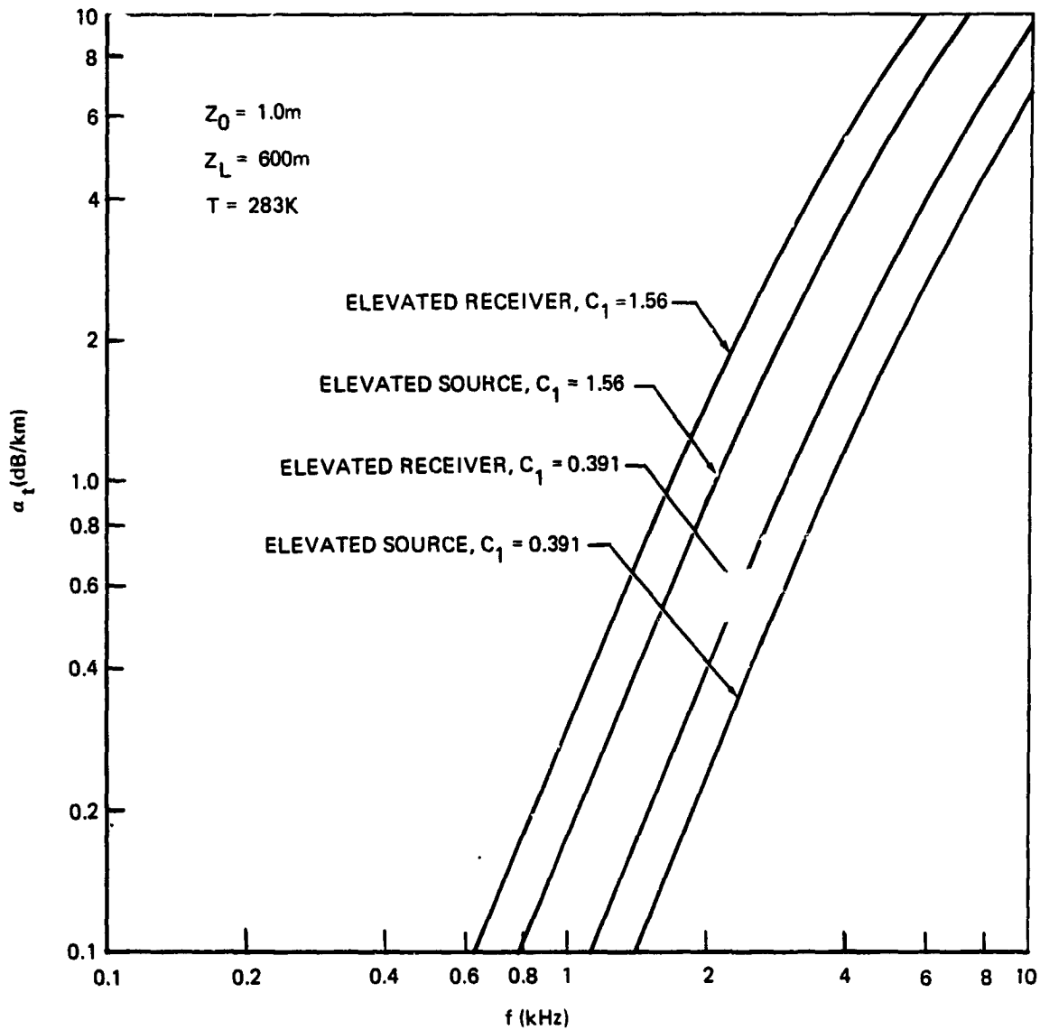
Figure 9.-Variation of turbulence-induced attenuation, \alpha_t , with frequency, f . \alpha_t according to eq. (22).
