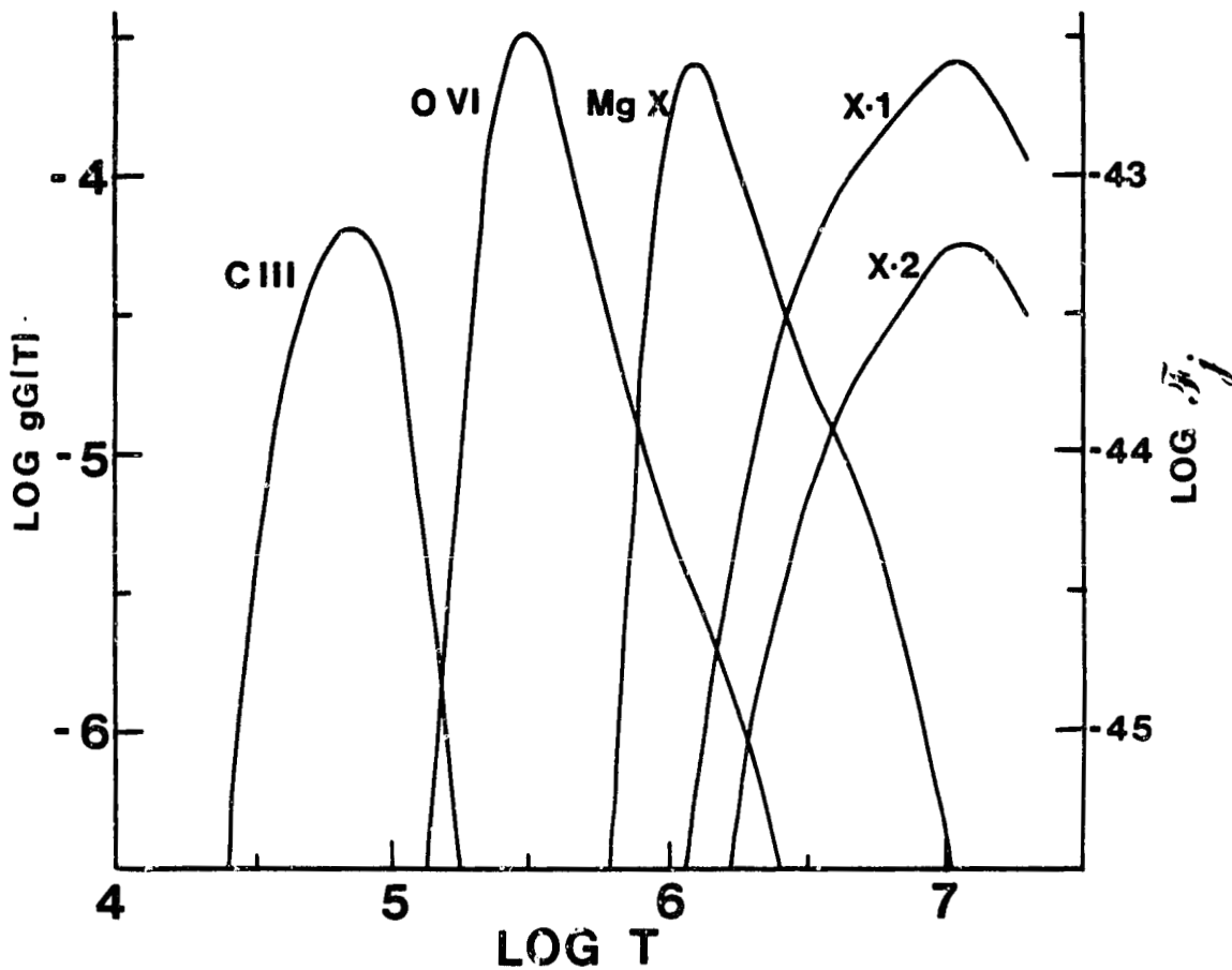
Figure 1. Values of \log gG(T) for the Three EUV Lines That Were Used in this Study (Given by the Left-Hand Scale) and Values of \text{Log } z_j for the Two X-Ray Bands Used in the Study (Given by the Right-Hand Scale).
