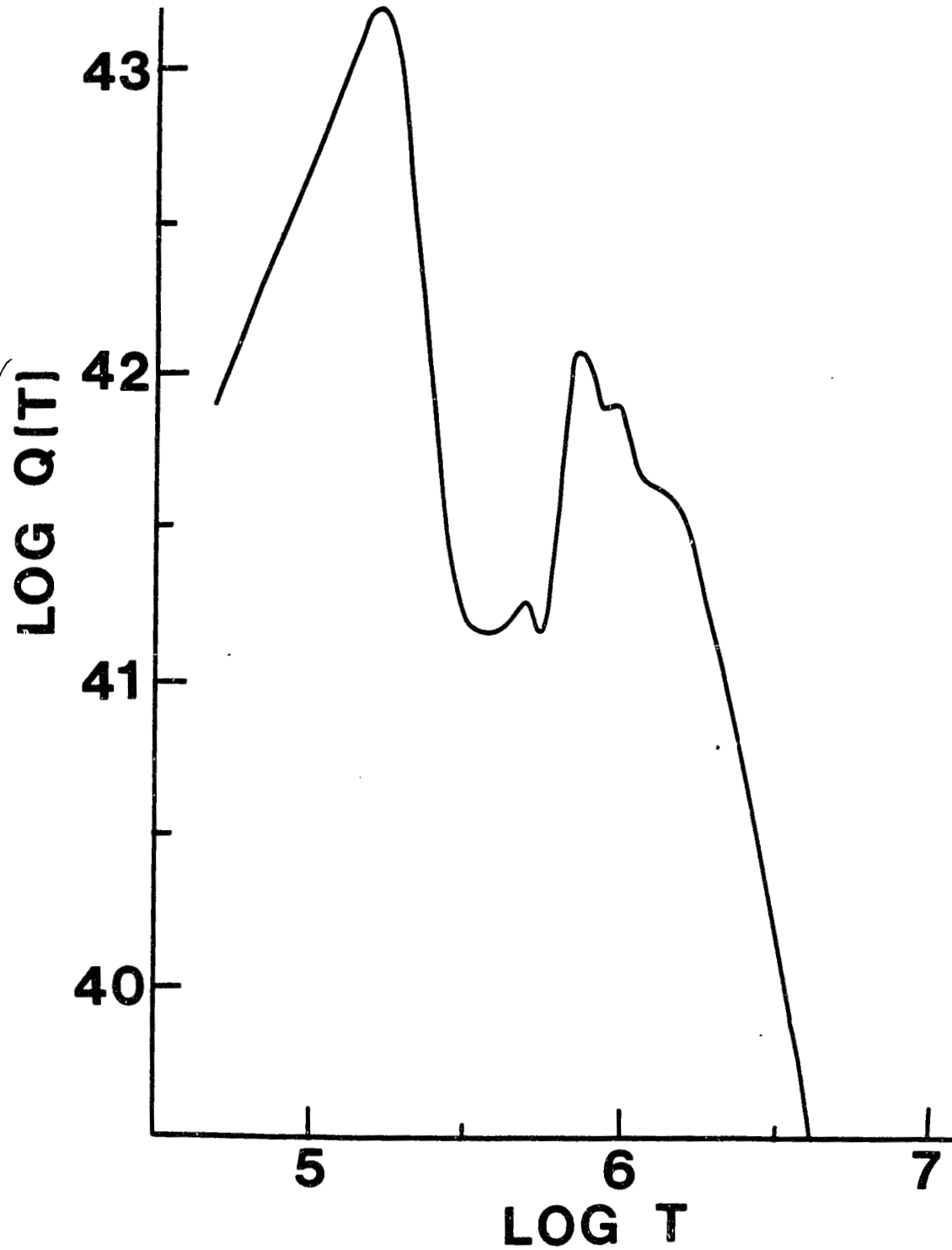
Figure 2(b). Emission Measures Q(T) for the Coronal Active Regions. Region 12375 at 2029 UT on 6 June 1973.
