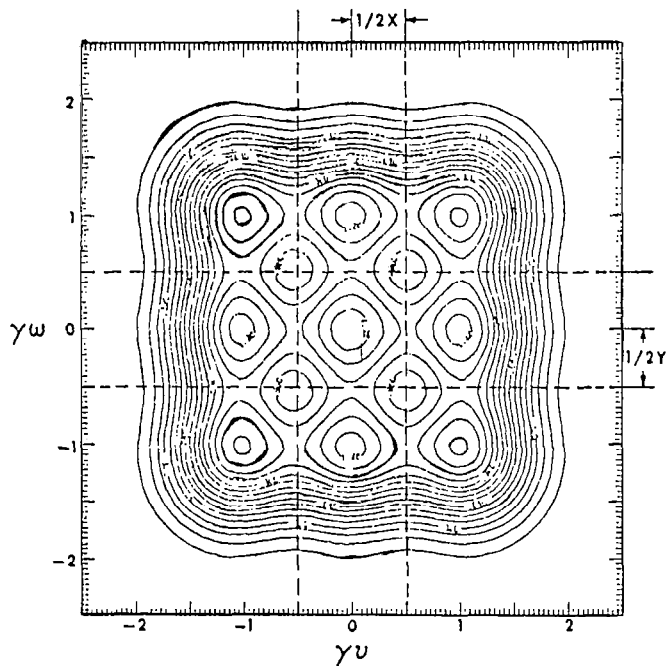
(a) Contiguous coverage (i.e., X/Y = Y/\gamma = 1 ) with discretely stepped circular photosensor aperture.
