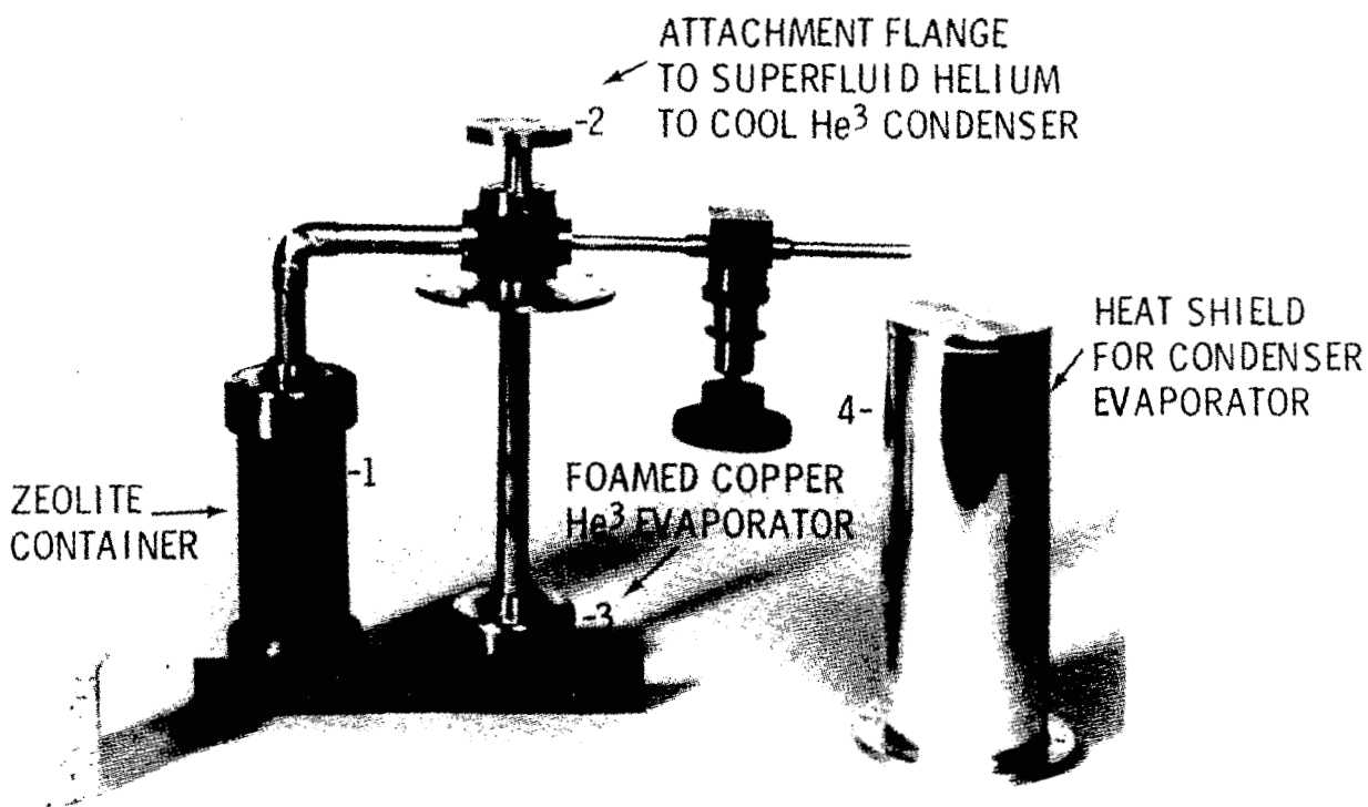
Figure 7.- He 3 cooler prototype designed by Ames Research Center.
