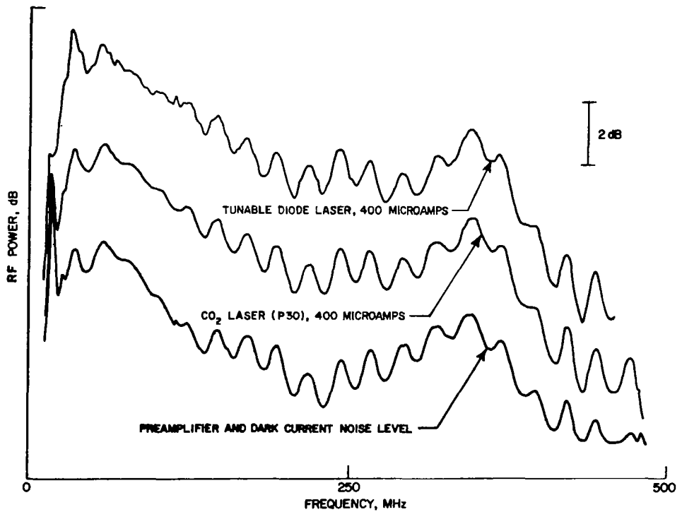
Figure 6.- Comparative RF noise measurements for CO 2 and semiconductor lasers.
