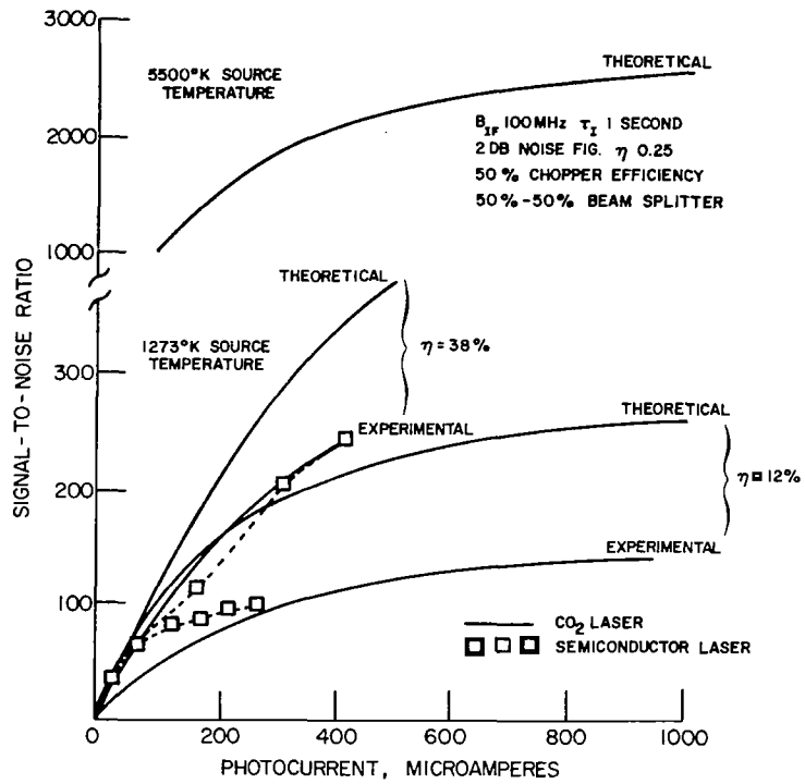
Figure 5.- Comparative signal-to-noise measurements for CO 2 and semiconductor lasers.
