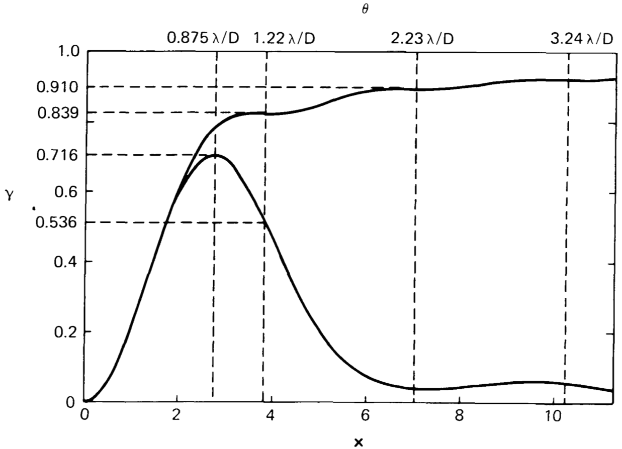
Figure 3.- Heterodyne efficiency for Airy function signal distribution on circular detector. Both curves are for circular detector of radius r = F\lambda x/\pi and Airy function signal field distribution. Upper curve is for matched local oscillator field distribution on detector, which gives maximum possible signal-to-noise ratio. Lower curve is for usual case of uniform local oscillator field distribution on detector. Angular radius detector is indicated on upper axis for peak of lower curve ( x = 2.75 ) and first three Airy dark rings ( x = 3.83, 7.02, \text{ and } 10.2 ).
