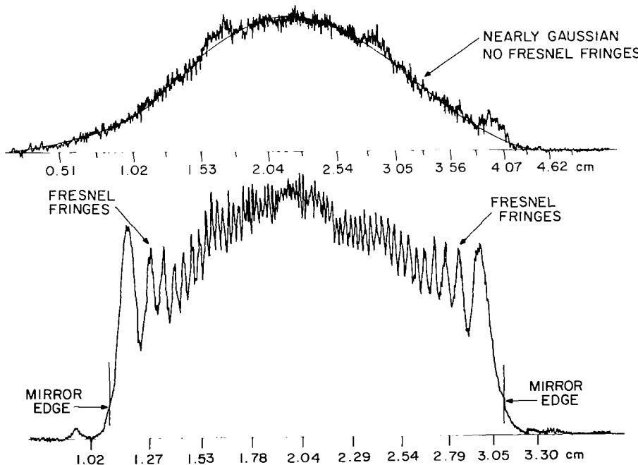
Figure 2.- CO 2 laser beam cross section. Upper plot shows nearly Gaussian output beam. Lower plot shows edge diffraction of beam by undersize mirror resulting in Fresnel interference fringes on laser beam profile.
