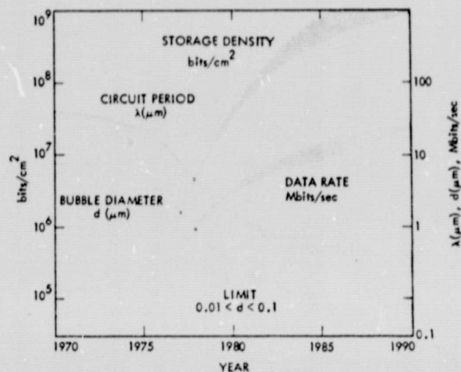
Figure 3-3. Bubble memory technology. About 4 \times 10^8 bits/cm² would be reached in 1985. This implies a bubble diameter of 10^{-5} cm, which is ten times greater than the theoretical limit. (Adapted from A.H. Bobeck, Bell Laboratory, ELECTRO '77, N. Y.).
