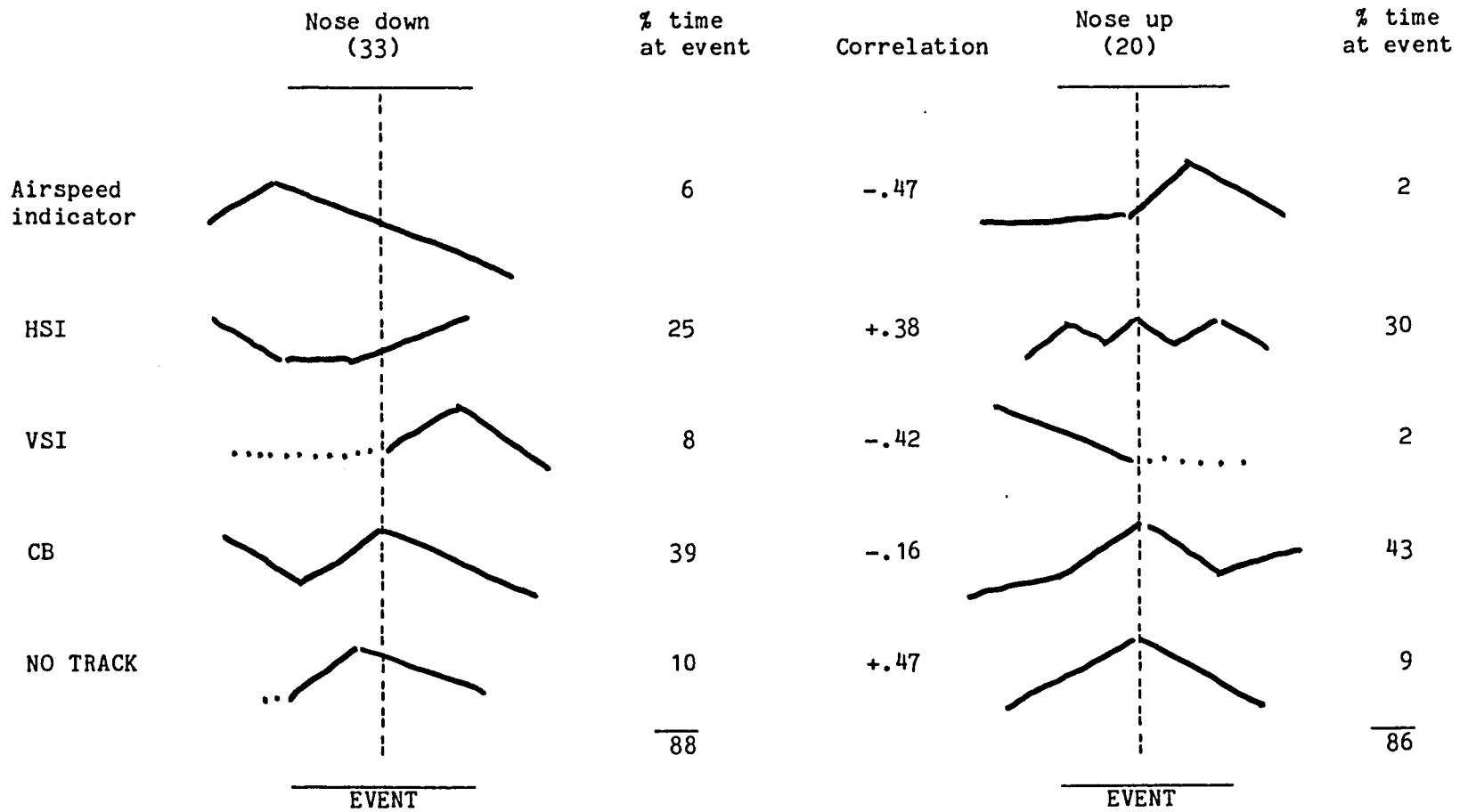
Figure 5b. Pilot 1. Eight Landings, Climbing - Column Movement.
