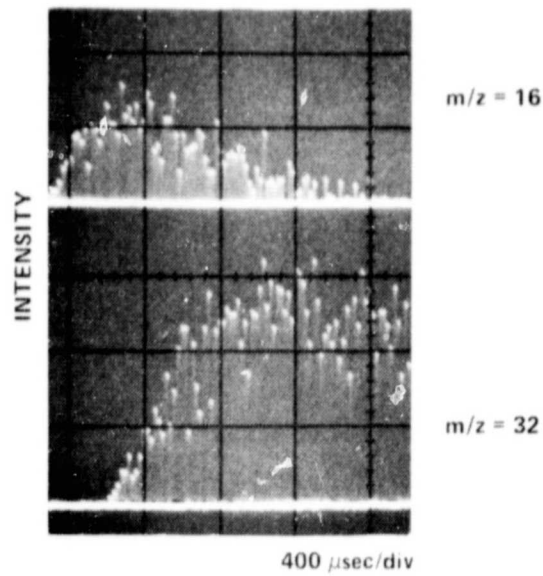
Figure 5. Two time-resolved masses from pulsed laser-heated \text{Al}_2\text{O}_3 .
