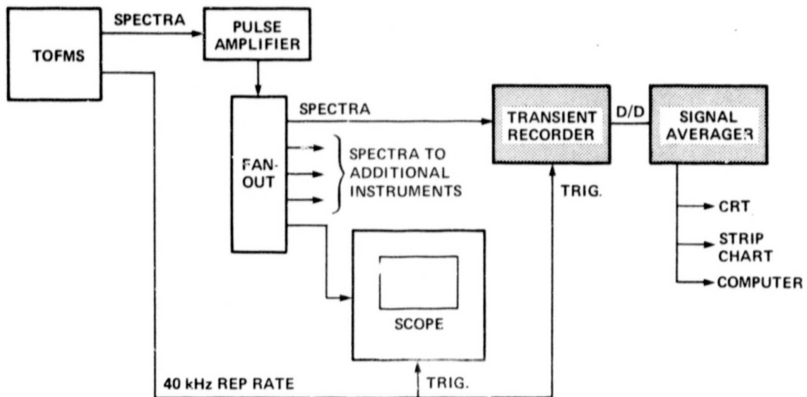
Figure 6. Instrumentation for accumulating spectra in signal averager.
