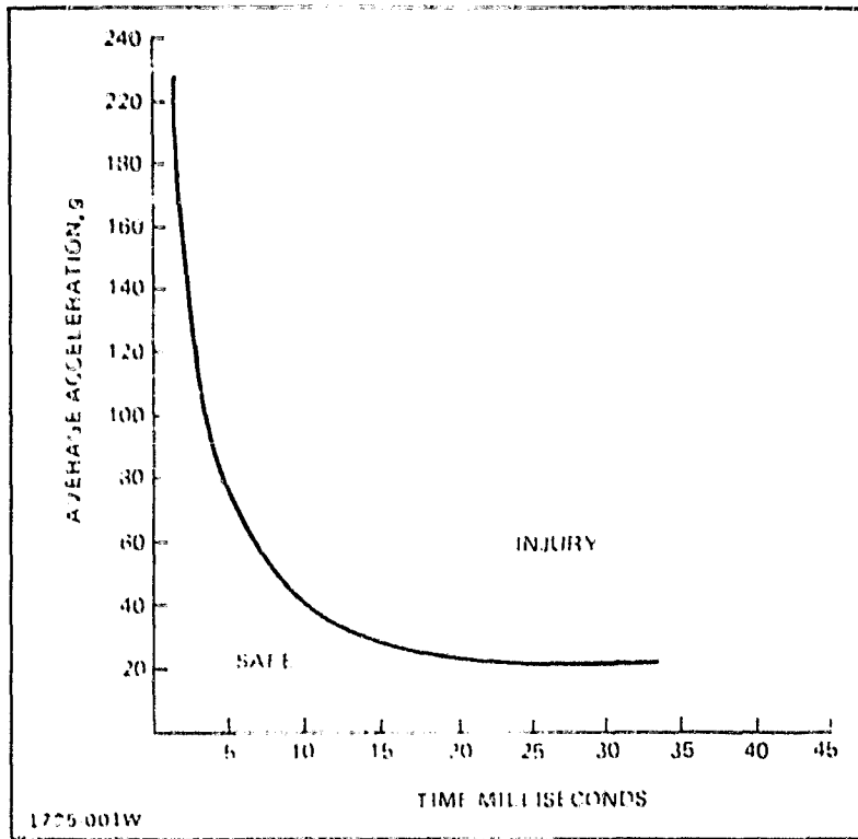
Fig. 10 Wayne State University Cerebral Concussion Tolerance Curve
