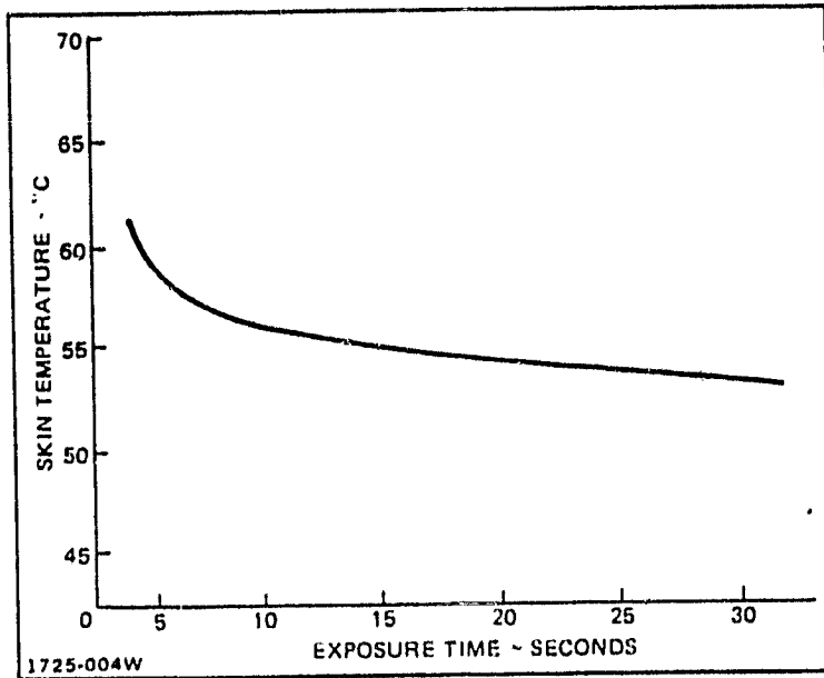
Fig. 1 Exposure Conditions for Threshold Blister
