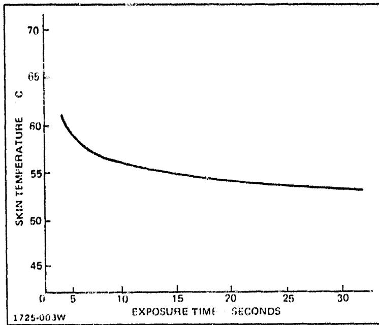
Fig. 1 Exposure Conditions for Threshold Blister
