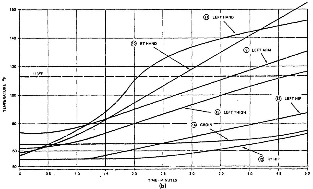
Fig. 8 Class 3 Heat Tests - Ensemble No. 1
