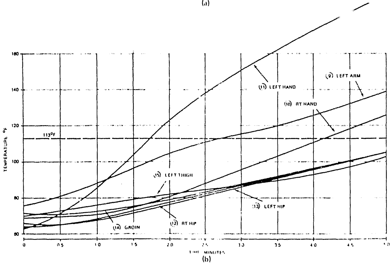
Fig. 9 Class 3 Heat Tests Ensemble No. 2
