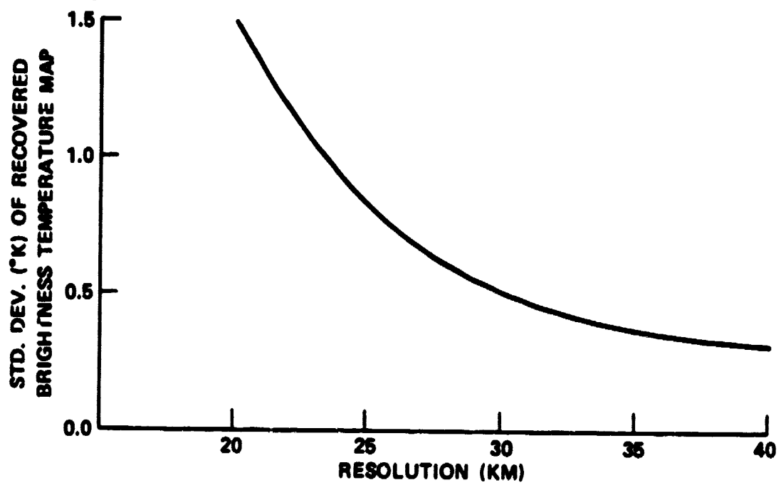
Figure 4. Standard Deviation of the Estimated Brightness Temperature Map as a Function of Resolution
