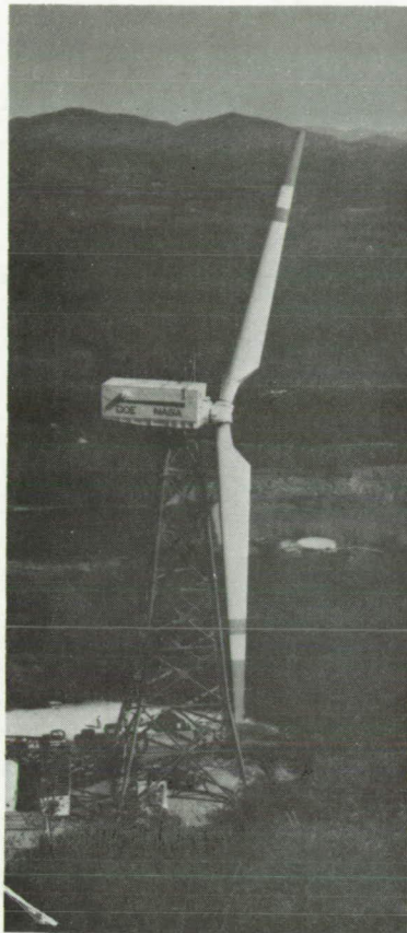
FIRST GENERATION (MOD-0A AND MOD-1)
