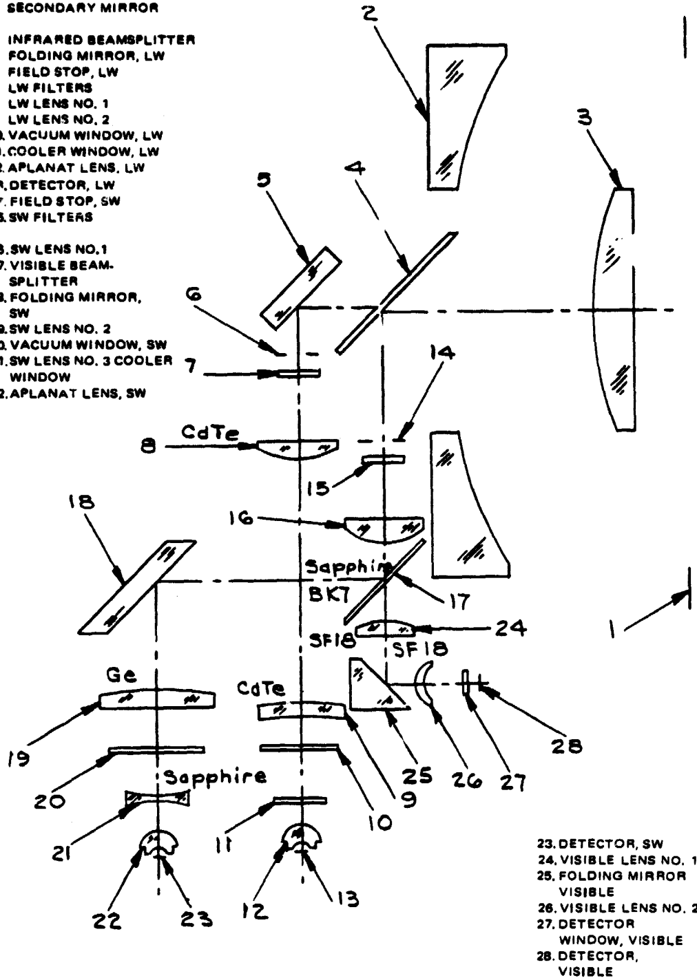
Figure 1-4. Optic Layout
