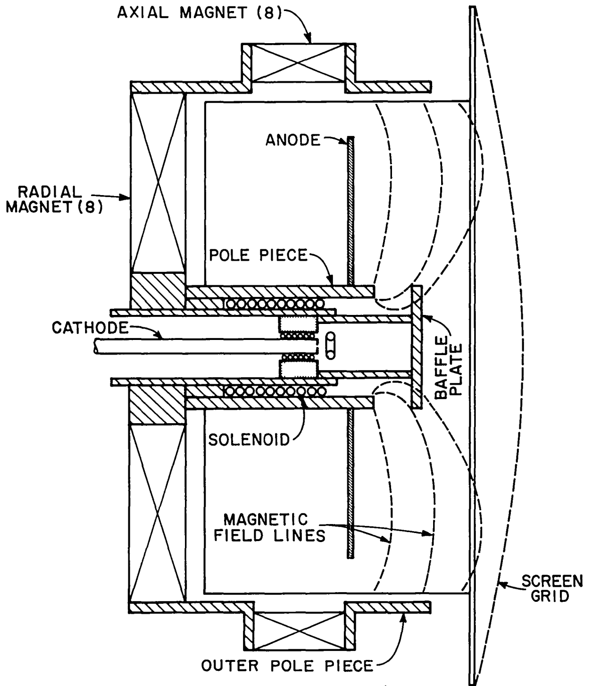
Fig. 7 Radial Field Thruster Equipped with Magnetic Baffle
