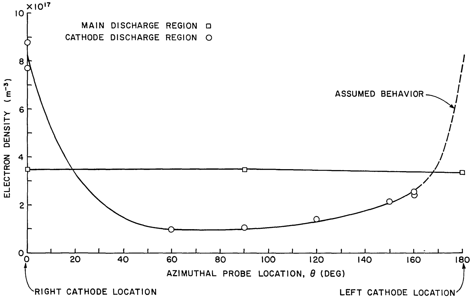
Fig. C-3 Aximuthal Plasma Variations
