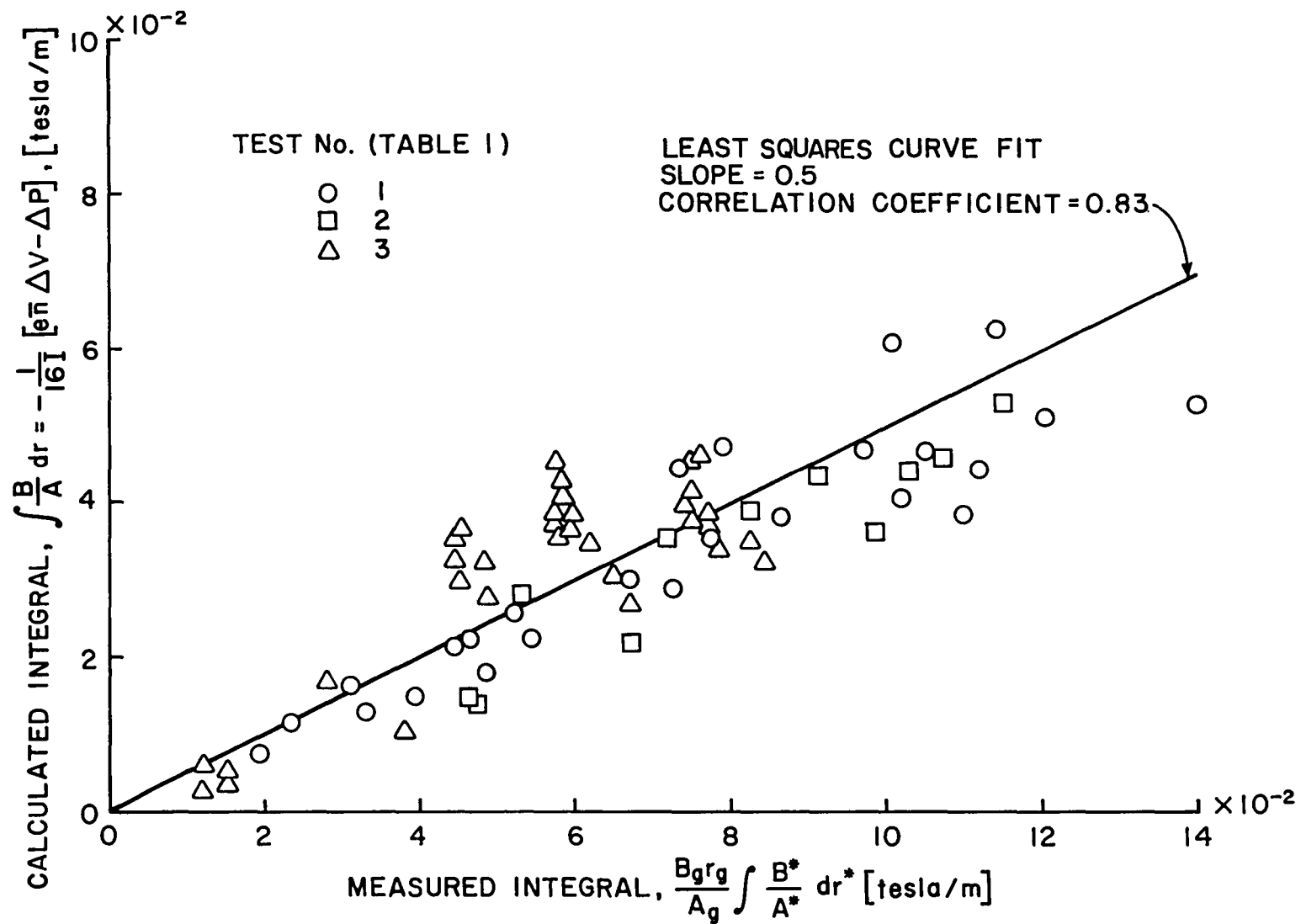
Fig. 11 Comparison of Calculated Integrals with the Measured Values for the Radial Field Thruster
