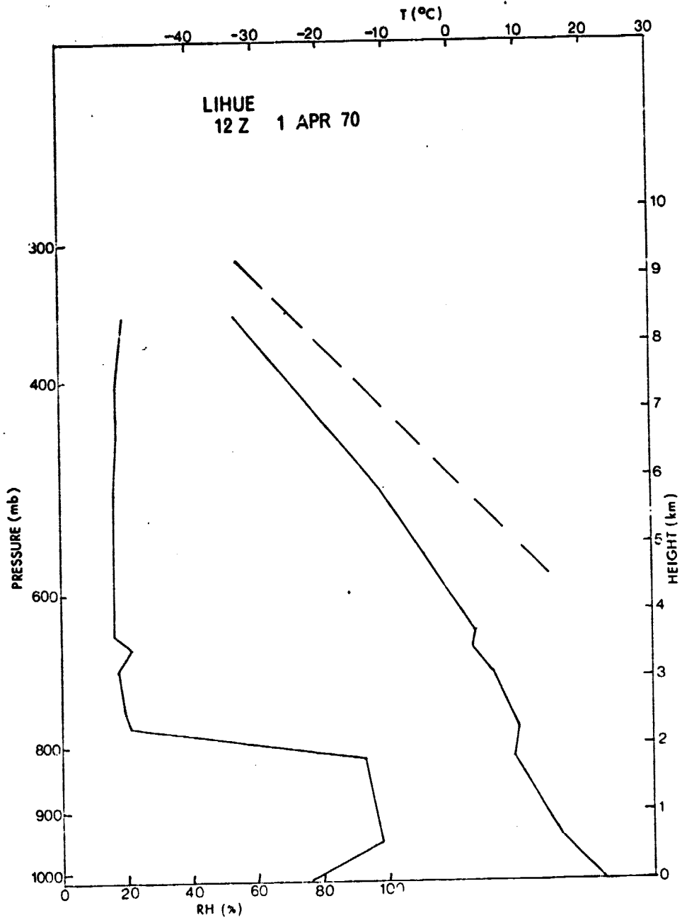
Fig. 2 Same as Fig. 1, but for 12Z ascent.
