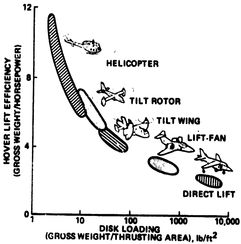
Figure 2. Hover efficiency.
