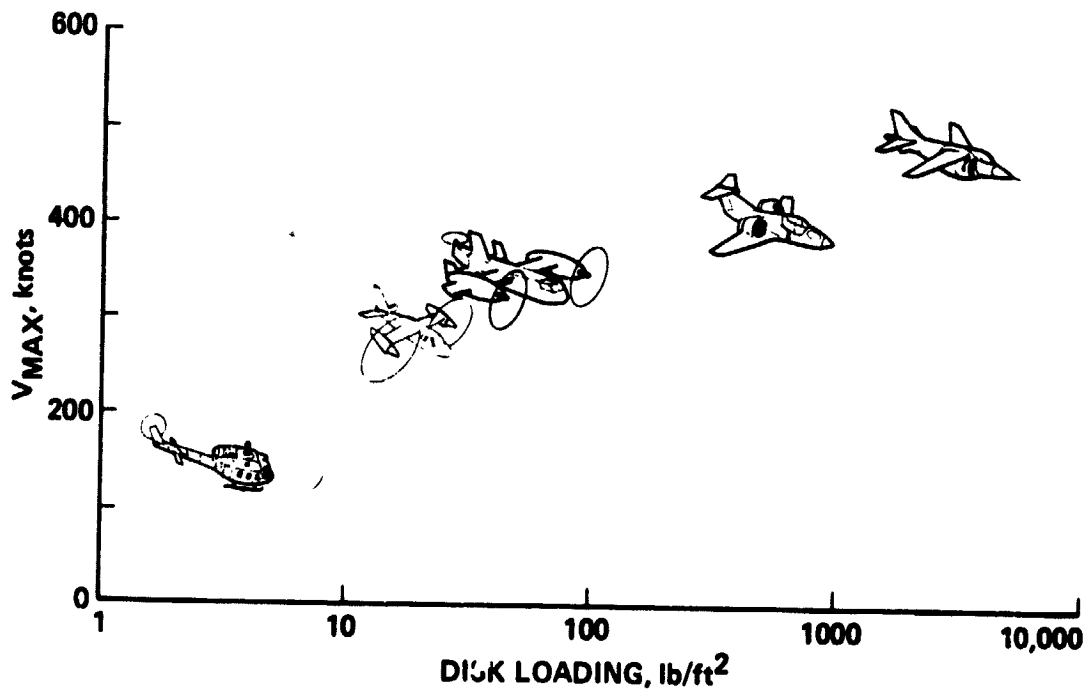
Figure 3. Cruise performance.
