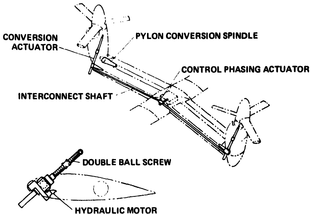
Figure 7. Conversion system.
