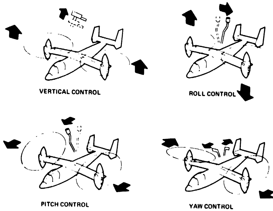
Figure 5. Control system.
