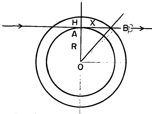
Figure 1. Geometry of extreme atmospheric path. The atmosphere is assumed homogeneous with a depth H = 8 \text{ km} and the mean radius of the earth R = 6378 \text{ km} . The extreme path in this approximation is 2x .
