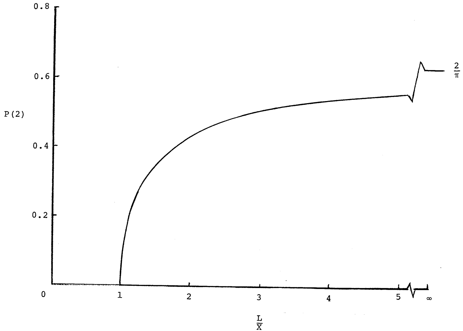
Figure 7.- Probability of one fiber intersecting both of two infinitely long conductors.
