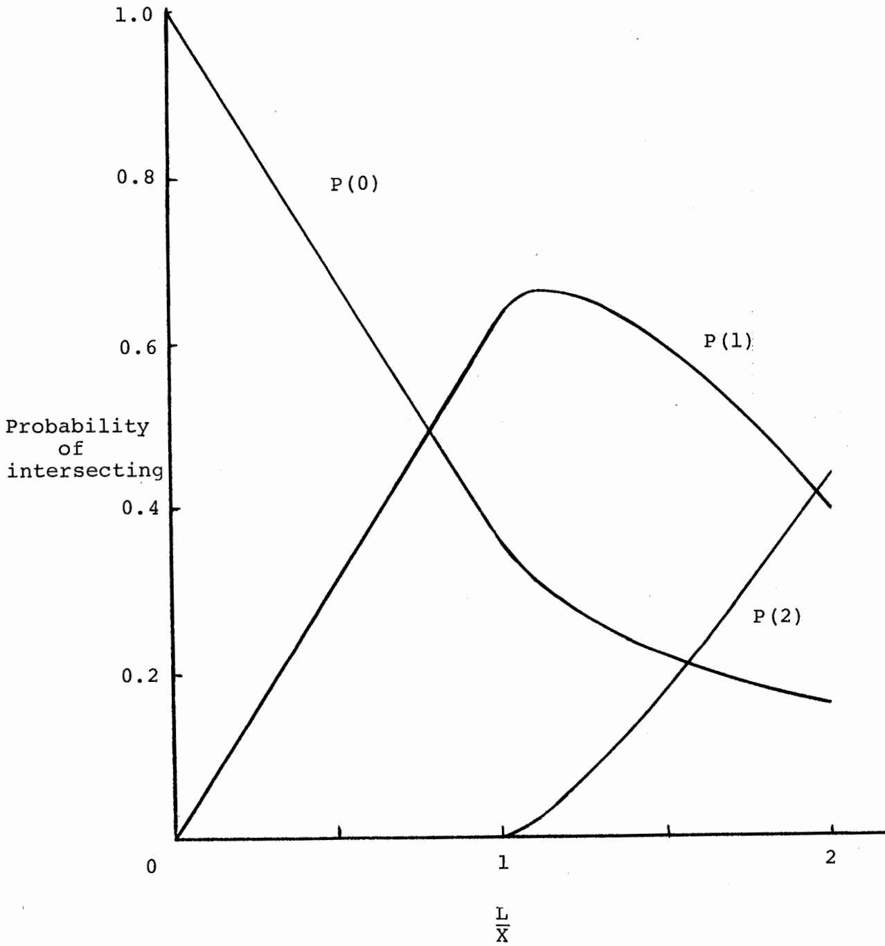
Figure 5.- Probability of a fiber intersecting none, one, or two of an infinite array of conductors.
