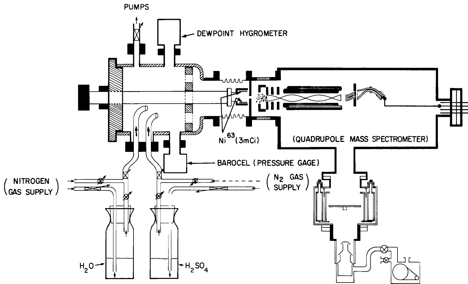
Figure 1.- Schematic diagram of experimental system used in study of ion-induced nucleation in ( \text{H}_2\text{O} + \text{H}_2\text{SO}_4 ) gas mixture.
