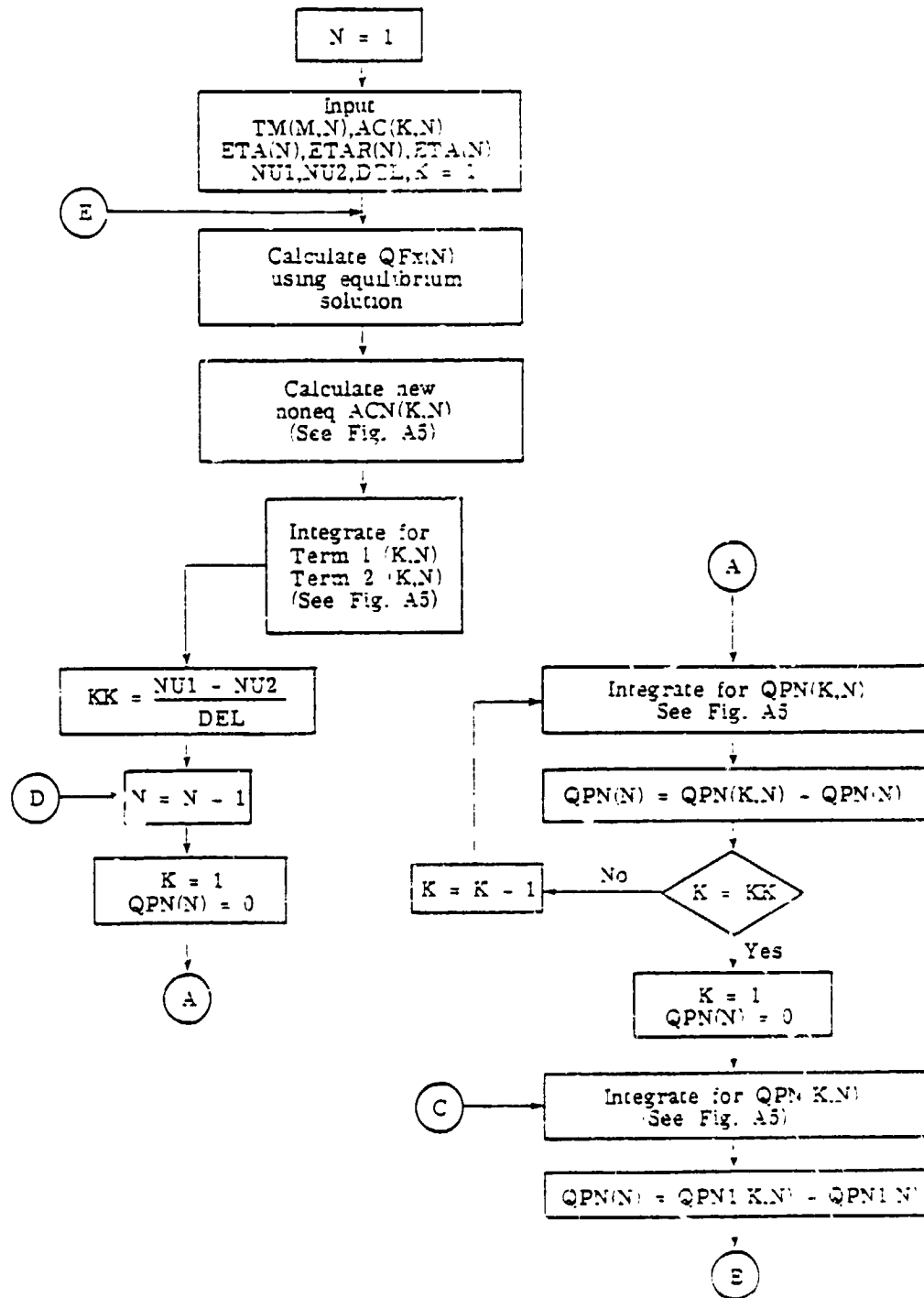
Figure A.4. Flow chart for subroutine NRAD.
