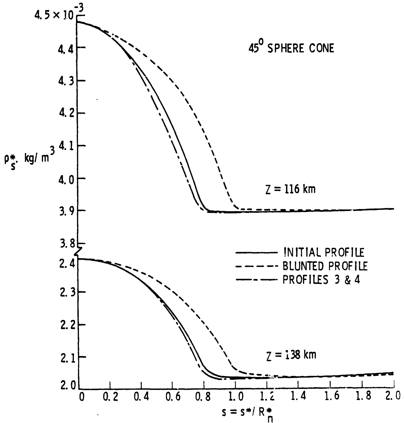
Figure 42. Variation of density just behind the shock for 45-degree sphere cone.
