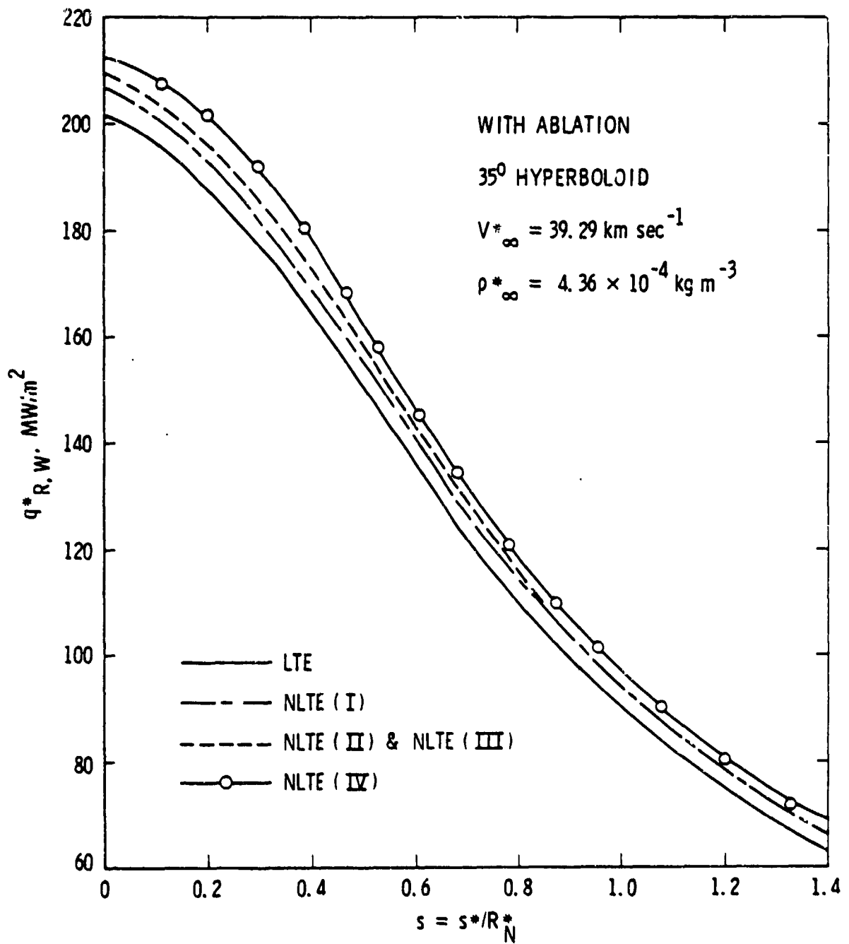
Figure 36(b). Comparison of LTE and NLTE radiative heating rates along the body surface with ablation.
