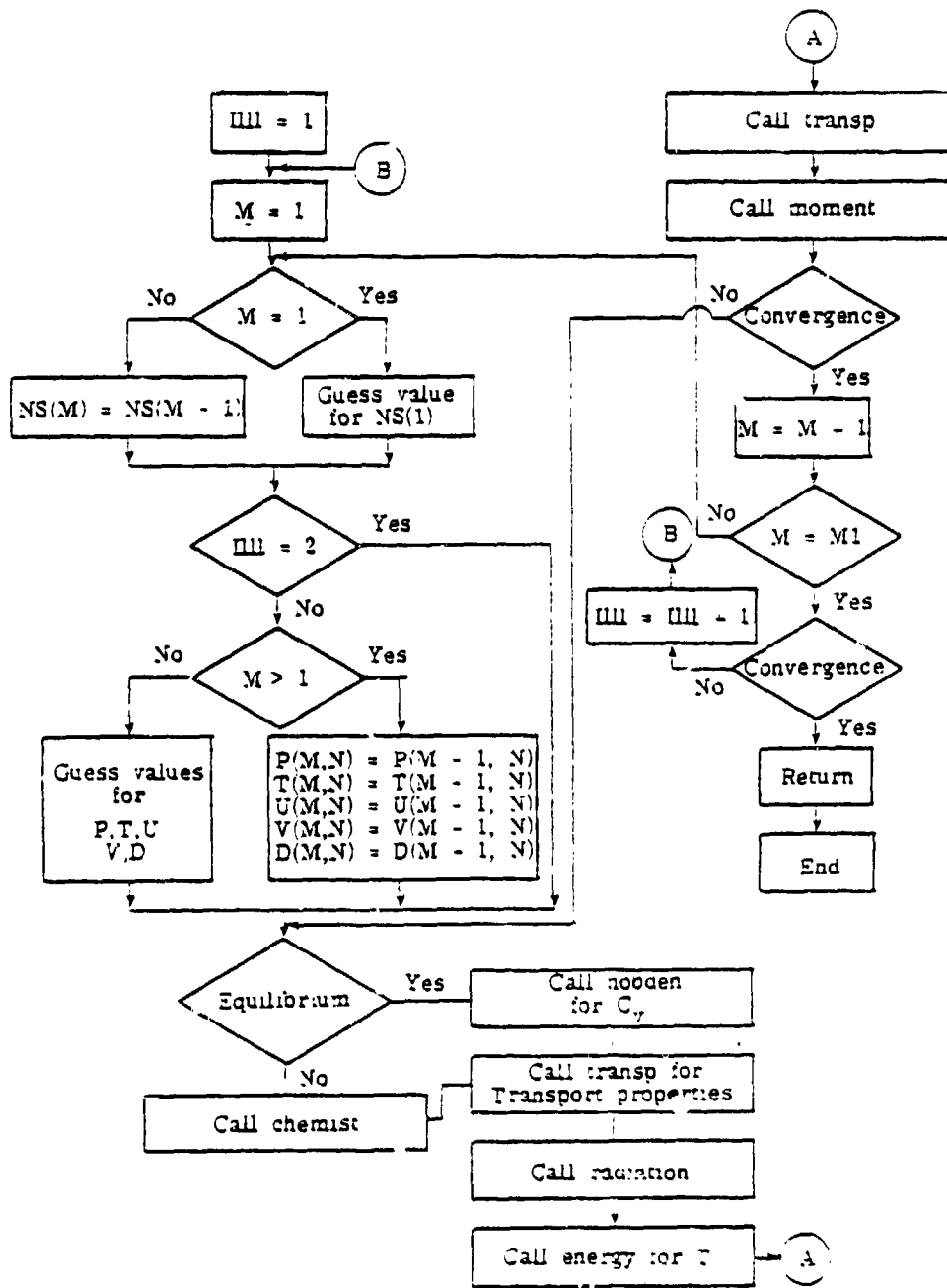
Figure A.3. Flow chart for subroutine SHOKLY for shock-layer solution.
