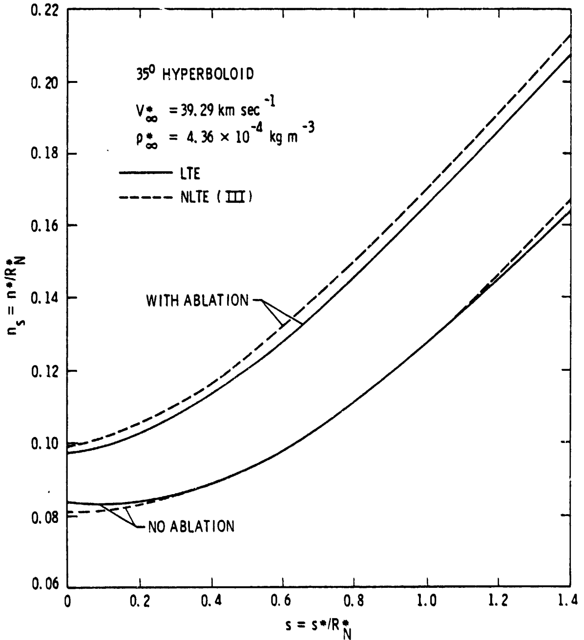
Figure 34. Shock standoff variation with distance along the body surface.
