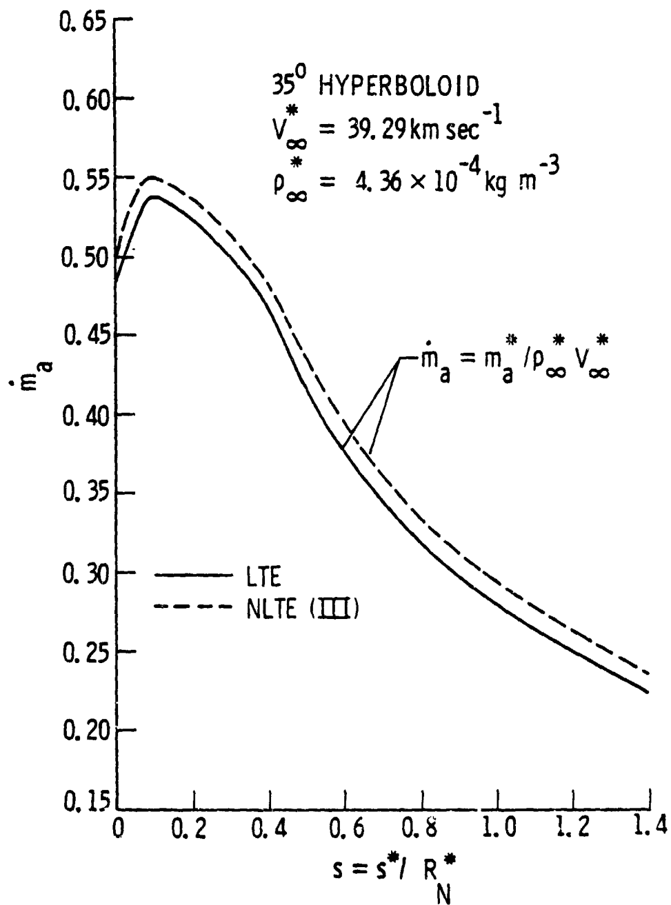
Figure 37. Ablation mass loss rate along the body surface.
