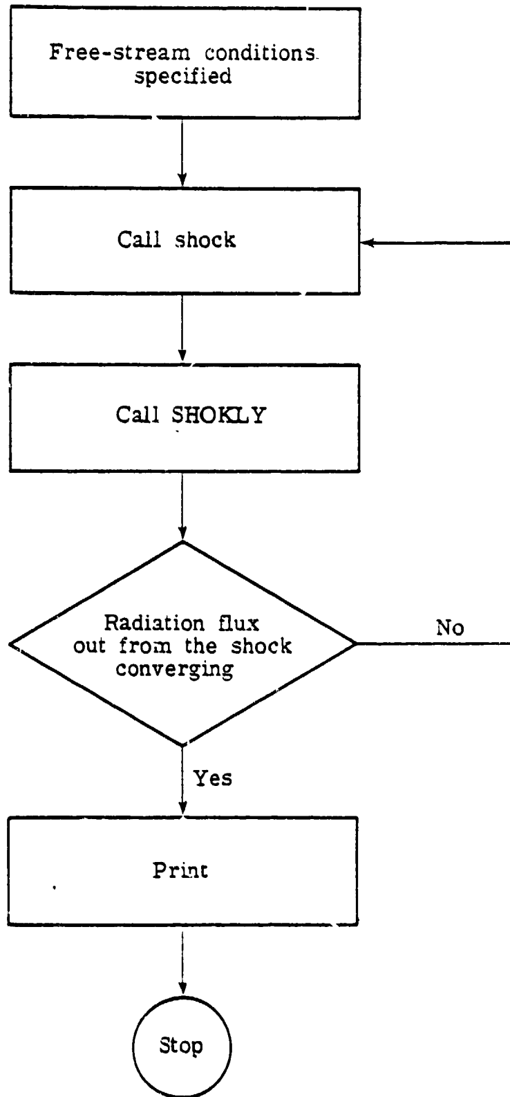
Figure A.2. Flow chart for shock layer solution procedure.
