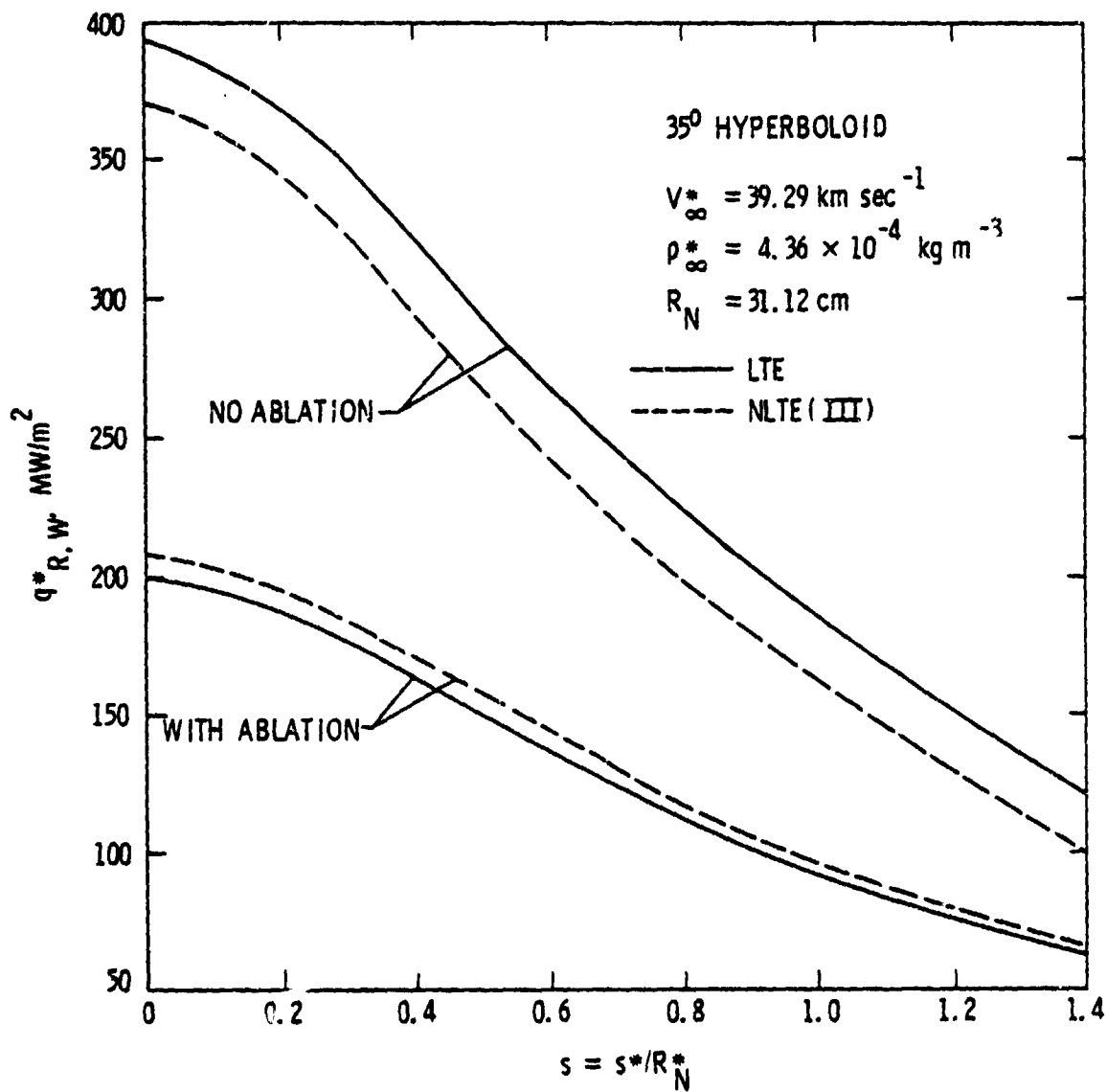
Figure 36(a). Variation of radiative heating rate along the body surface (with and without ablation).
