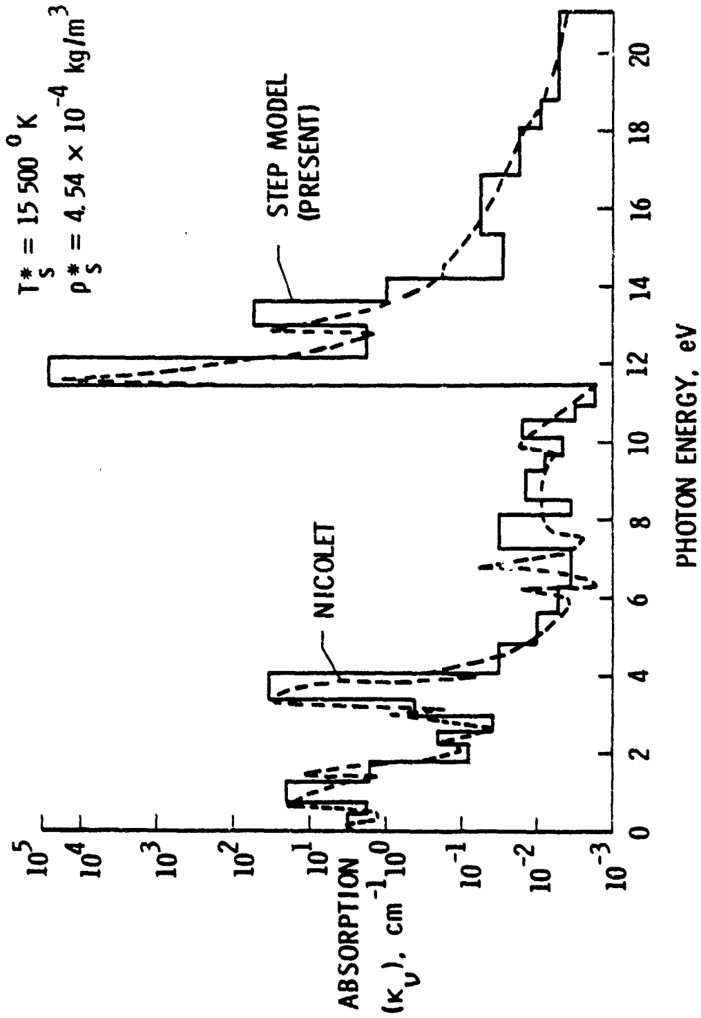
Figure 3. A 30-step model to approximate the absorption by Nicolet's detailed model ( T_S = 15,500\text{ K} ).
