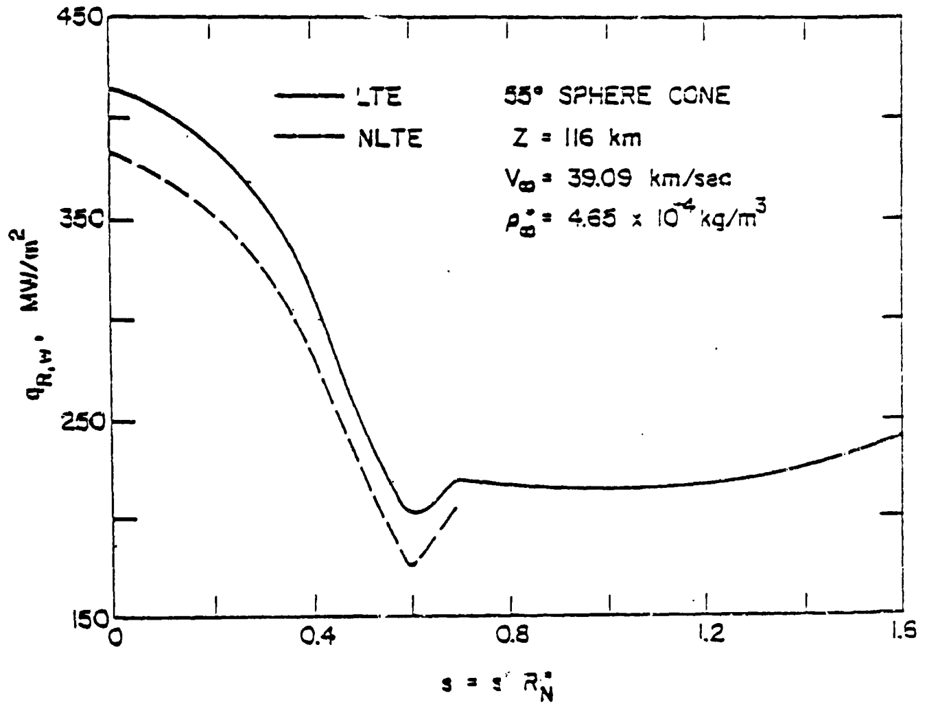
Figure 30. Radiative heating along the body (55° sphere cone) for entry conditions at Z = 116 km, H-H and H-H + collisions.
