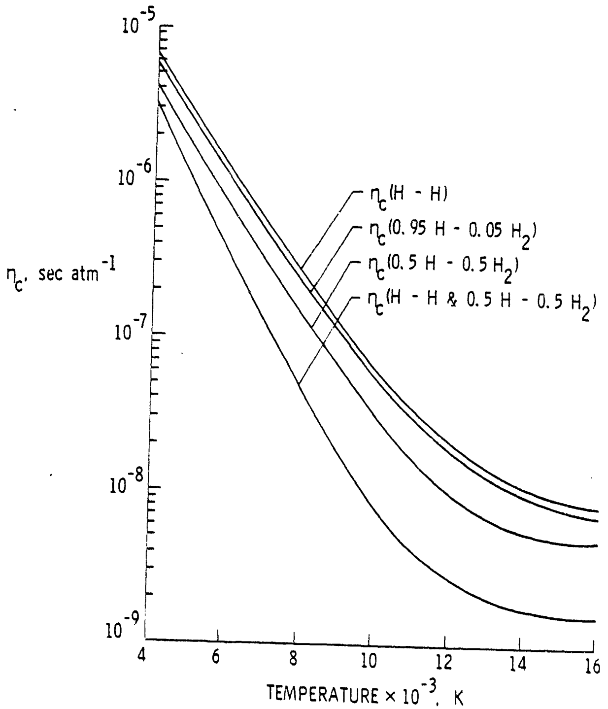
Figure 4. Collisional relaxation time for atomic and molecular hydrogen species.
