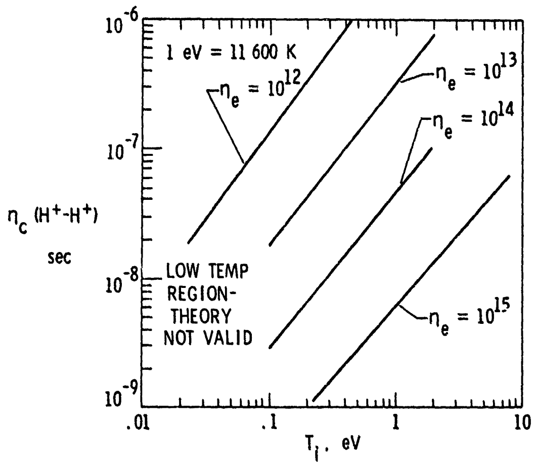
Figure 6. Collisional relaxation time for hydrogen ions.
