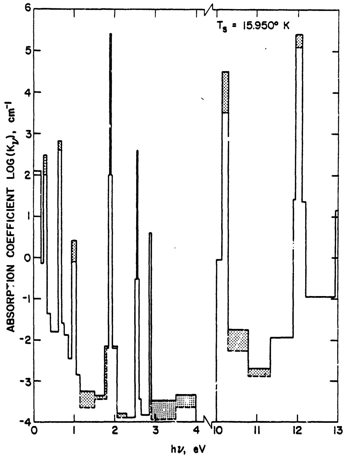
Figure 21. Equilibrium and nonequilibrium absorption coefficients for two-level energy transitions.
