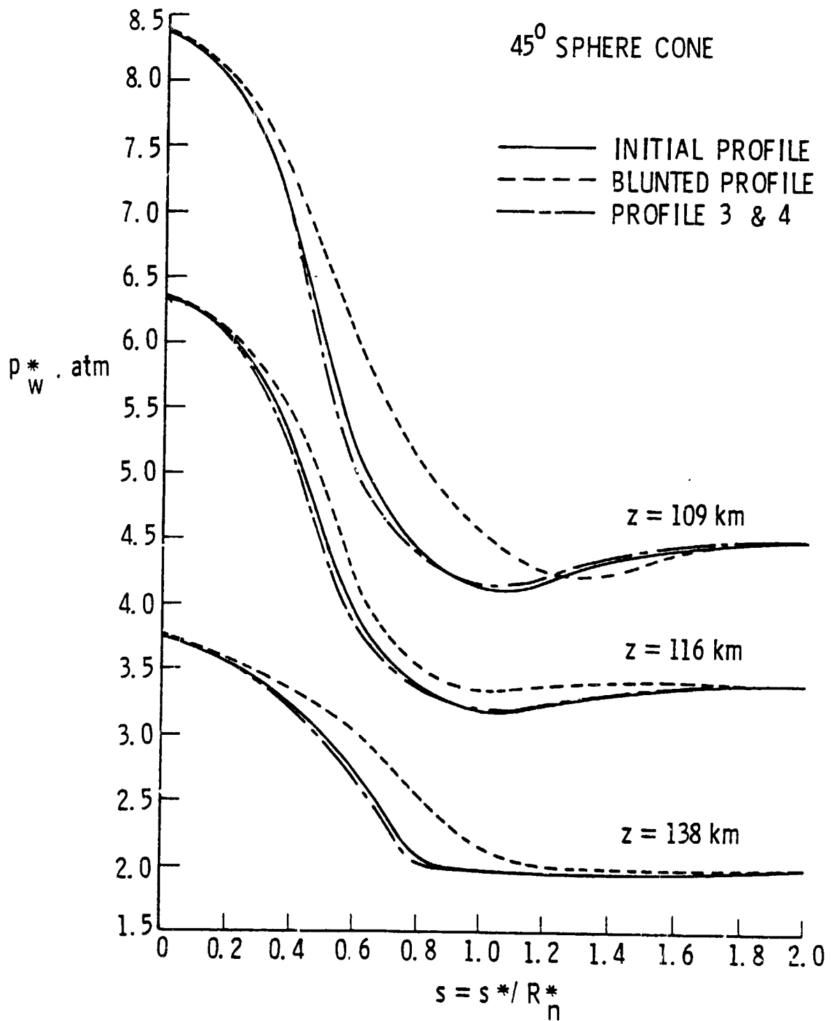
Figure 45. Surface pressure variation for 45-degree sphere cone.
