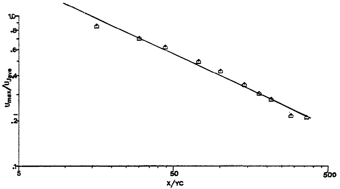
Fig. 5.8(a) Variation of U_{max}
