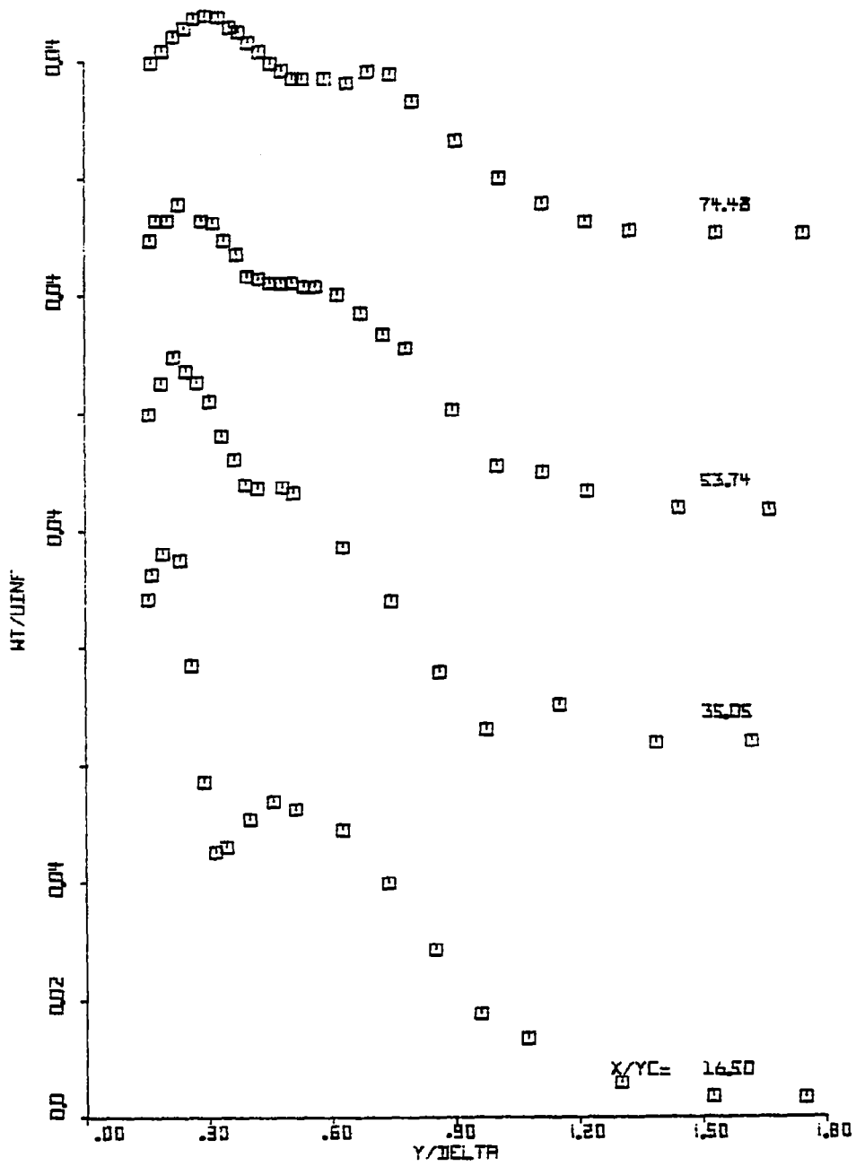
Fig. 4.12(a) Distribution of the Turbulence Intensity w_t/U_\infty at x/y_c = 16.5 to 74.48
