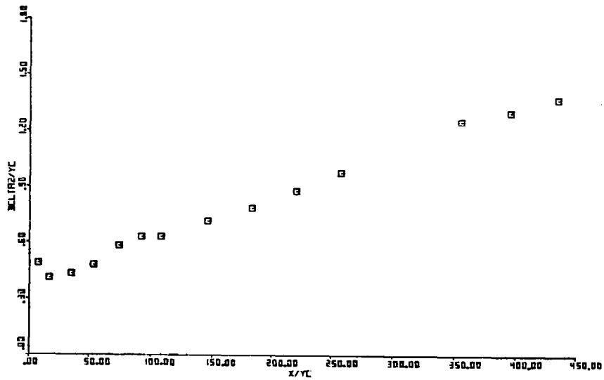
Fig. 4.6(c) Growth of the Momentum Thickness
