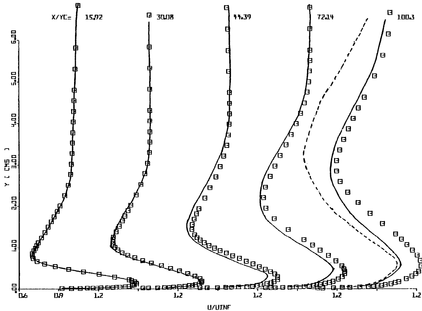
Fig. 5.4(b) Mean Velocity Profiles at x/y_c = 15.92 to 100.3
