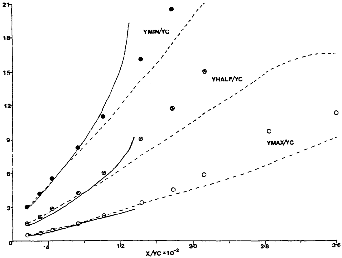
Fig. 7.2(h) Predicted Development of the Profile Length Scales for the Adverse Pressure Gradient Flow
