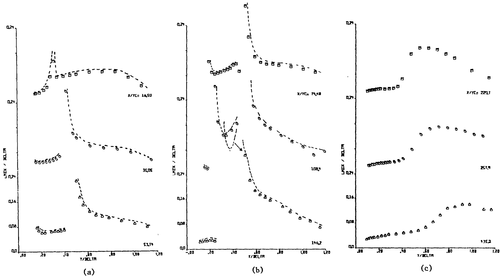
Fig. 4.18 Distributions of the Prandtl Mixing Length L_{mix}
