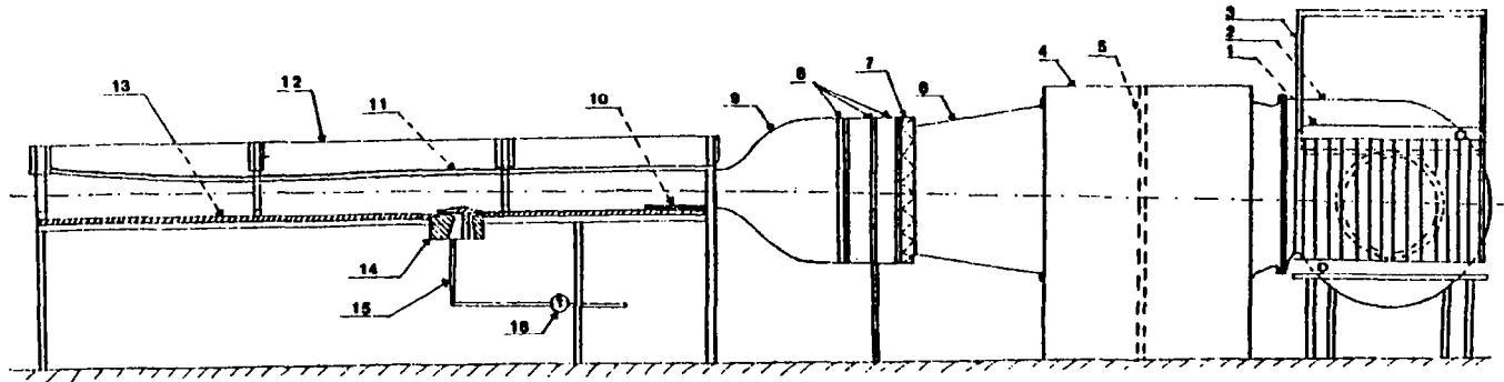
Fig. 2.1 Schematic Arrangement of the Wind Tunnel
