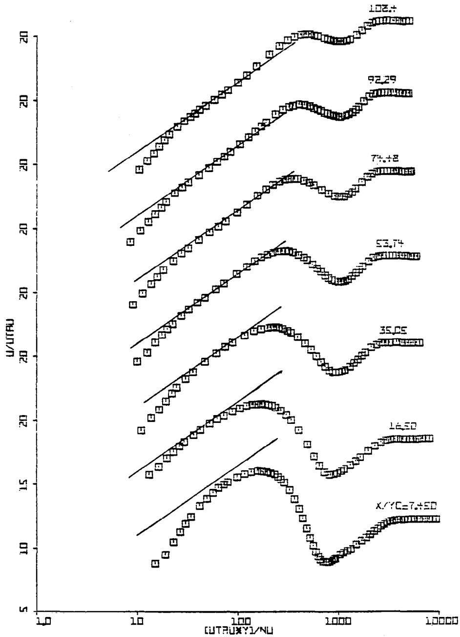
Fig. 4.5(a) Mean Velocity Profiles in the Wall Coordinates at x/y_c = 7.45 to 108.4
