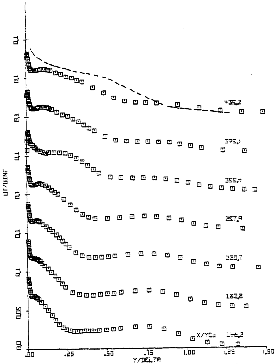
Fig. 4.9(c) Distribution of the Turbulence Intensity u_t/U_{\infty} at x/y_c = 146.2 to 435.2
