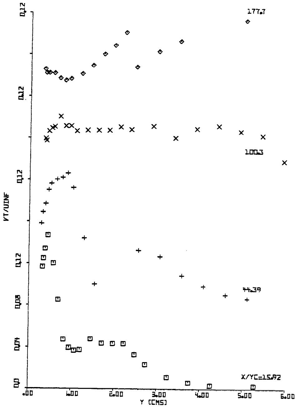
Fig. 5.11 Distributions of the Turbulence Intensity v_t/U_\infty
