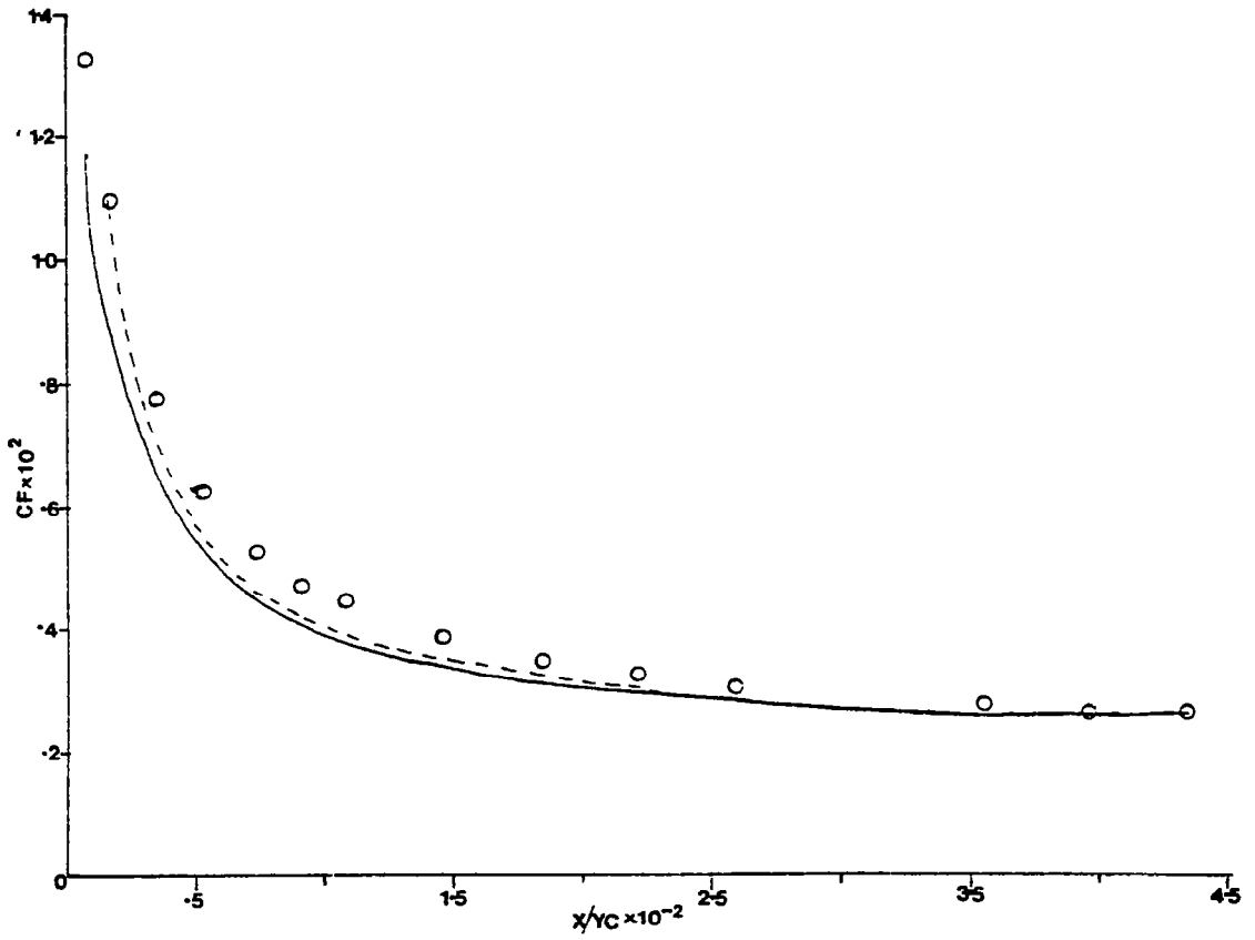
Fig. 7.1(d) Predicted Variation of the Skin Friction for the Zero Pressure Gradient Flow
