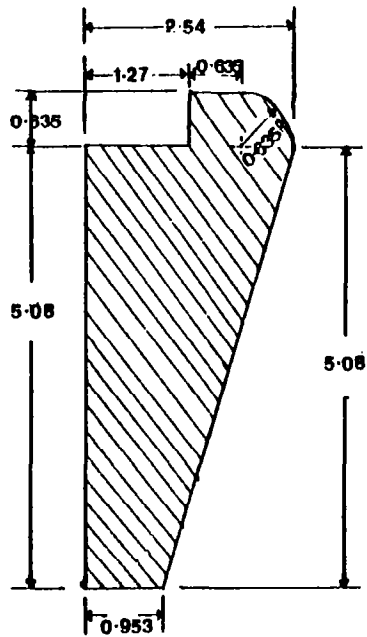
Fig. 2.6 Poplar Wood Section "A" (Fig. 2.5) (All dimensions are in cm.)
