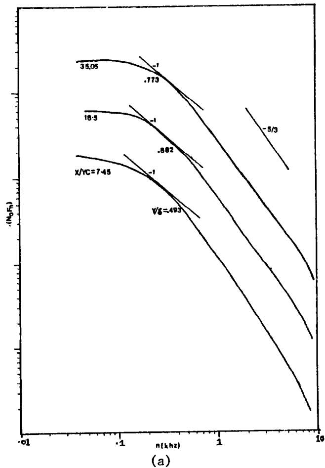
Fig. 4.23 Spectra of u^2 Representing the Outer Layer at Different Stations
