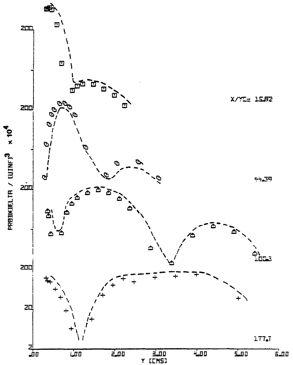
Fig. 5.20 Distributions of the Shear Stress Production of Turbulent Kinetic Energy
