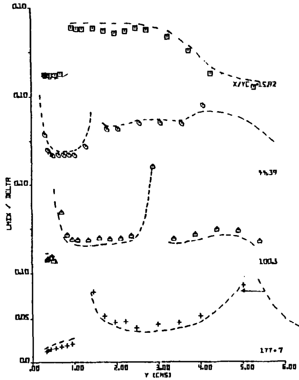
Fig. 5.18 Distributions of the Prandtl Mixing Length L_{mix}
