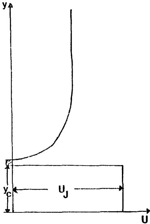
Fig. 1.2(a) Uniform Jet Velocity Profile
