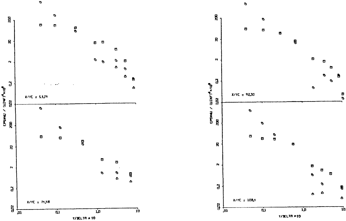
Fig. 4.24(b) Distributions of the Dissipation Rate at x/y_c = 53.74 to 108.4
