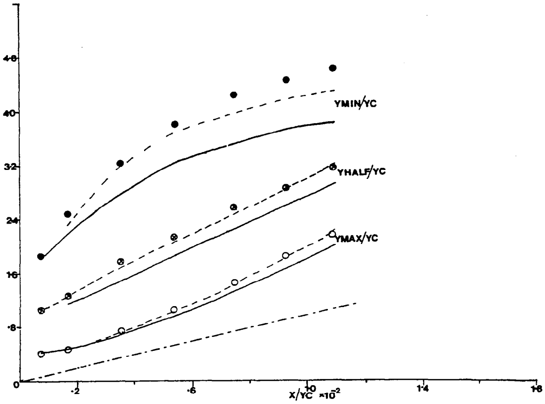
Fig.7.1(e) Predicted Variation of the Profile Length Scales for the Zero Pressure Gradient Flow
