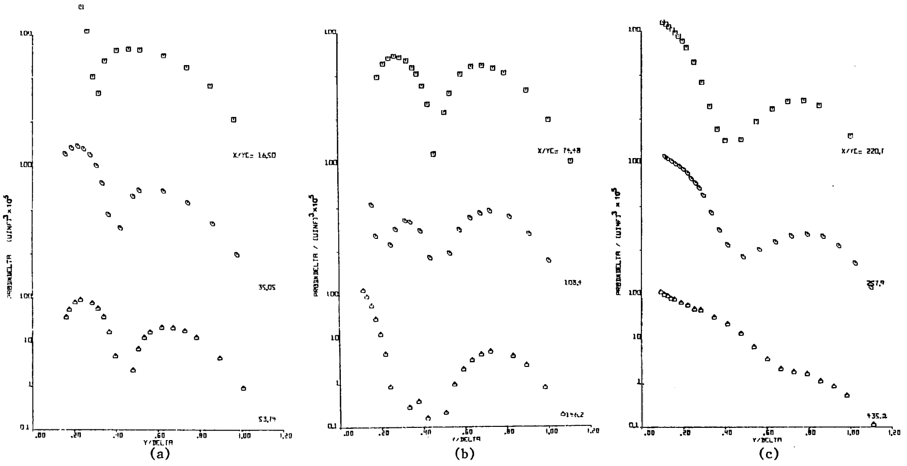
Fig. 4.20 Distributions of the Shear Stress Production of Turbulent Kinetic Energy
