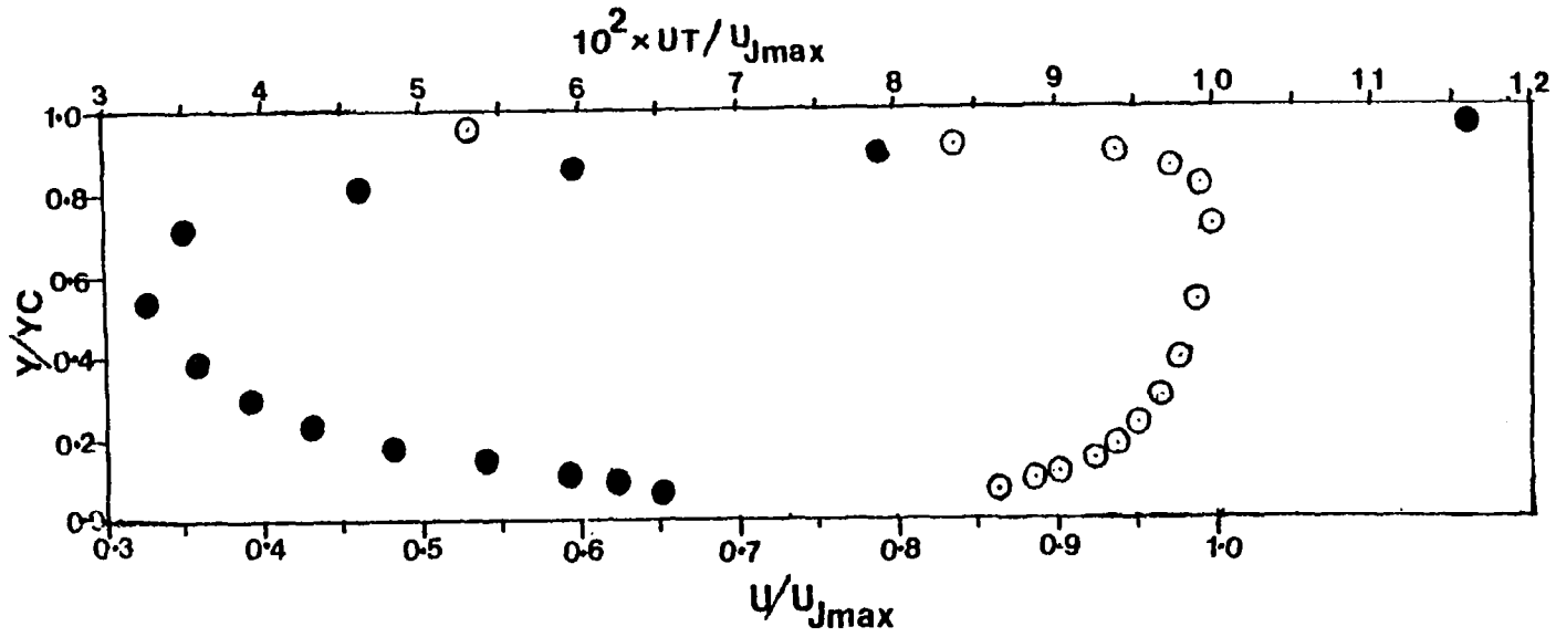
Fig. 2.11 Measured Velocity and Turbulence Profiles at the Slot ( x/y_c = 0.292 )
