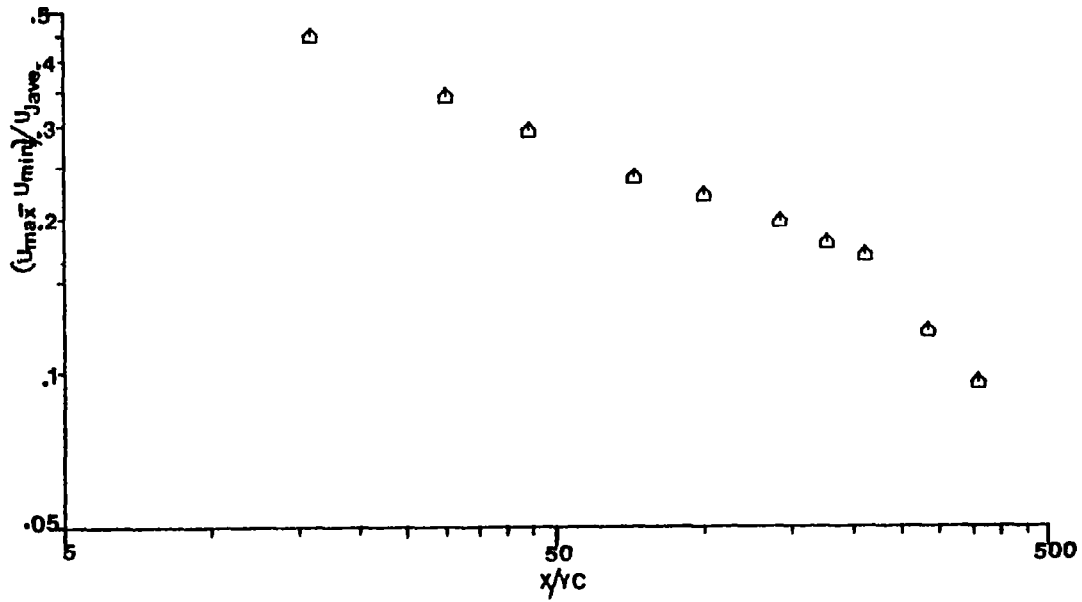
Fig. 5.8(c) Variation of (U_{\max} - U_{\min})
