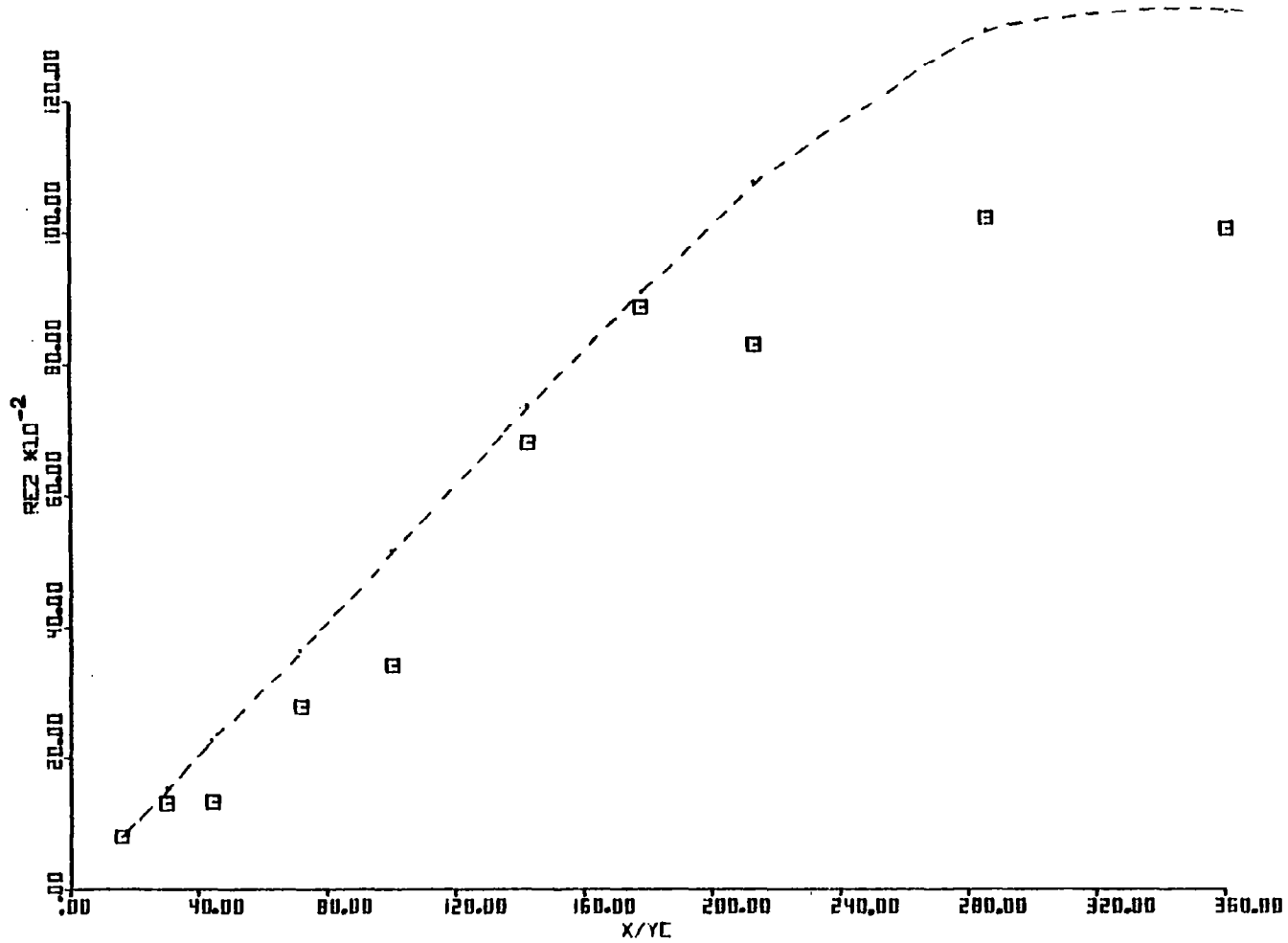
Fig. 5.6(e) Variation of the Momentum Thickness Reynolds Number Re_2
