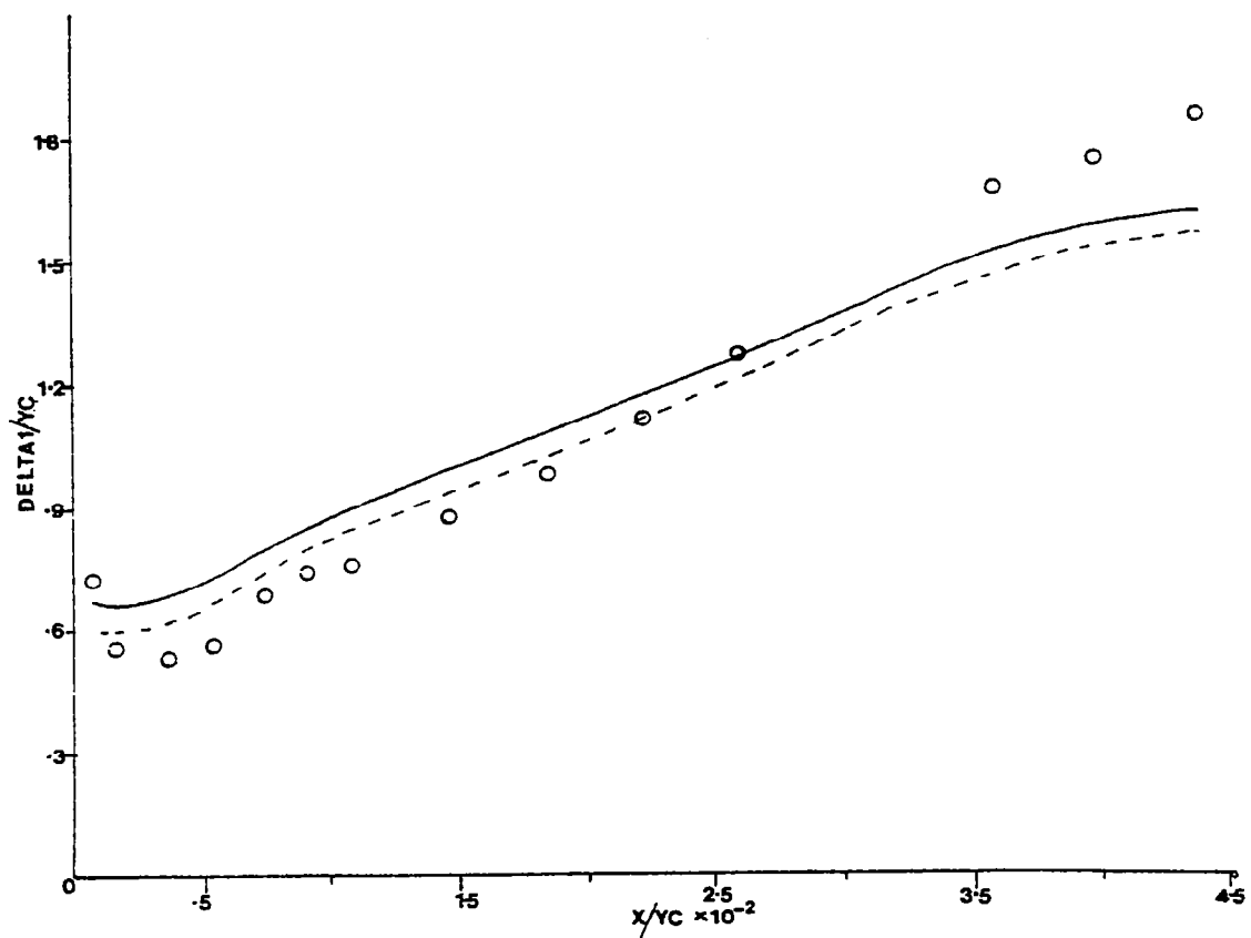
Fig. 7.1(b) Predicted Development of the Displacement Thickness for the Zero Pressure Gradient Flow
