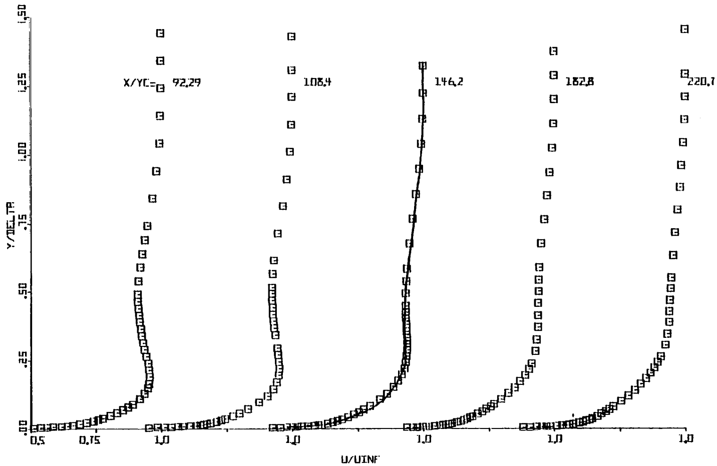
Fig. 4.4(d) Mean Velocity Profiles at x/y_c = 92.29 to 220.7
