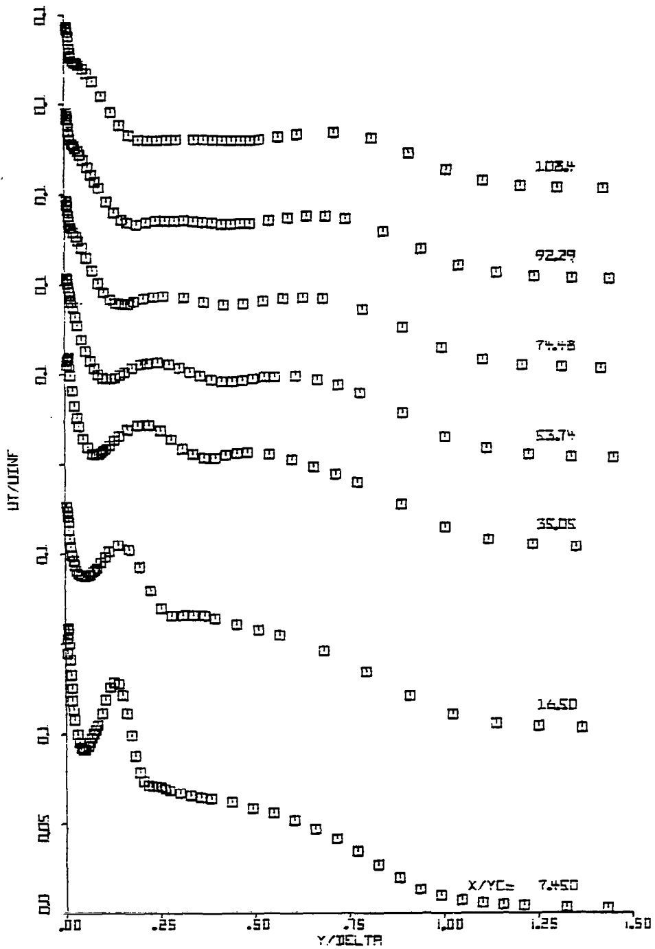
Fig. 4.9(b) Distribution of the Turbulence Intensity u_t/U_\infty at x/y_c = 7.45 to 108.4
