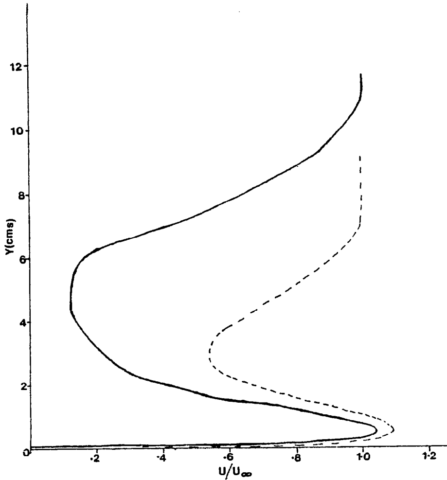
Fig. 7.4(a) Predicted Velocity Profiles at x/y_c = 100.3 for the Adverse Pressure Gradient c Flow
