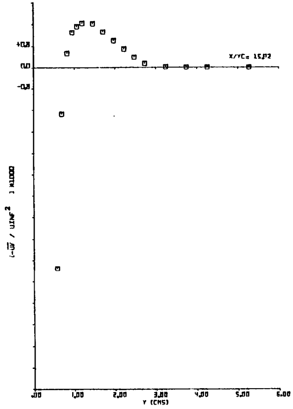
Fig. 5.13(a) Distribution of the Shear Stress at x/y_c = 15.92 and 44.39
