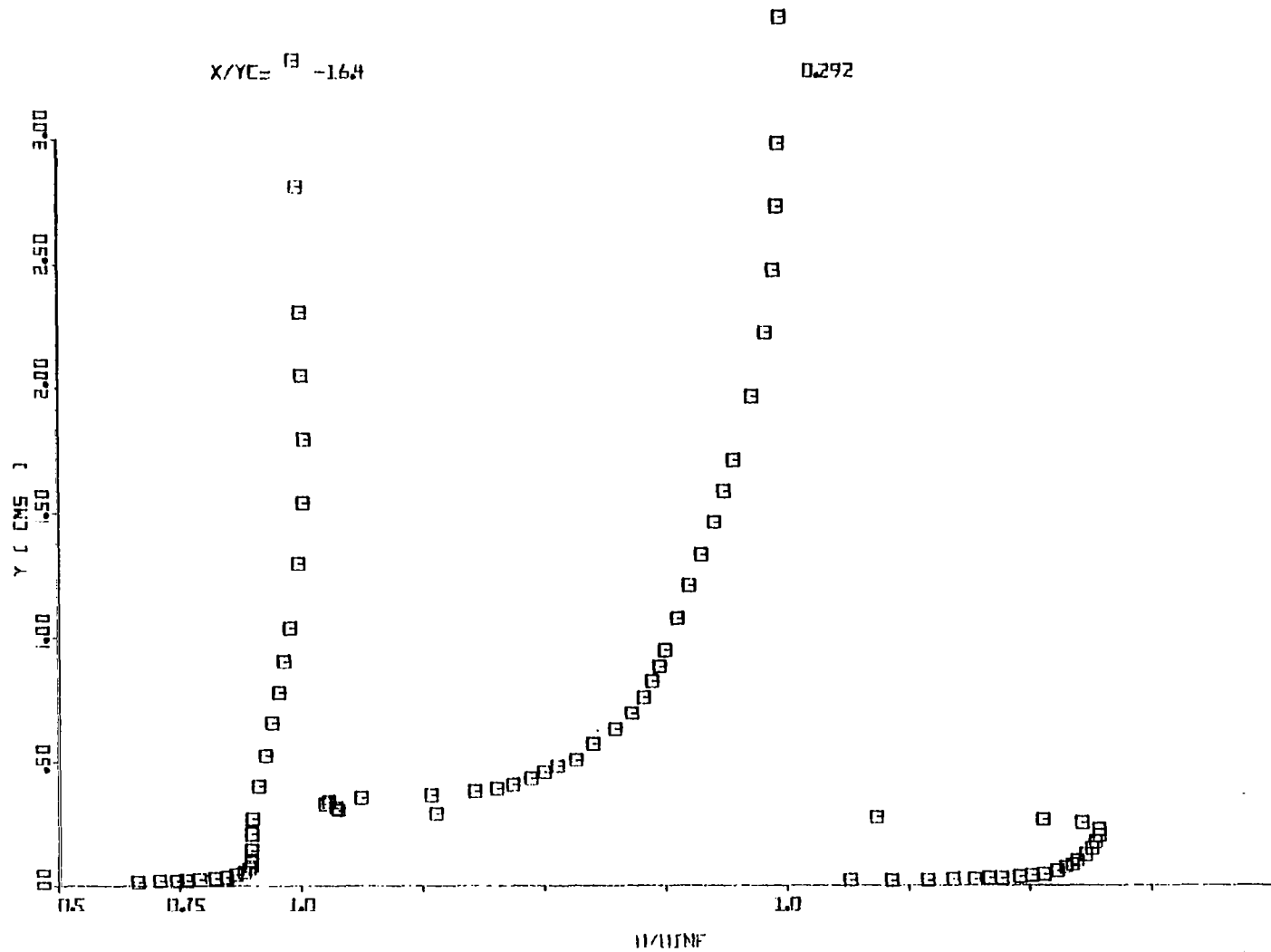
Fig. 5.4(a) Mean Velocity Profiles Upstream of the Slot ( x/y_c = -16.4 ) and at the Slot ( x/y_c = 0.292 )
