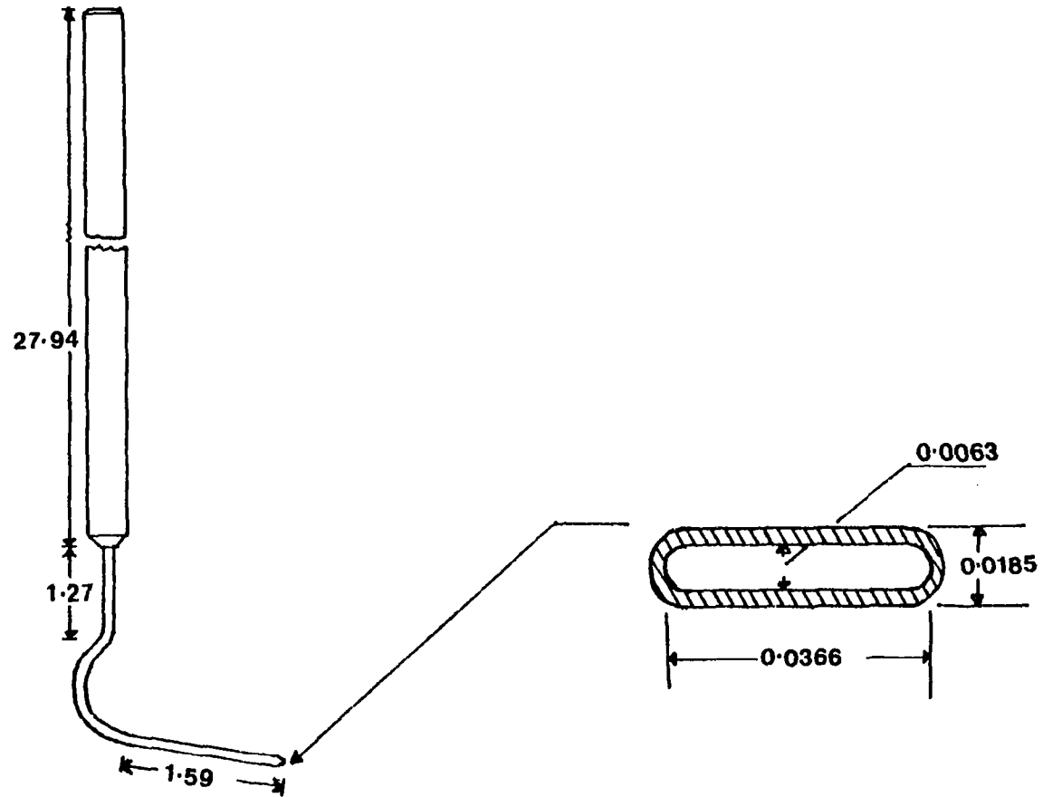
Fig. 3.1 Rectangular Mouth Boundary Layer Pilot (total head) Tube (All dimensions are in cm.)
