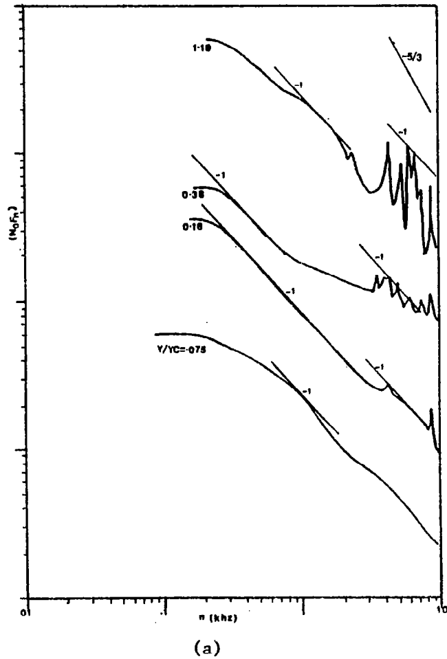
Fig. 4.21 Spectra of u^2 at x/y_c = 0.292 and at Different y/y_c Locations
