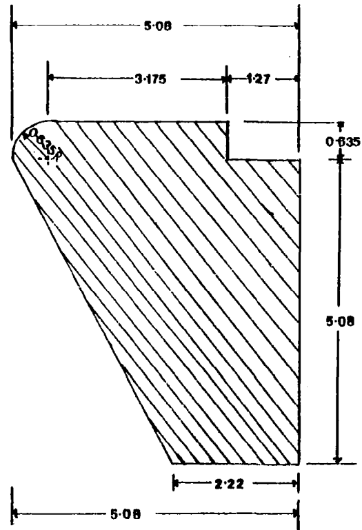
Fig. 2.7 Poplar Wood Section "B" (Fig. 2.5) (All dimensions are in cm.)
