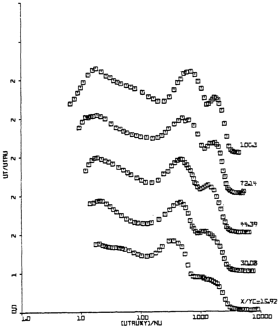
Fig. 5.10(a) Distribution of u^+ in Wall Coordinates at x/y_c = 15.92 to 100.3
