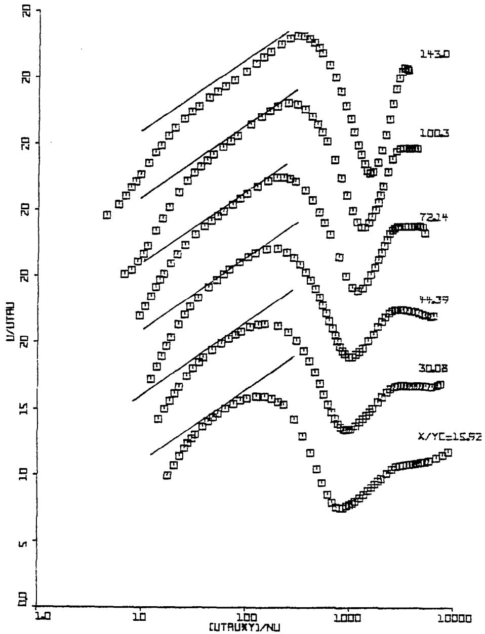
Fig. 5.5(a) Mean Velocity Profiles in the Wall Coordinates at x/y_c = 15.92 to 143.0
