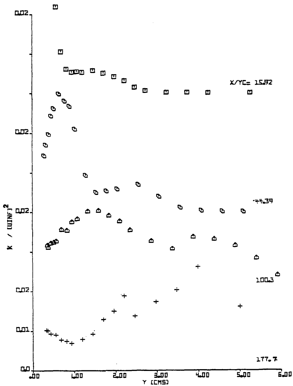
Fig. 5.14 Variation of the Turbulent Kinetic Energy k
