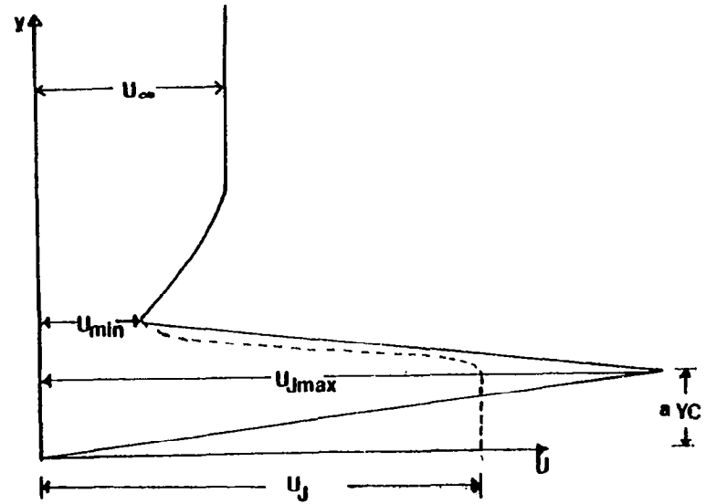
Fig. 7.3(b) Starting Velocity Profile for the Predictions with Linear Jet Velocity Profile using the Automatic Starting Procedure
