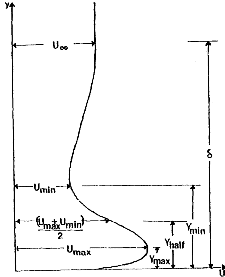
Fig. 1.1(b) Velocity Profile for a Blown Boundary Layer
