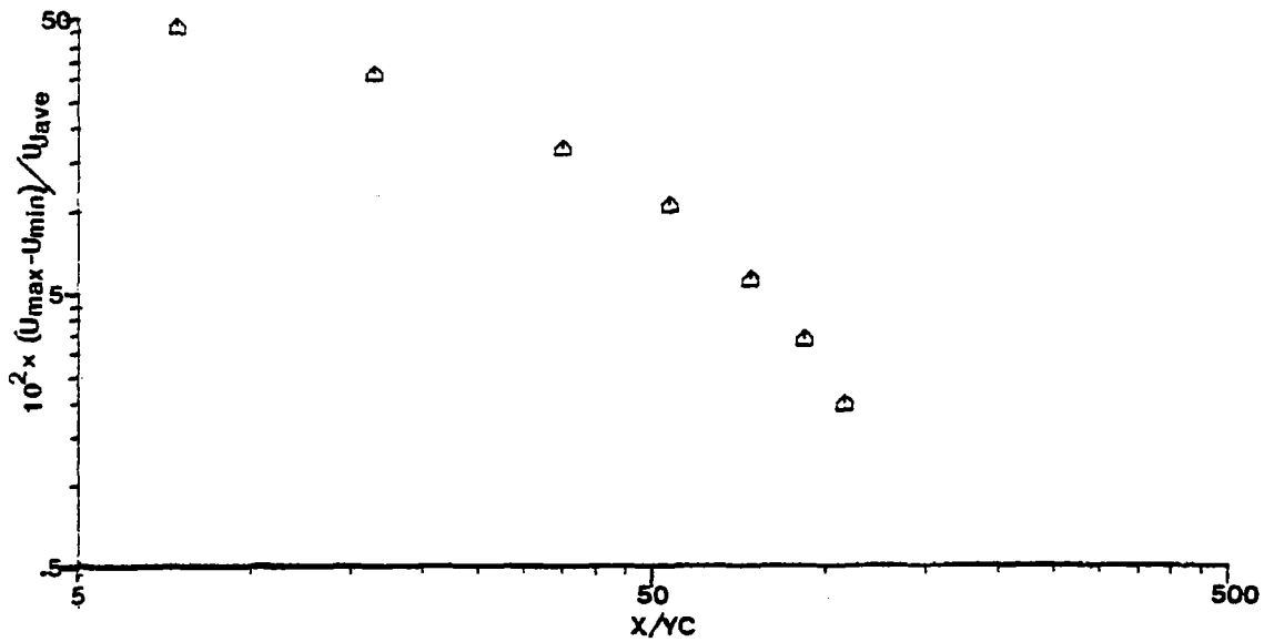
Fig. 4.8(b) Variation of (U_{max} - U_{min})
