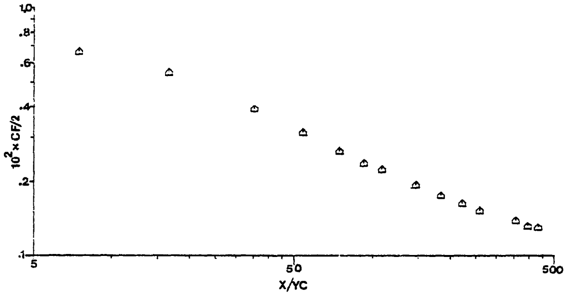
Fig. 4.3(b) Variation of Skin Friction in Logarithmic Coordinates
