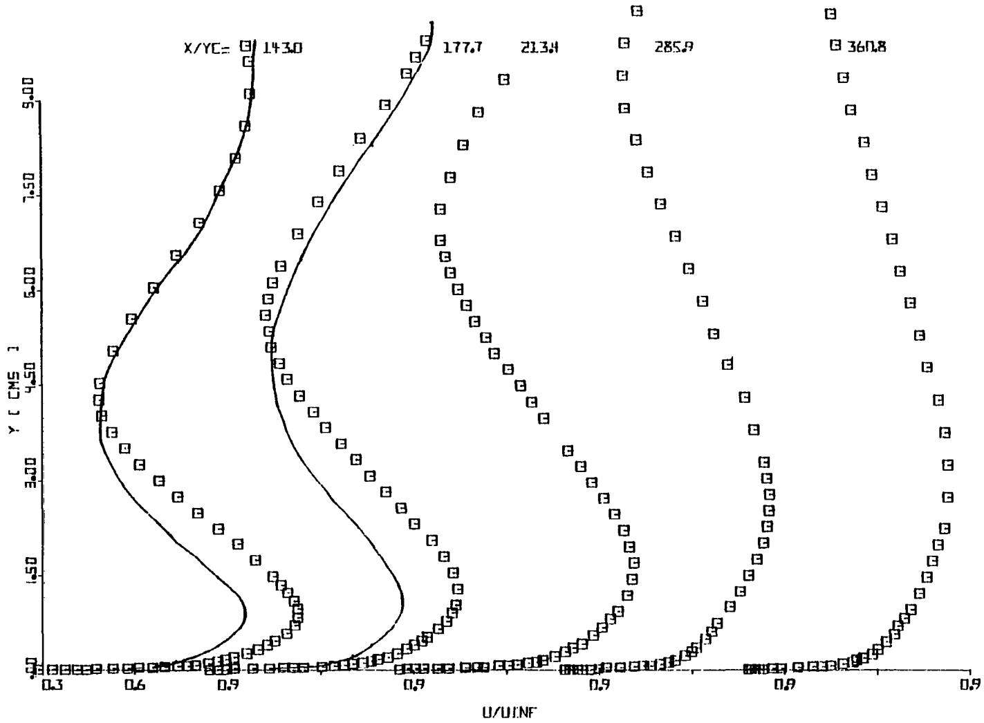
Fig. 5.4(c) Mean Velocity Profiles at x/y_c = 143.0 to 360.8
