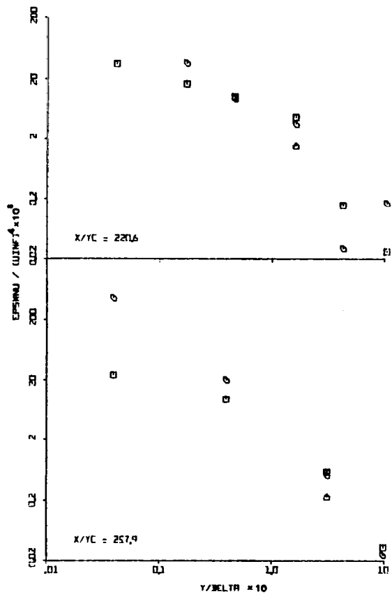
Fig. 4.24(c) Distribution of the Dissipation Rate at x/y_c = 146.2 to 257.9
