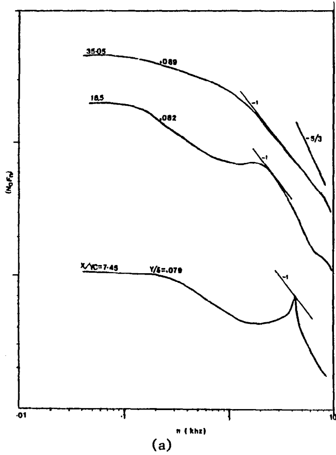
Fig. 4.22 Spectra of \overline{u^2} Representing the Inner Layer at Different Stations
