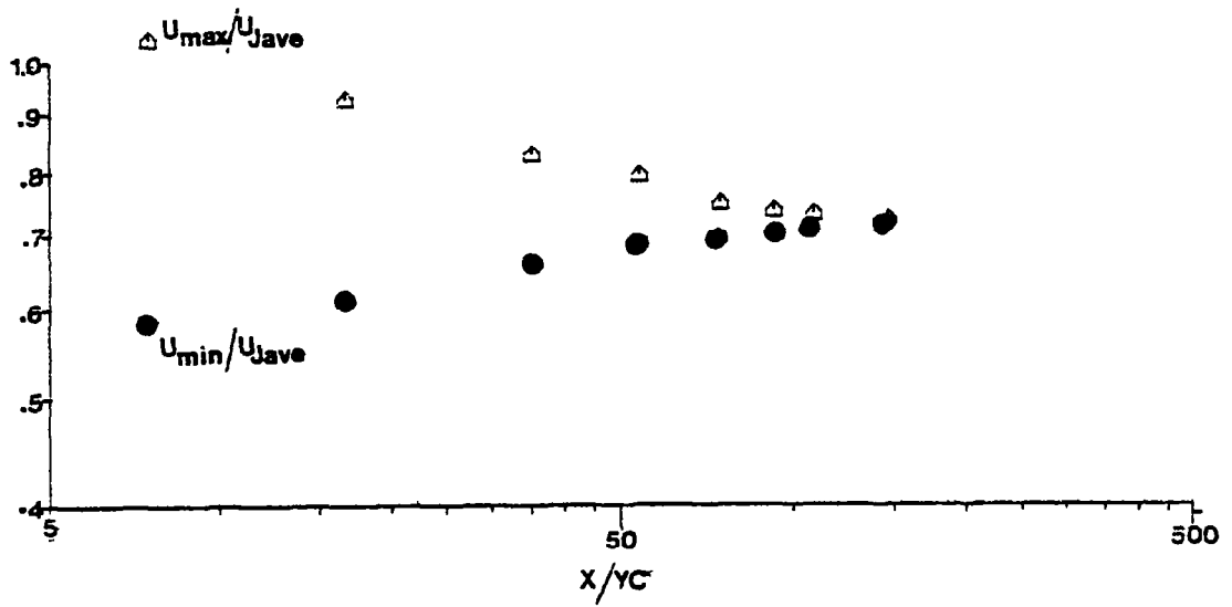
Fig. 4.8(a) Variation of U_{max} and U_{min}
