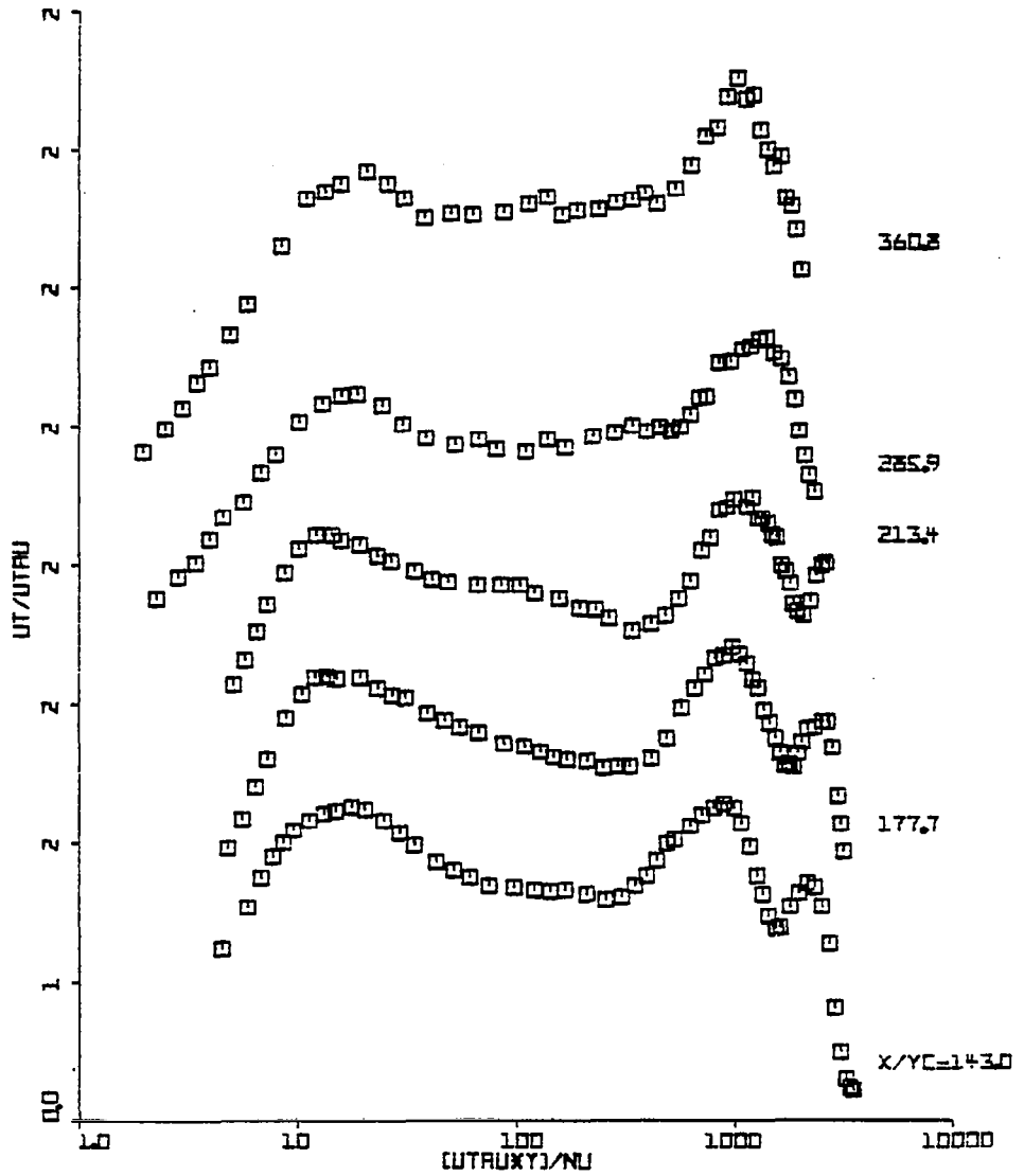
Fig. 5.10(b) Distribution of u^+ in Wall Coordinates at x/y_c = 143.0 to 360.8
