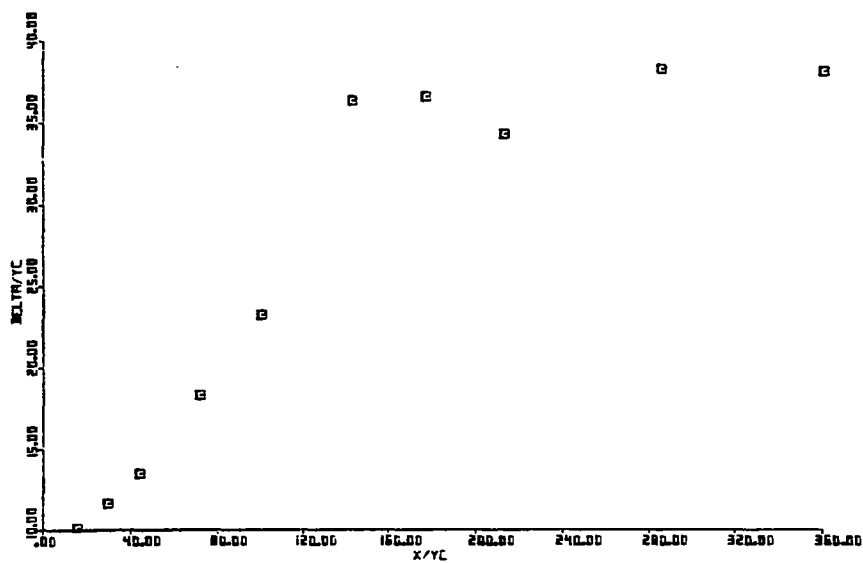
Fig. 5.6(a) Growth of the Boundary Layer Thickness
