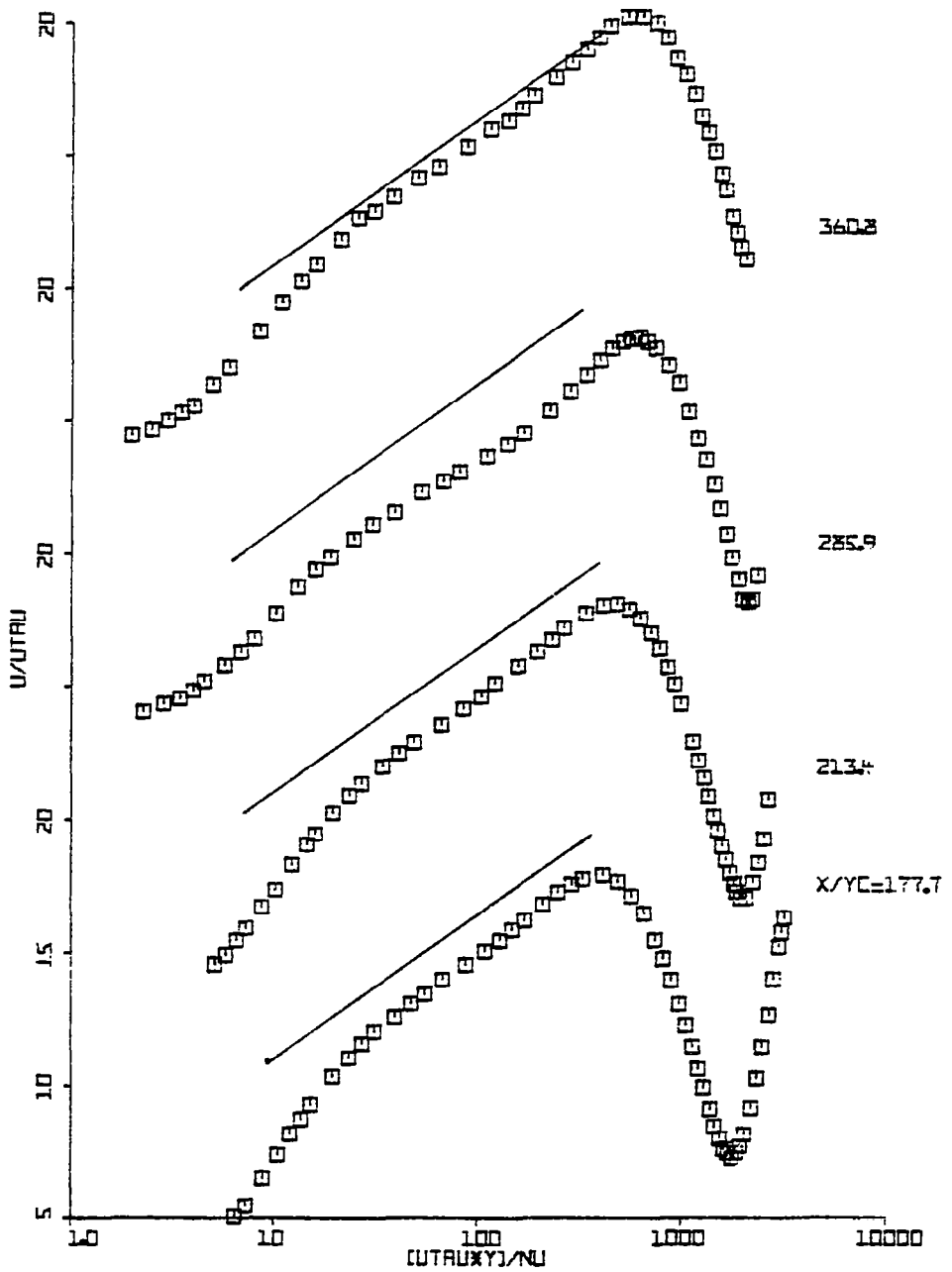
Fig. 5.5(b) Mean Velocity Profiles in the Wall Coordinates at x/y_c = 177.7 to 360.8
