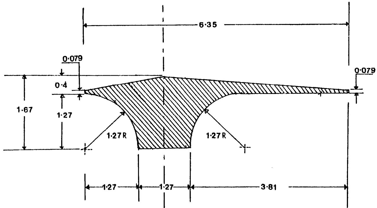
Fig. 2.8 Extruded Aluminum End Piece (All dimensions are in cm.)
