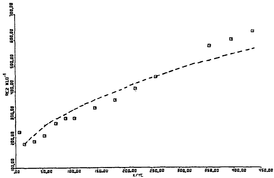
Fig. 4.6(e) Variation of the Momentum Thickness Reynolds Number Re_2
