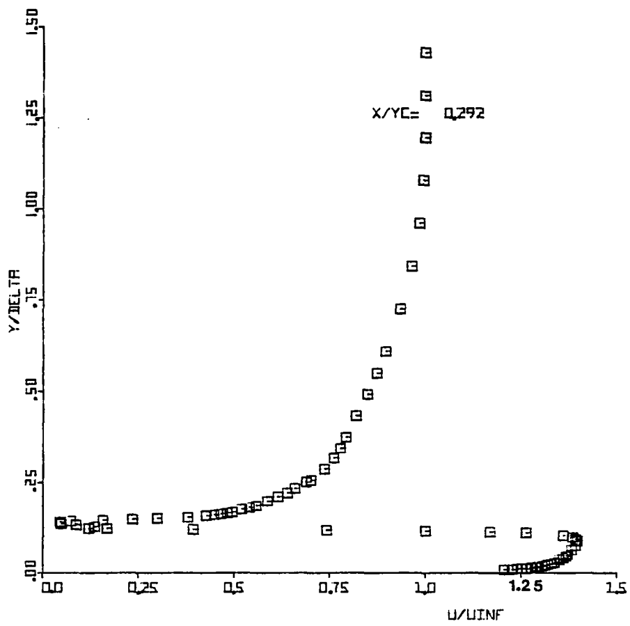
Fig. 4.4(b) Mean Velocity Profile at the Slot ( x/y_c = 0.292 )
