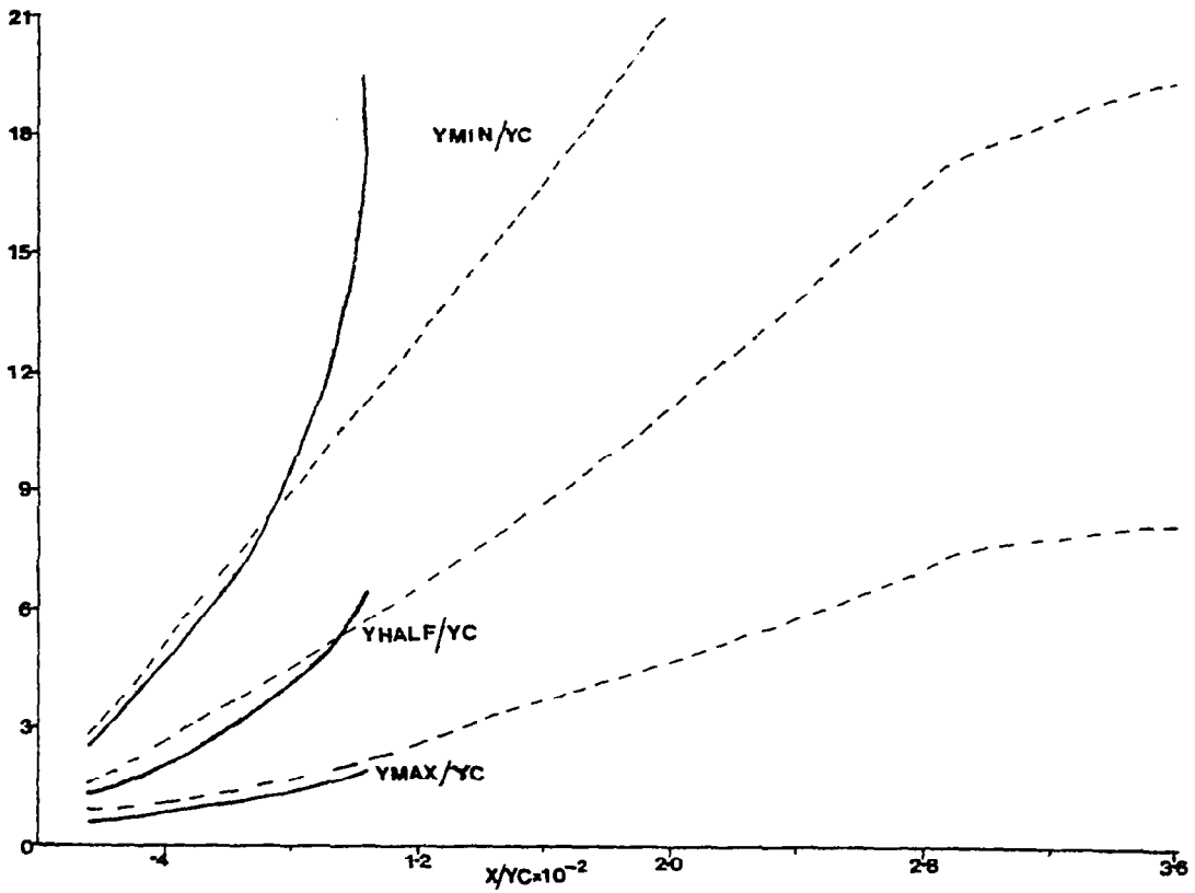
Fig. 7.4(g) Predicted Variation of the Profile Length Scales for the Adverse Pressure Gradient Flow
