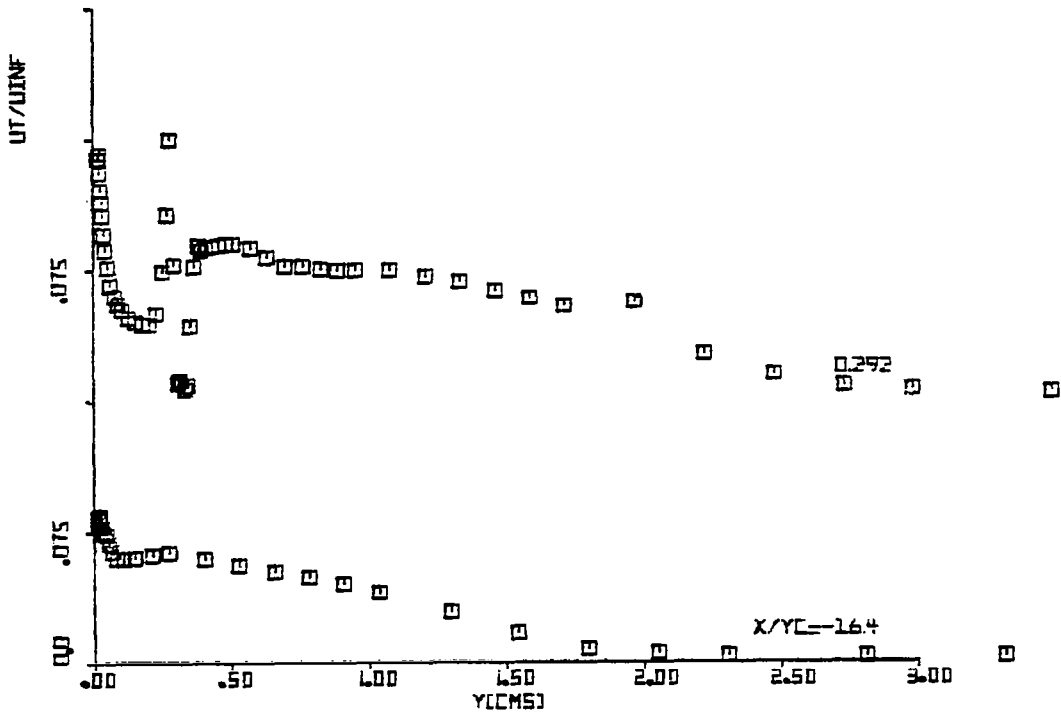
Fig. 5.9(a) Distribution of the Turbulence Intensity u_t/U_{\infty} at x/y_c = -16.4 and 0.292
