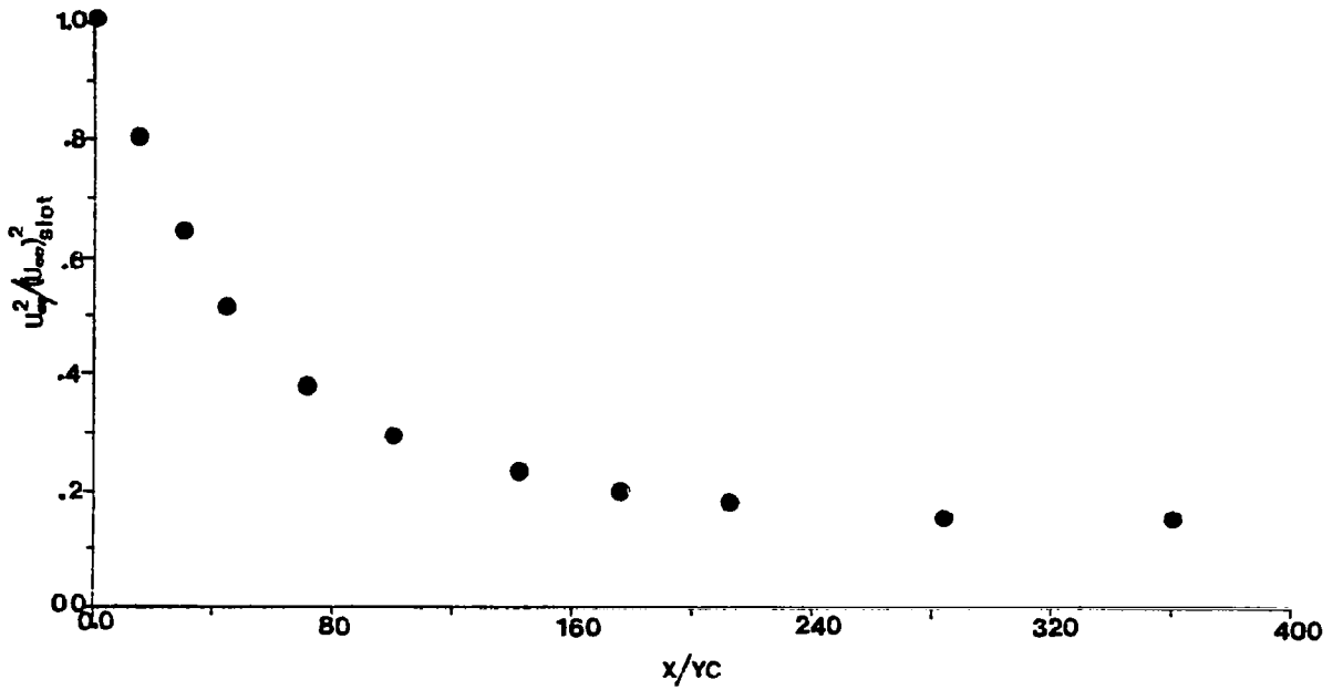
Fig. 5.2 Free-Stream Velocity Distribution
