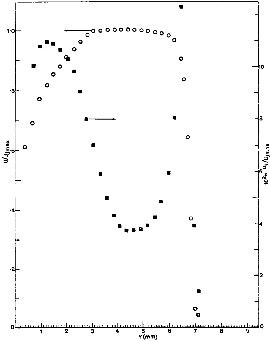
Fig. A-1 Mean Velocity and Turbulence Profiles at the Exit of the Jet (Bowles)
