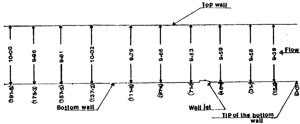
Fig. 4.1 Position of the Top Wall for the Zero Pressure Gradient Flow
