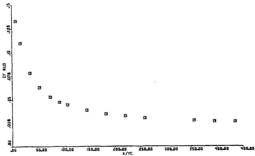
Fig. 4.3(a) Variation of Skin Friction
