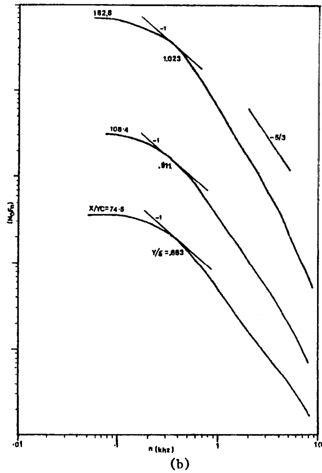
Fig. 4.23 Spectra of u^2 Representing the Outer Layer at Different Stations
