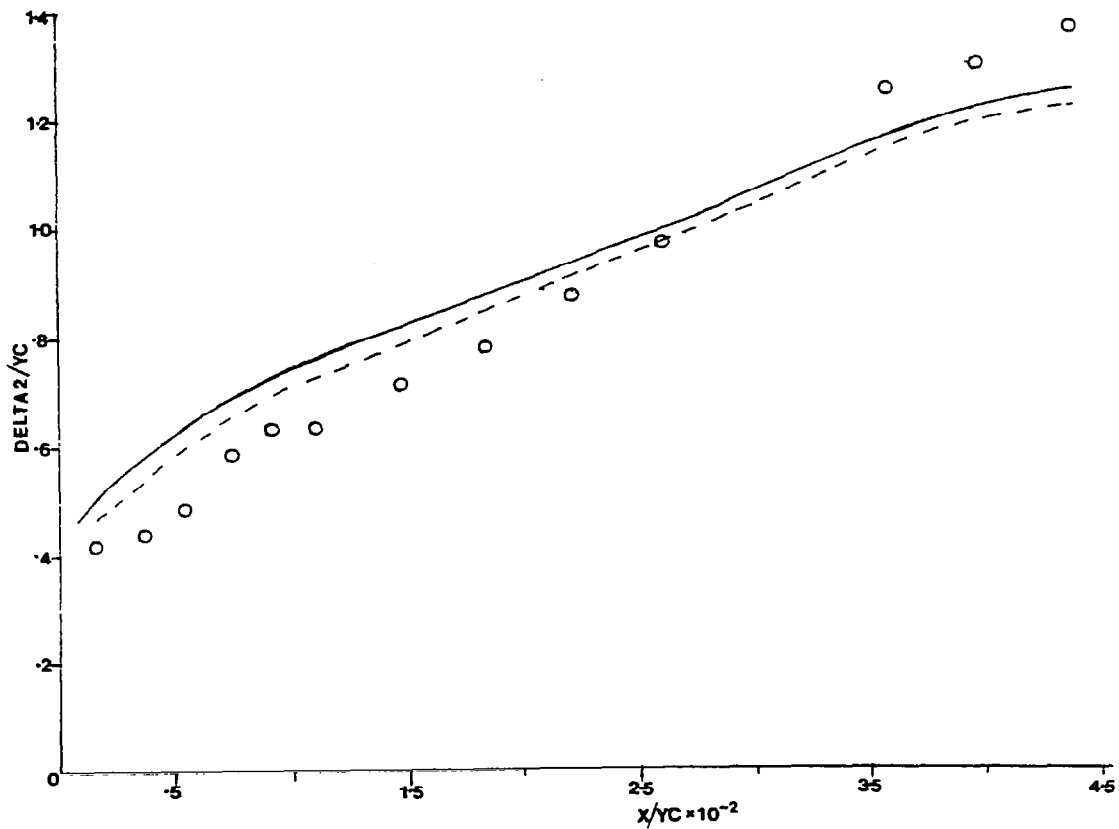
Fig. 7.1(c) Predicted Development of the Momentum Thickness for the Zero Pressure Gradient Flow
