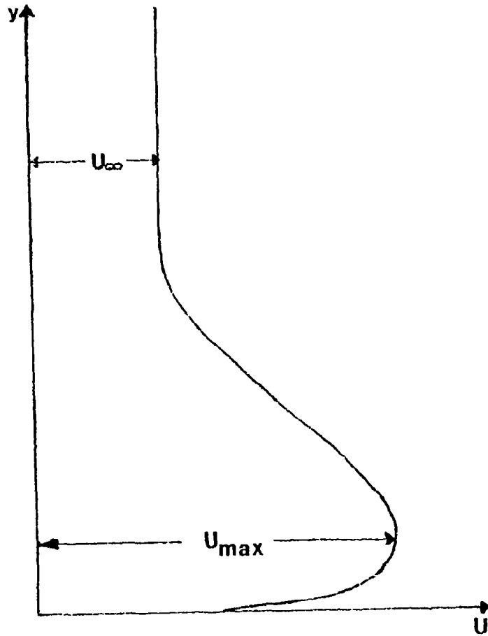
Fig. 1.1(a) Velocity Profile for a "Simple" Wall Jet
