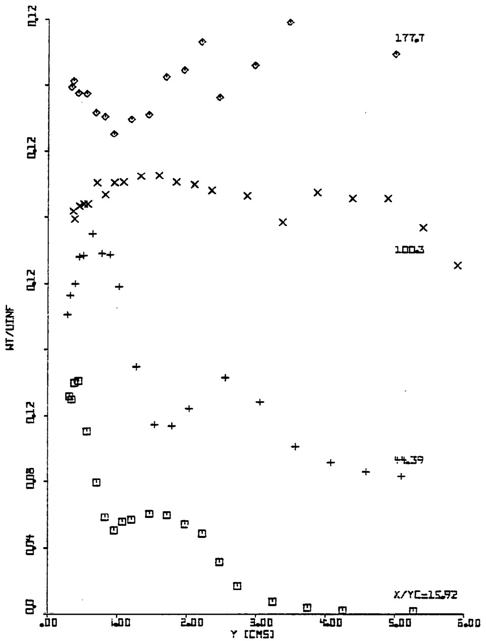
Fig. 5.12 Distributions of the Turbulence Intensity w_t/U_\infty
