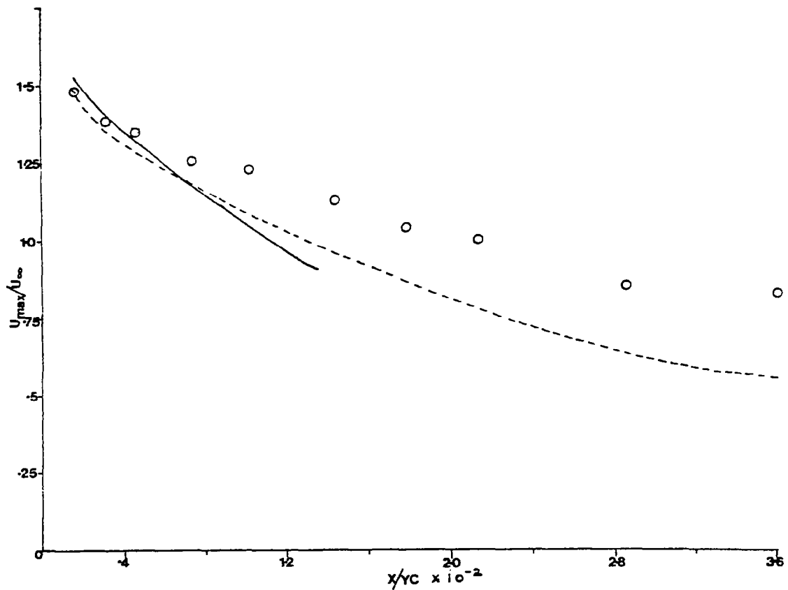
Fig. 7.2(e) Predicted Variation of U_{max} for the Adverse Pressure Gradient Flow
