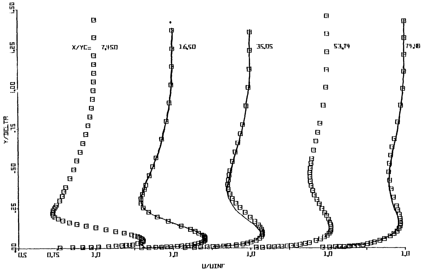
Fig. 4.4(c) Mean Velocity Profiles at x/y_c = 7.45 to 74.48
