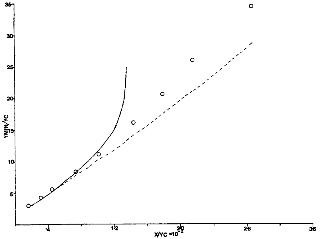
Fig. 7.2(g) Predicted Variation of Y_{\min} for the Adverse Pressure Gradient Flow
