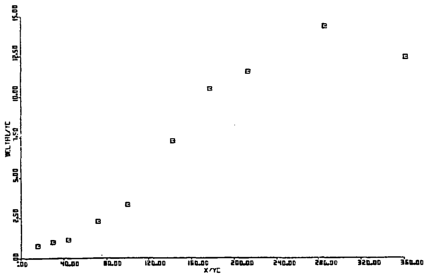
Fig. 5.6(b) Growth of the Displacement Thickness
