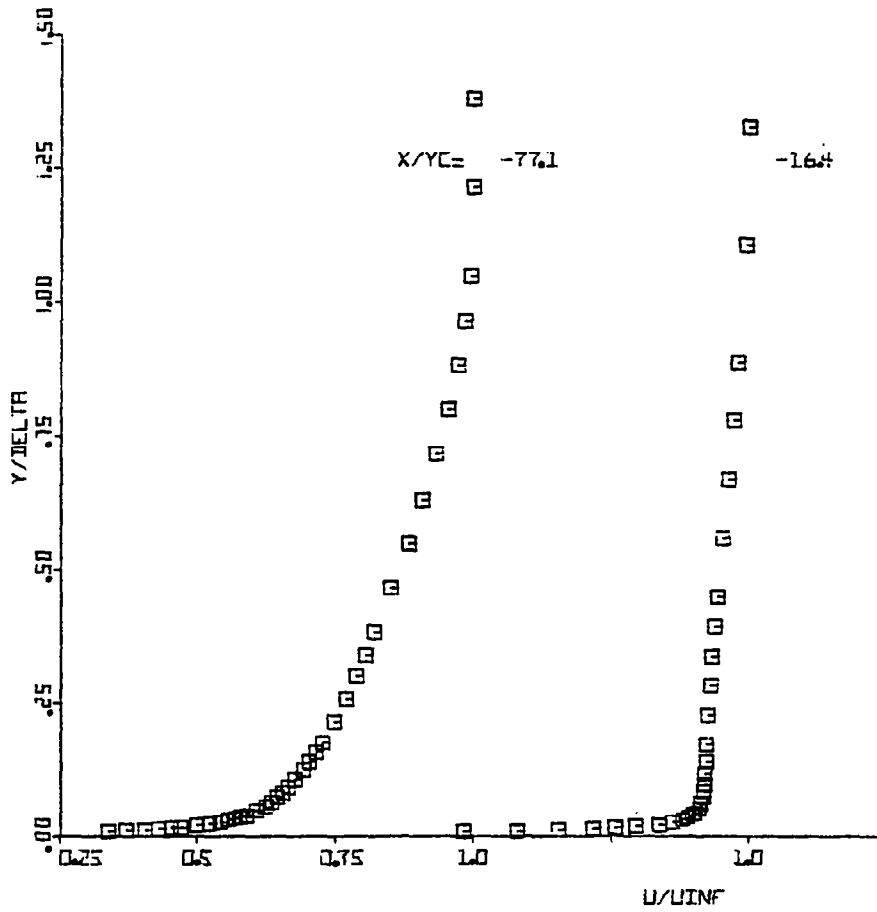
Fig. 4.4(a) Mean Velocity Profiles Upstream of the Slot ( x/y_c = -77.1 and -16.4 )
