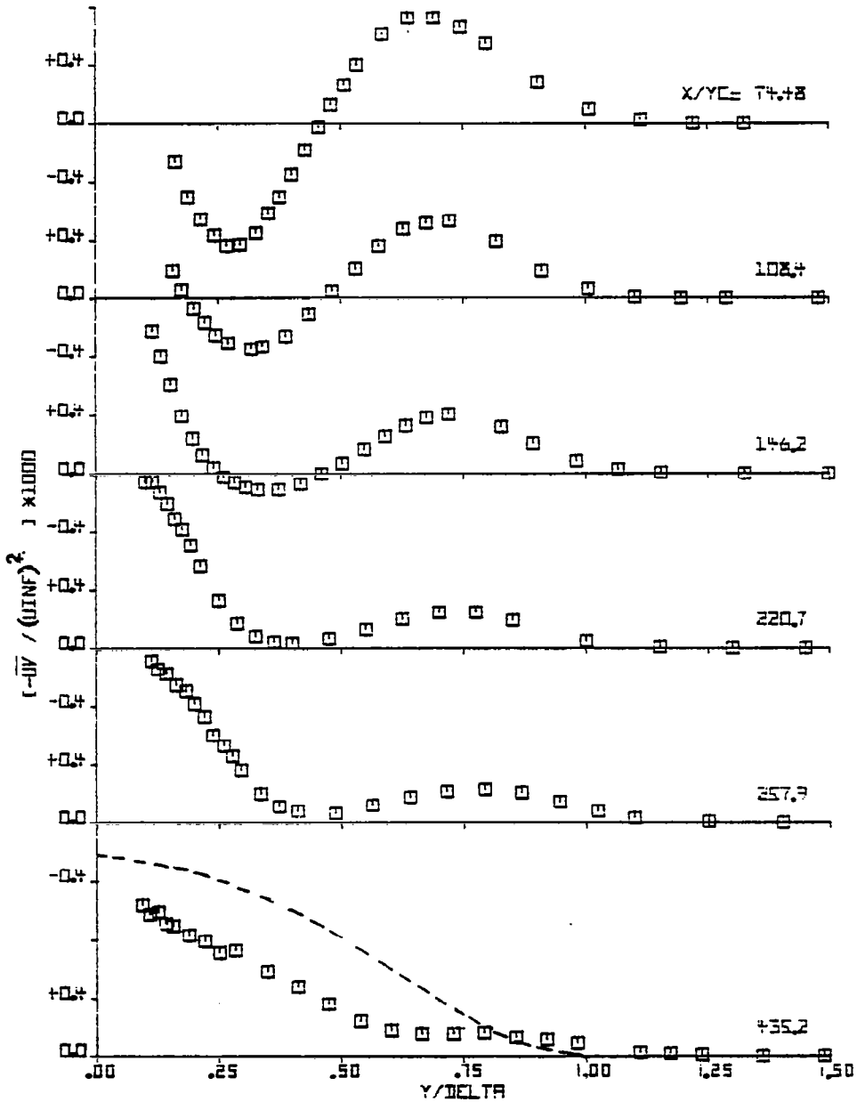
Fig. 4.13(b) Distribution of the Shear Stress at x/y_c = 74.48 to 435.2
