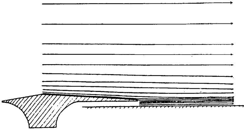
Fig. 4.5(c) Streamline Pattern Around the Slot Lip
