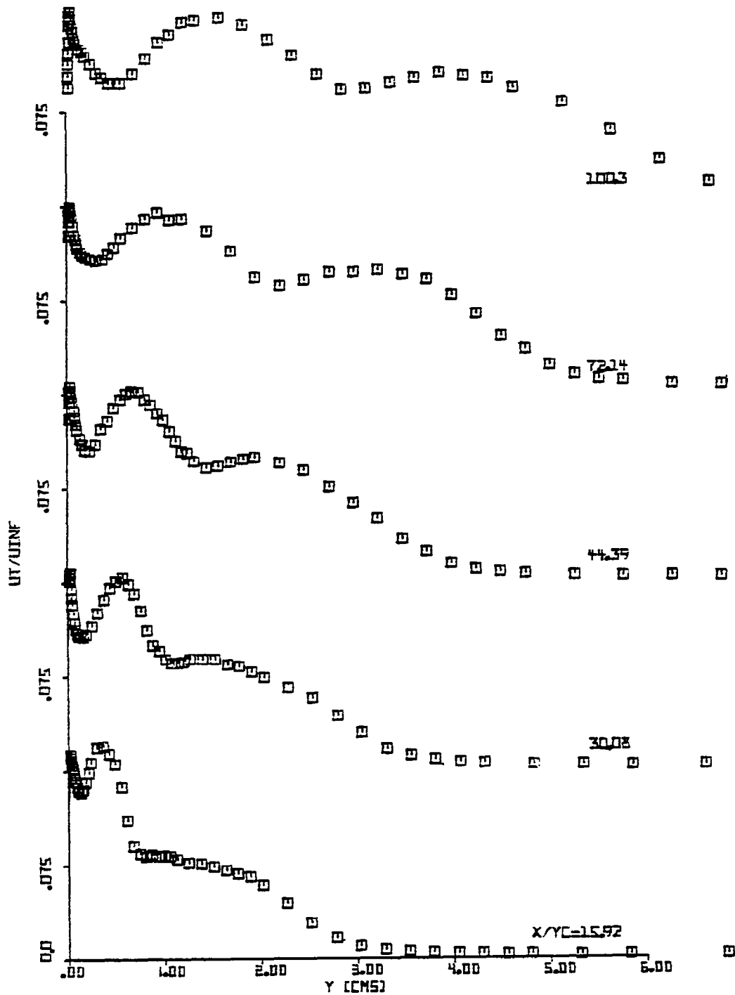
Fig. 5.9(b) Distribution of the Turbulence Intensity u_t/U_\infty at x/y_c = 15.92 to 100.3
