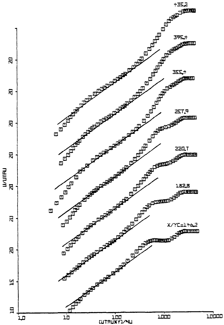
Fig. 4.5(b) Mean Velocity Profiles in the Wall Coordinates at x/y_c = 146.2 to 435.2
