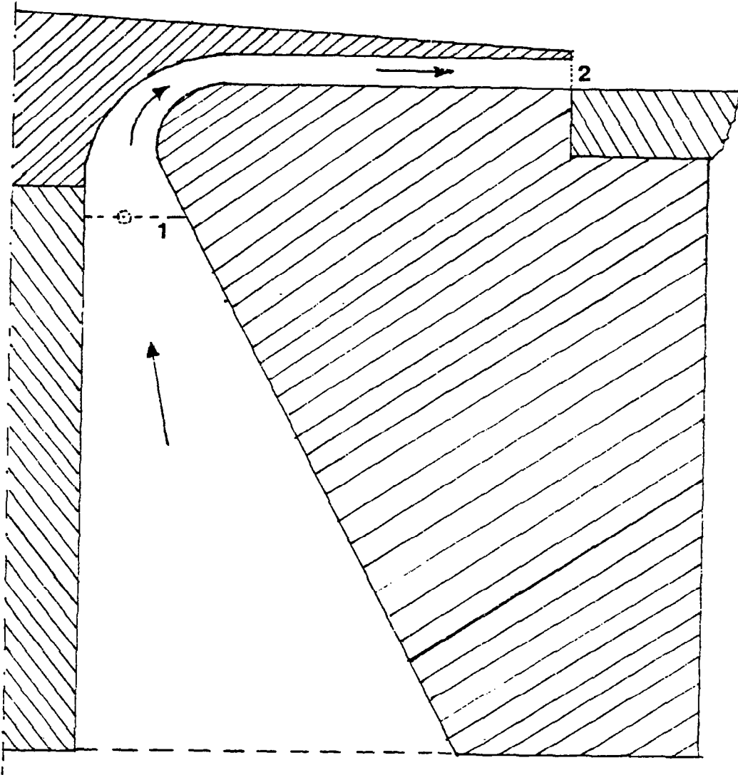
Fig. B-1 Close-up View of the Jet Nozzle
