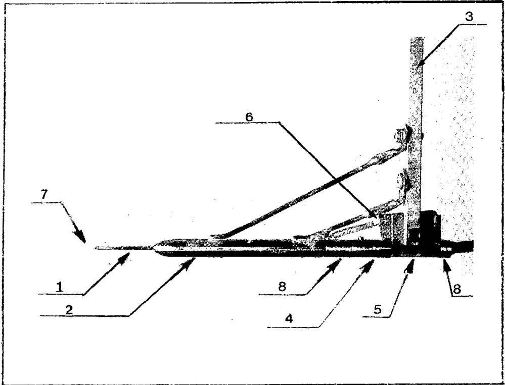
Fig. 3.2 Slant-Wire Rotating Mechanism with the Probe Mounted on It.
