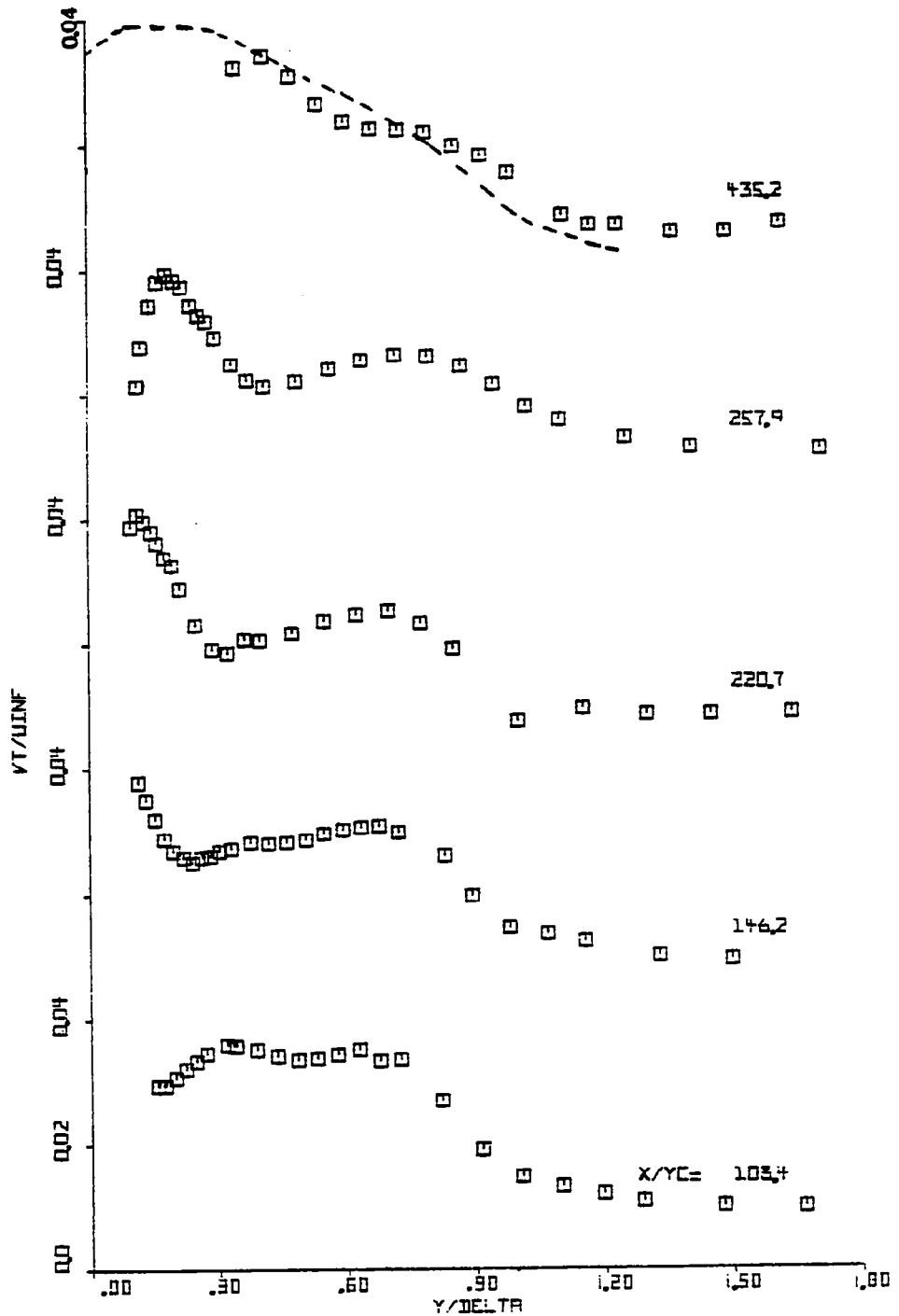
Fig. 4.11(b) Distribution of the Turbulence Intensity v_t/U_\infty at x/y_c = 108.4 to 435.2
