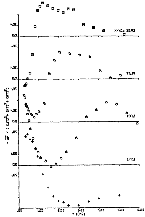
Fig. 5.16 Variation of the Correlation Function a_1
