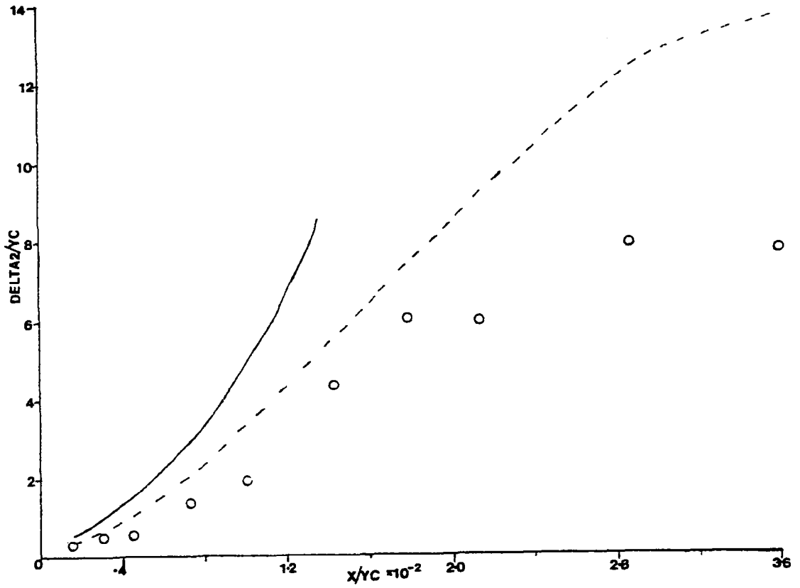
Fig. 7.2(c) Predicted Development of the Momentum Thickness for the Adverse Pressure Gradient Flow
