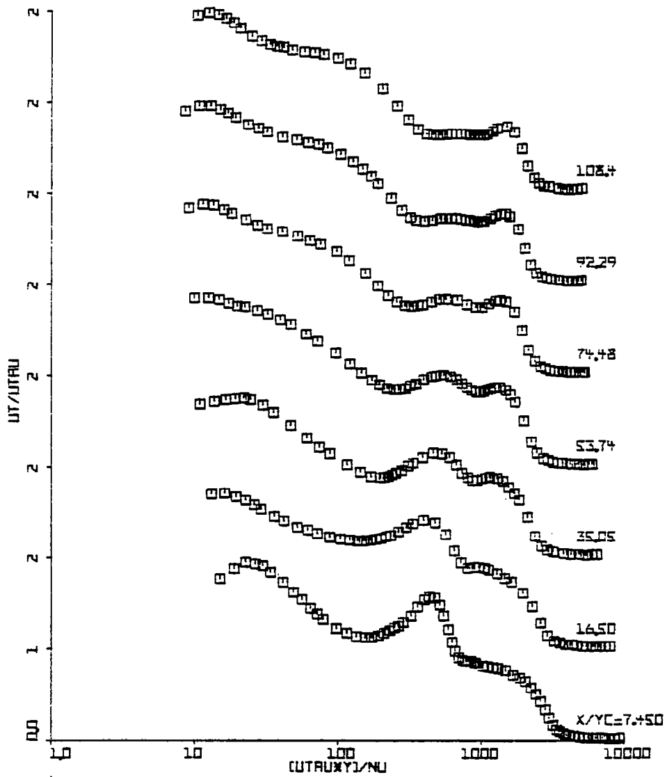
Fig. 4.10(a) Distribution of u_t in the Wall Coordinates at x/y_c = 7.45 to 108.4
