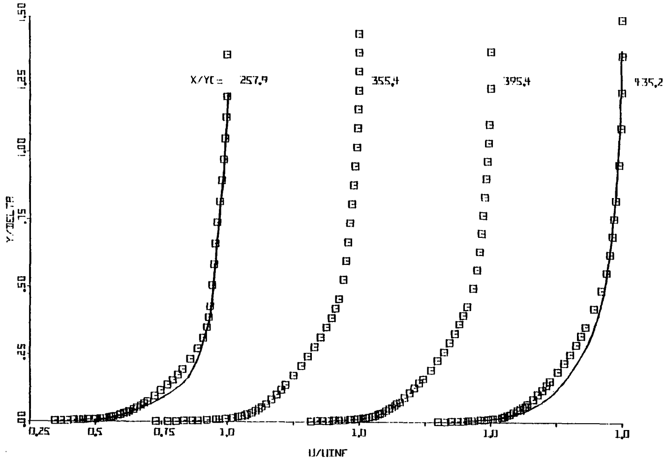
Fig. 4.4(e) Mean Velocity Profiles at x/y_c = 257.9 to 435.2
