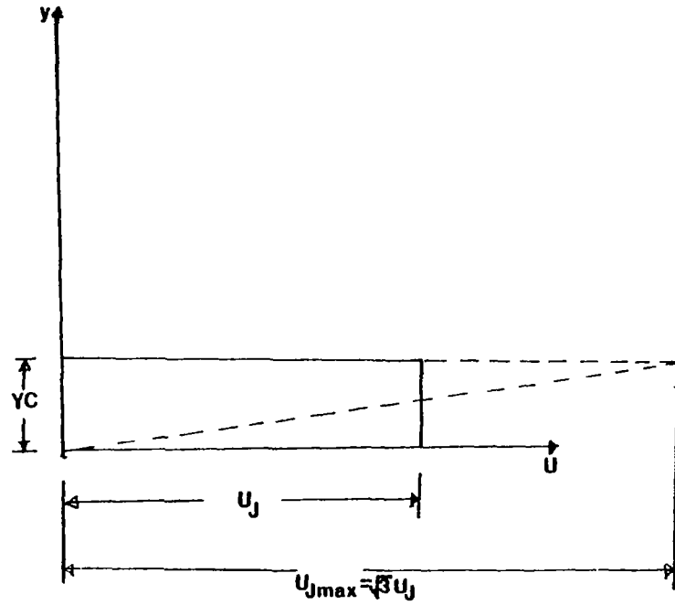
Fig. 7.3(c) Comparison of Uniform and Linear Jet Velocity Profiles Without the Mixing Layer
