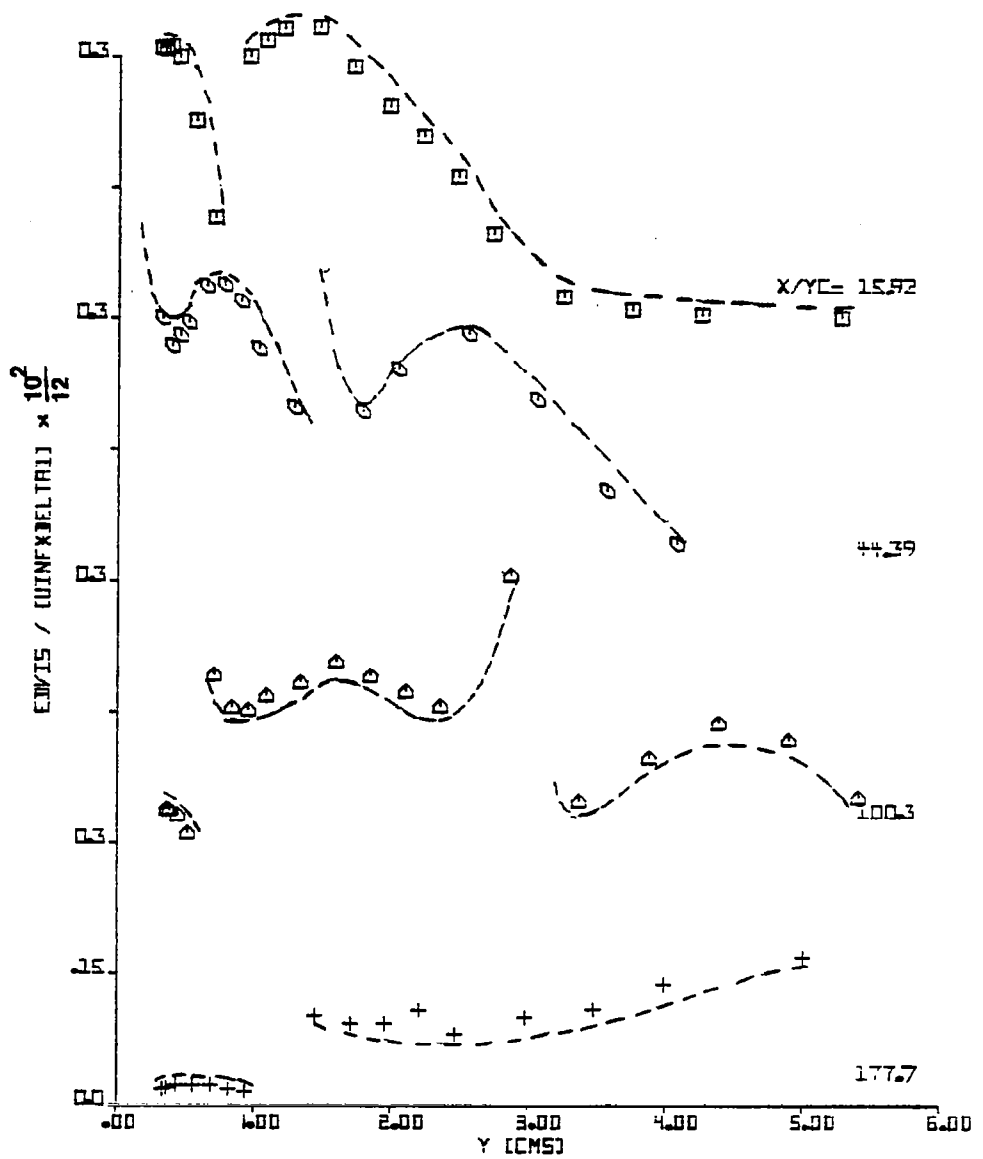
Fig. 5.17 Distributions of the Eddy Viscosity
