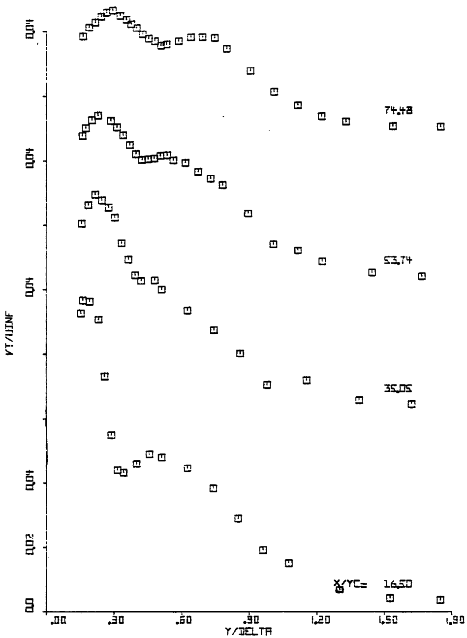
Fig. 4.11(a) Distribution of the Turbulence Intensity v_t/U_{\infty} at x/y_c = 16.5 to 74.48
