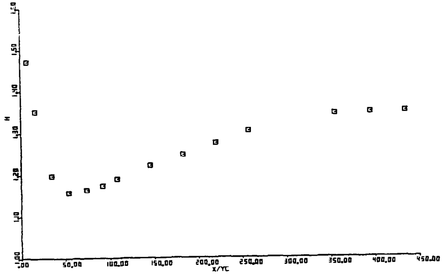
Fig. 4.6(d) Variation of the Shape Factor
