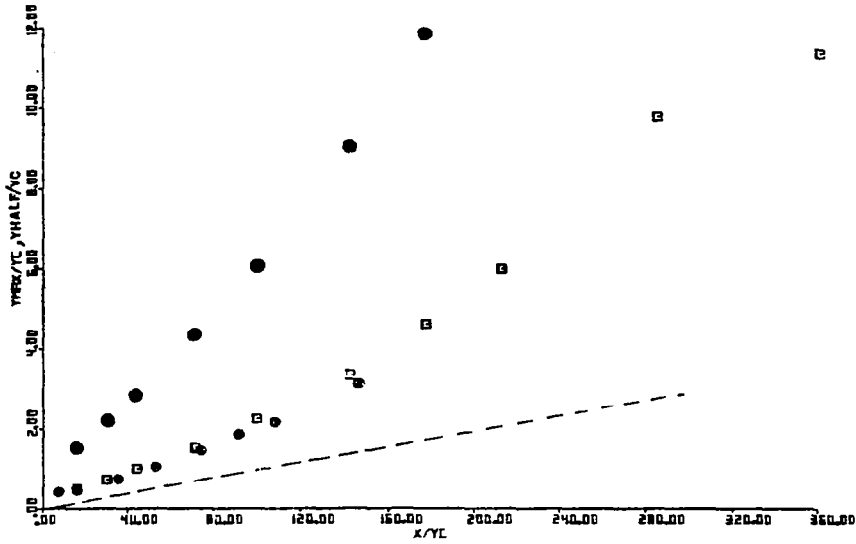
Fig. 5.7(a) Development of Y_{\max} and Y_{\text{half}}
