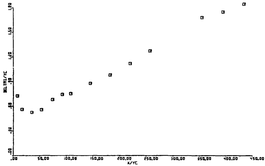
Fig. 4.6(b) Growth of the Displacement Thickness
