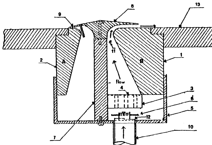
Fig. 2.5 Wall Jet Assembly
