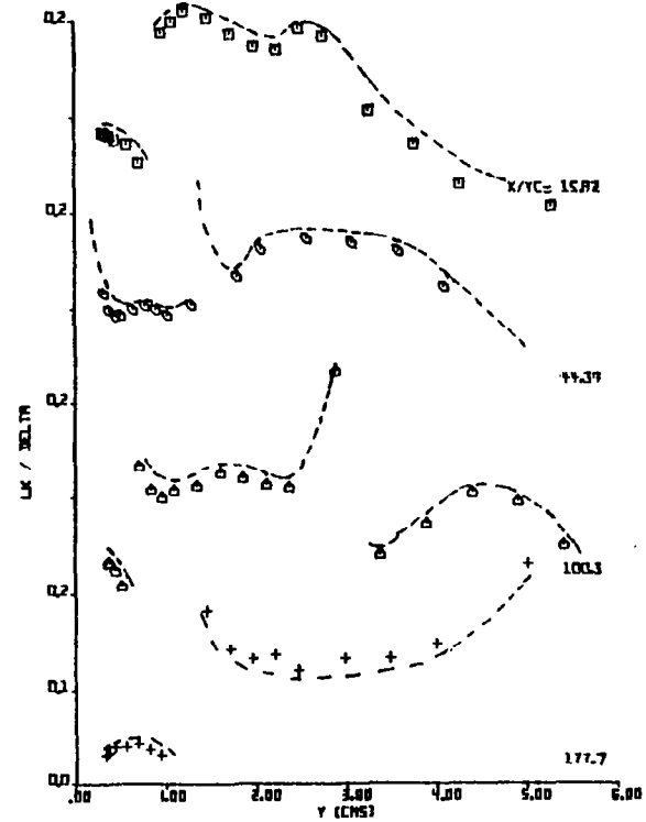
Fig. 5.19 Distributions of the Prandtl-Kolmogorov Length Scale L_k
