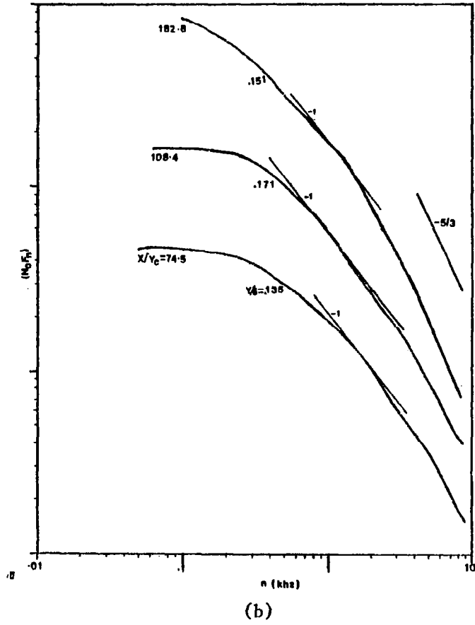
Fig. 4.22 Spectra of \overline{u^2} Representing the Inner Layer at Different Stations
