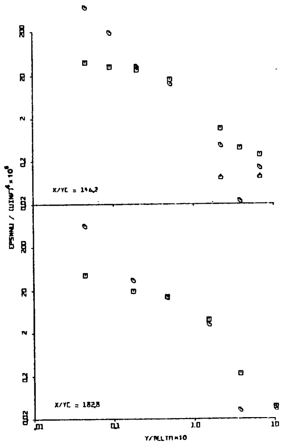
Fig. 4.24(c) Distribution of the Dissipation Rate at x/y_c = 146.2 to 257.9
