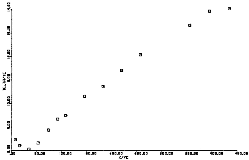
Fig. 4.6(a) Growth of the Boundary Layer Thickness
