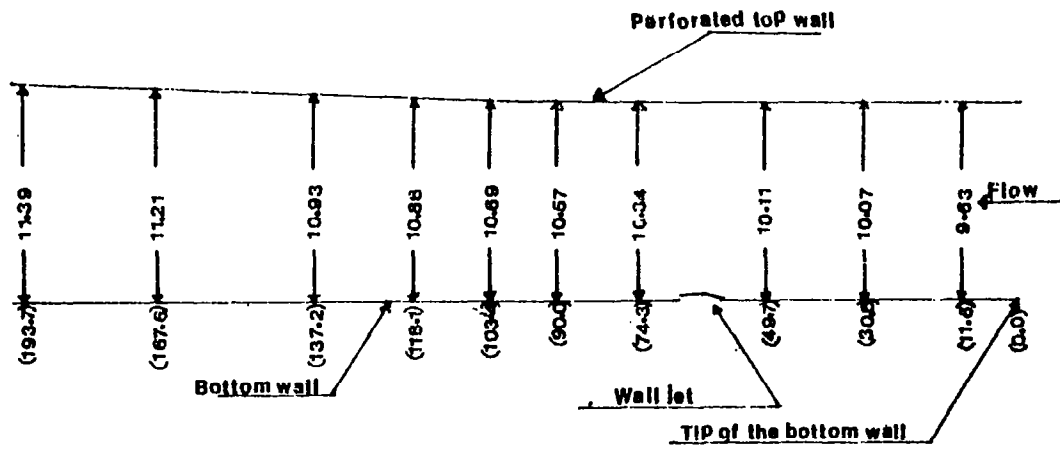
Fig. 5.1 Position of the Top Wall for the Adverse Pressure Gradient Flow
