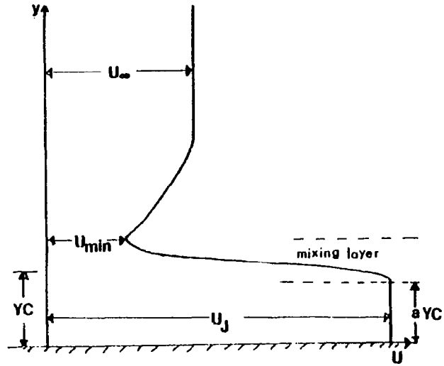
Fig. 7.3(a) Starting Velocity Profile for the Predictions with Uniform Jet Velocity Profile using the Automatic Starting Procedure
