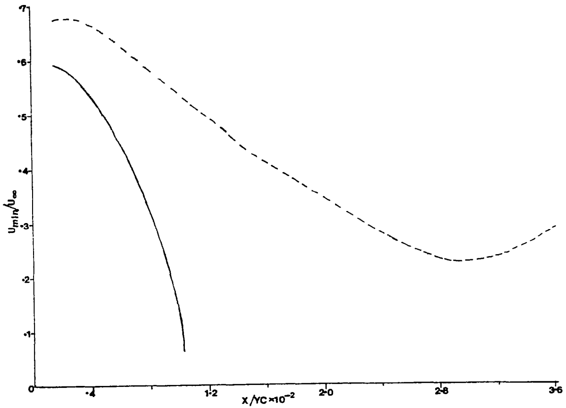
Fig. 7.4 (e) Predicted Variation of U_{min} for the Adverse Pressure Gradient Flow
