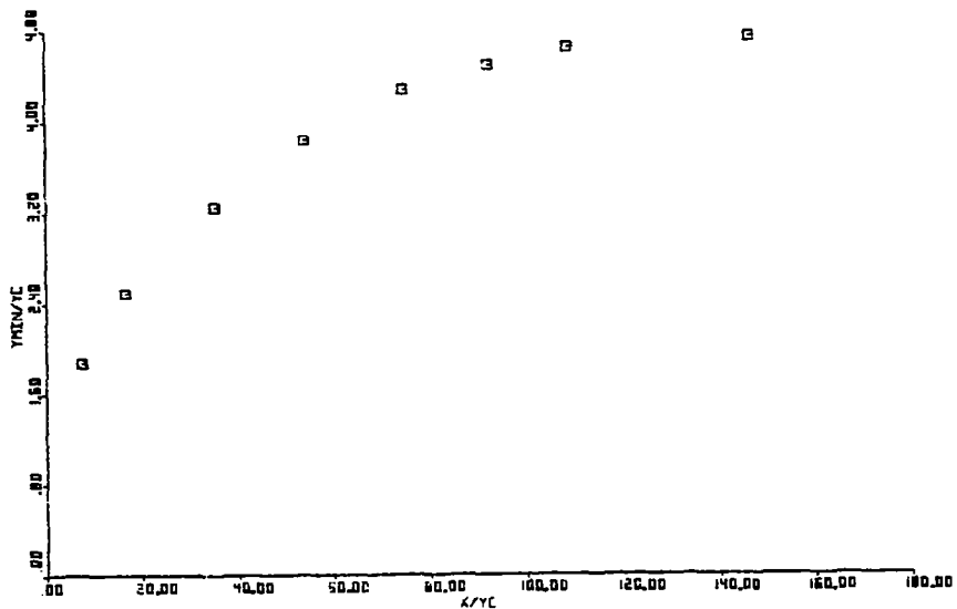
Fig. 4.7(b) Development of Y_{min}
