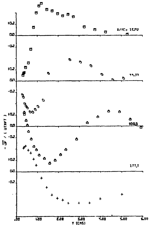
Fig. 5.15 Variation of the Correlation Function R_{uv}
