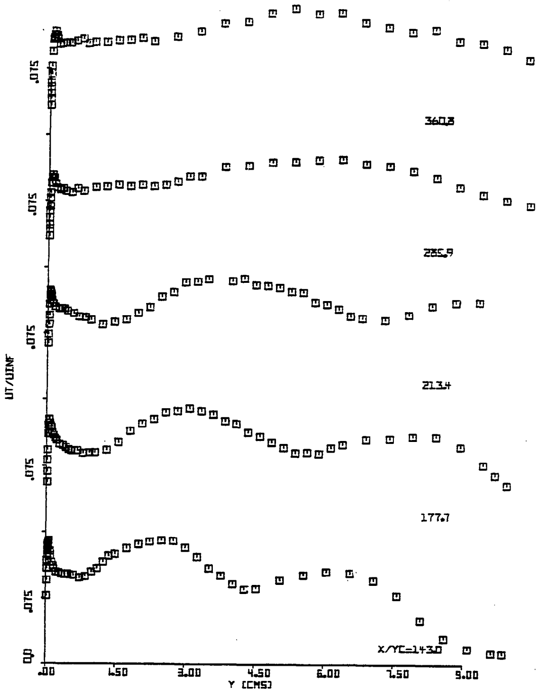
Fig. 5.9(c) Distribution of the Turbulence Intensity u_t/U_\infty at x/y_c = 143.0 to 360.8
