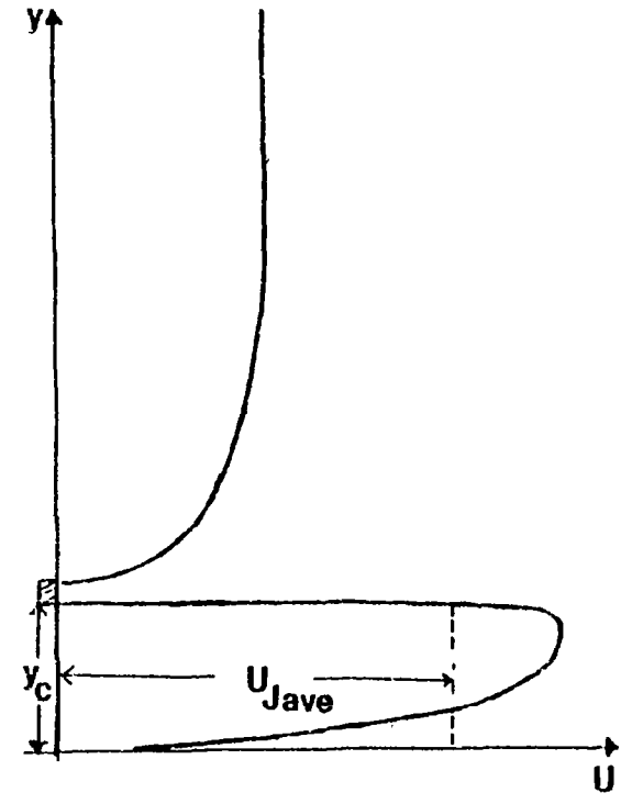
Fig. 1.2(c) Asymmetric Jet Velocity Profile
