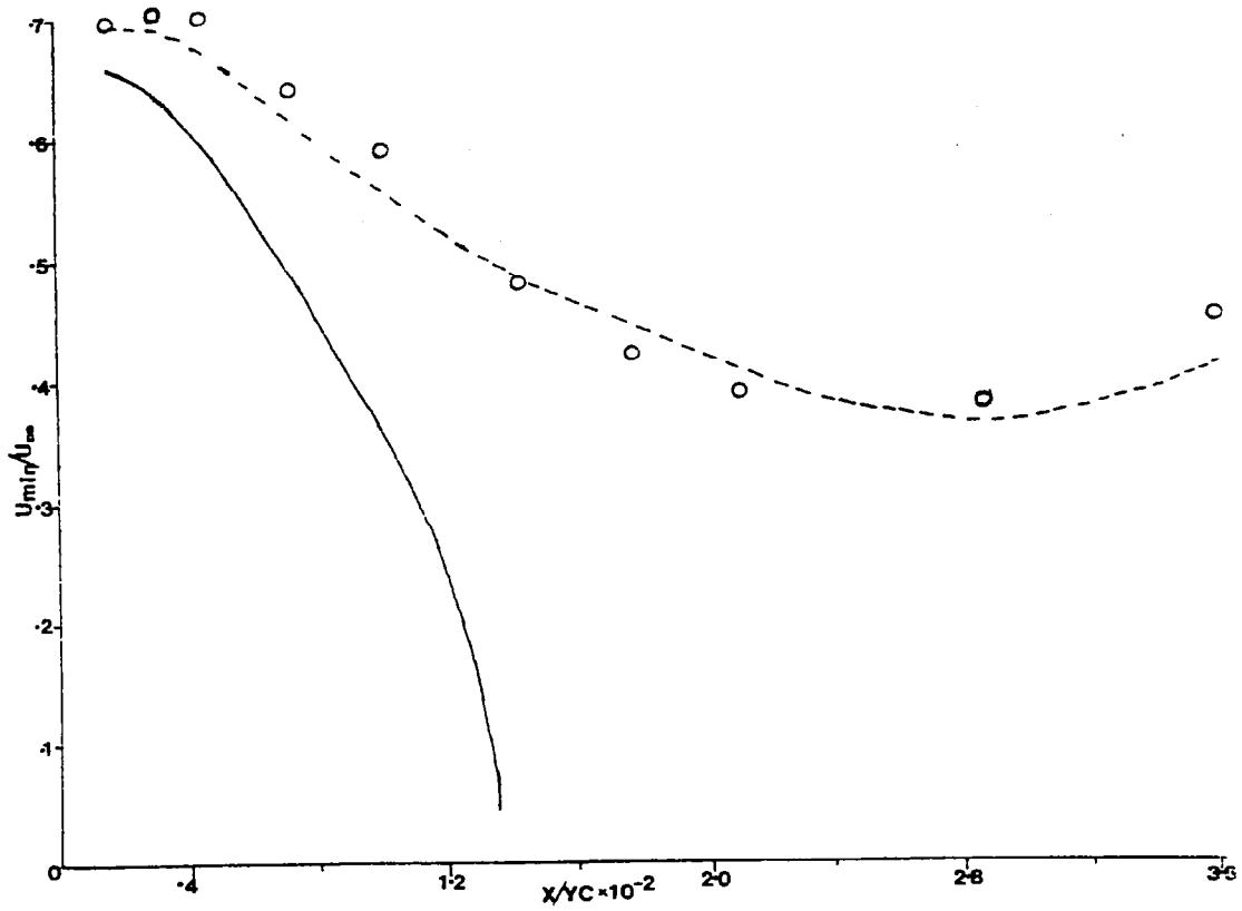
Fig. 7.2(f) Predicted Variation of U_{min} for the Adverse Pressure Gradient Flow
