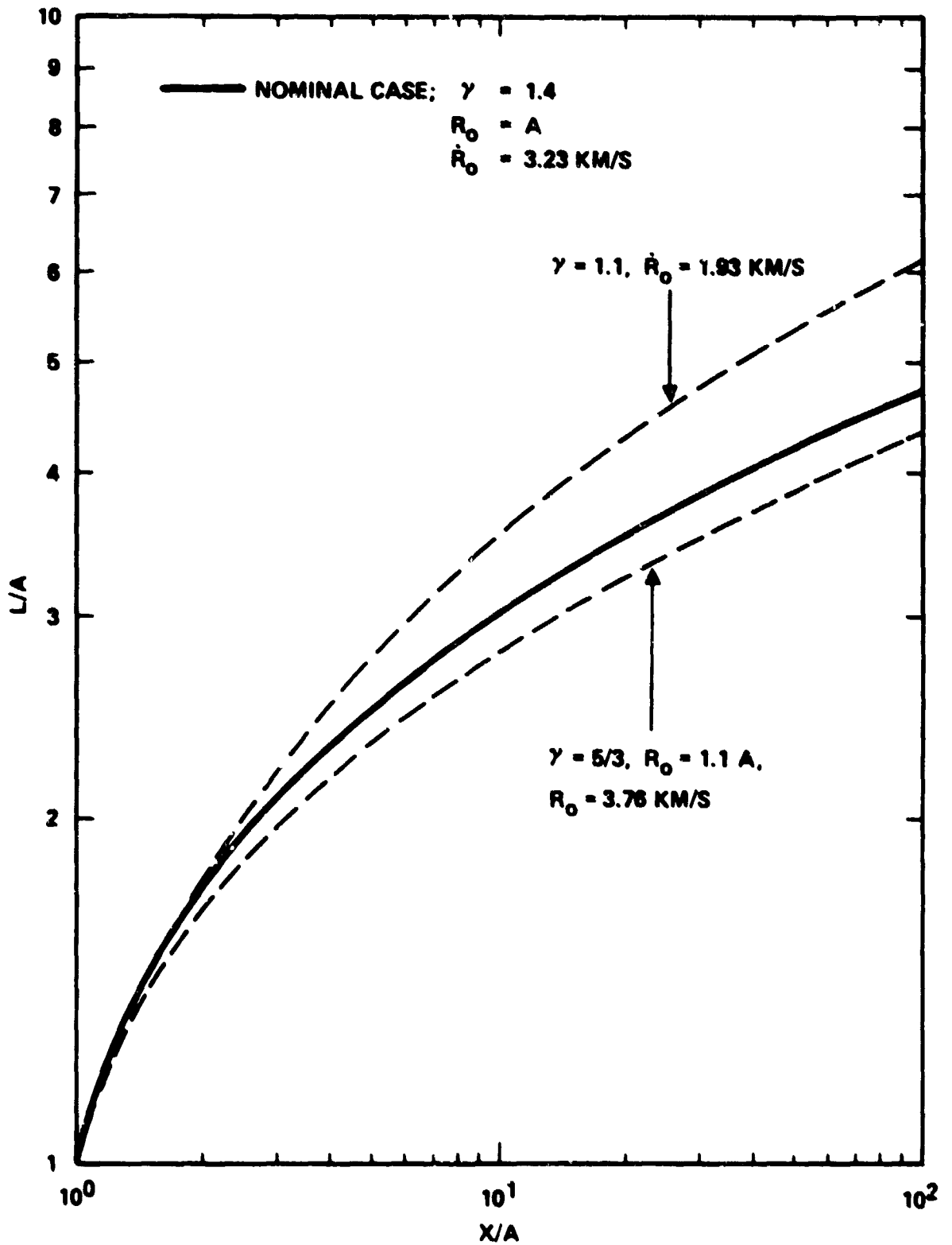
FIG. 20. Normalized travel distance versus normalized axial position for different values of the ratio of specific heats.
