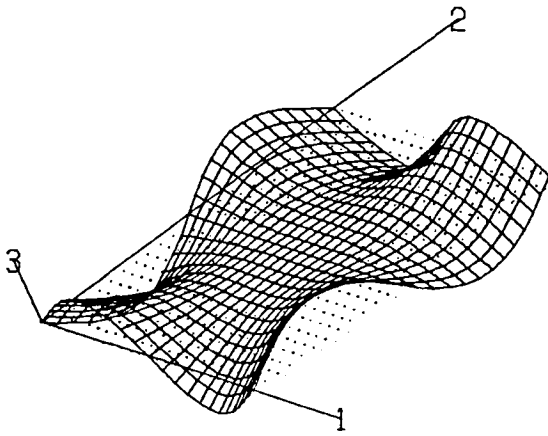
Mode 9 (0.0450 Hz)
