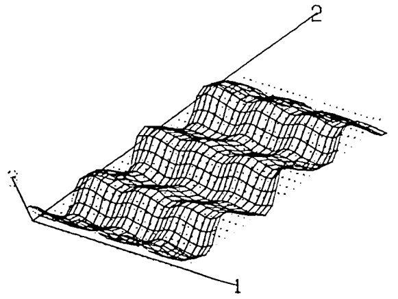
Mode 42 (0.270 Hz)
