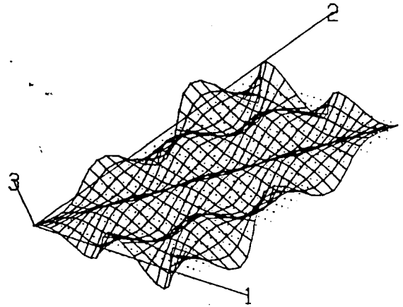
Mode 38 (0.237 Hz)
