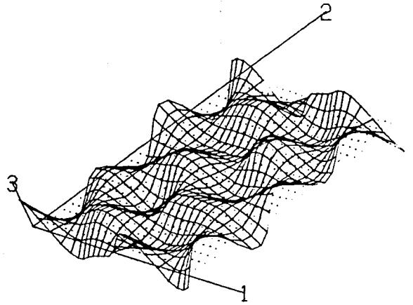
Mode 40 (0.256 Hz)
