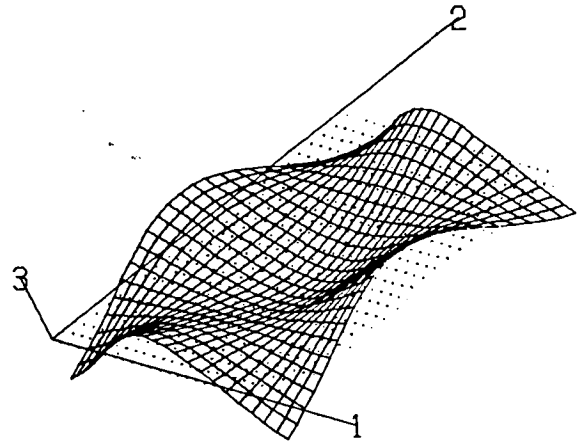
Mode 8 (0.0414 Hz)
