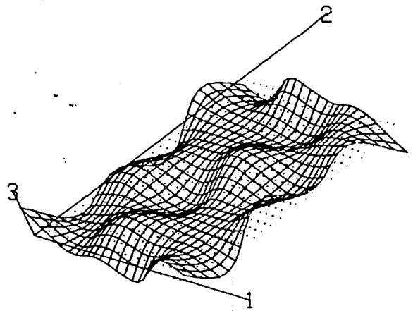
Mode 26 (0.158 Hz)
