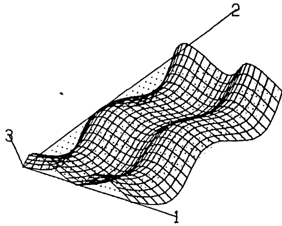
Mode 13 (0.0761 Hz)
