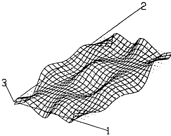
Mode 27 (0.158 Hz)
