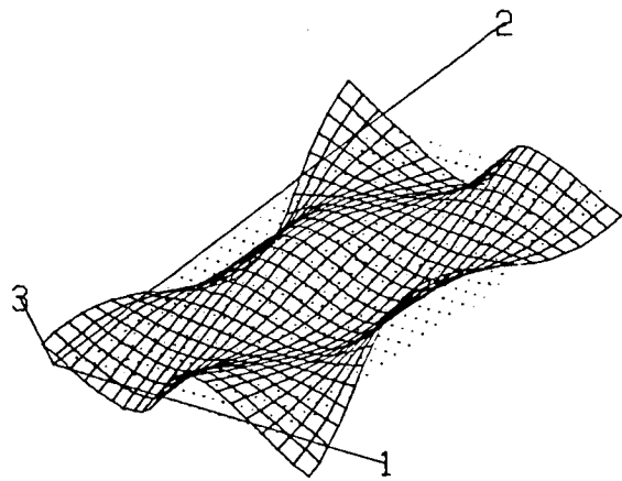
Mode 12 (0.0685 Hz)
