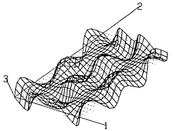
Mode 35 (0.219 Hz)
