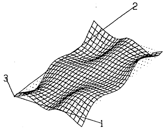
Mode 16 (0.0854 Hz)
