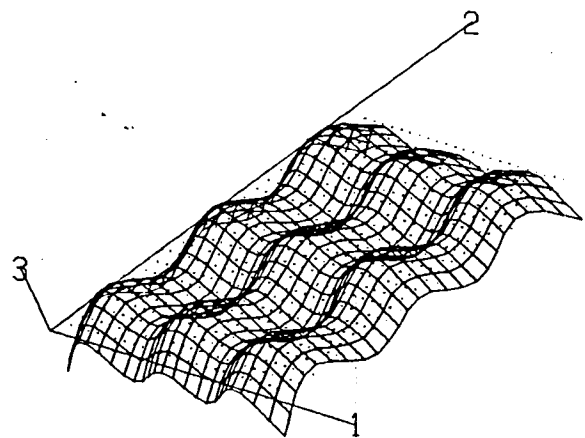
Mode 32 (0.195 Hz)
