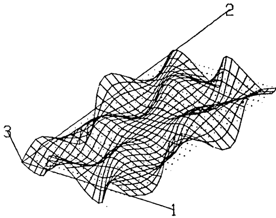
Mode 29 (0.190 Hz)
