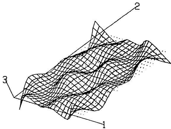
Mode 31 (0.194 Hz)
