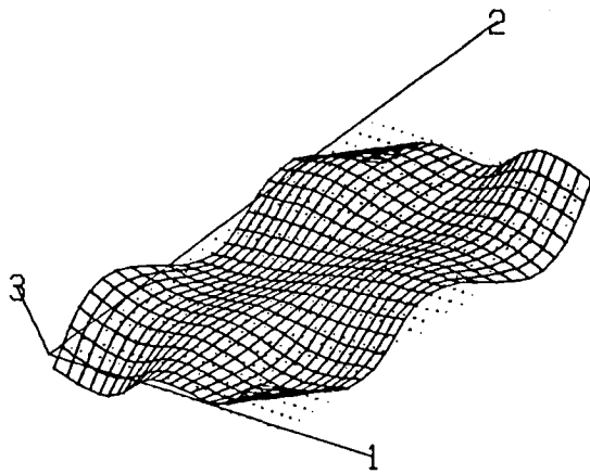
Mode 15 (0.0854 Hz)
