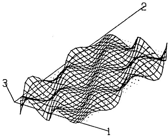
Mode 37 (0.237 Hz)
