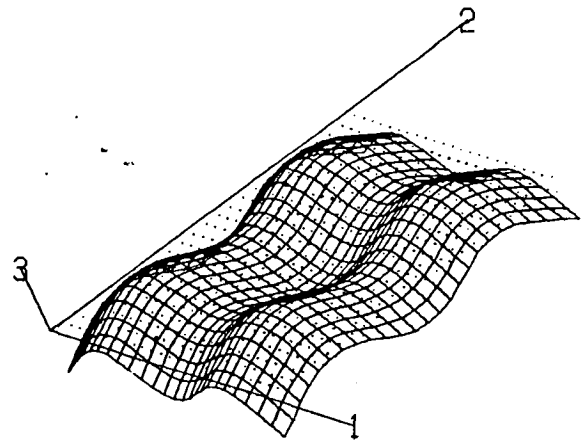
Mode 14 (0.0796 Hz)
