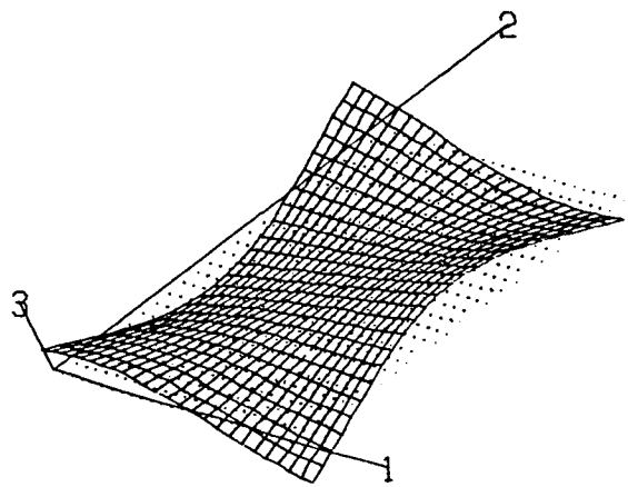
Mode 5 (0.0226 Hz)
