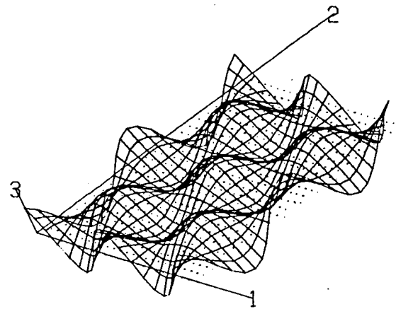
Mode 28 (0.183 Hz)
