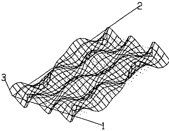
Mode 39 (0.256 Hz)
