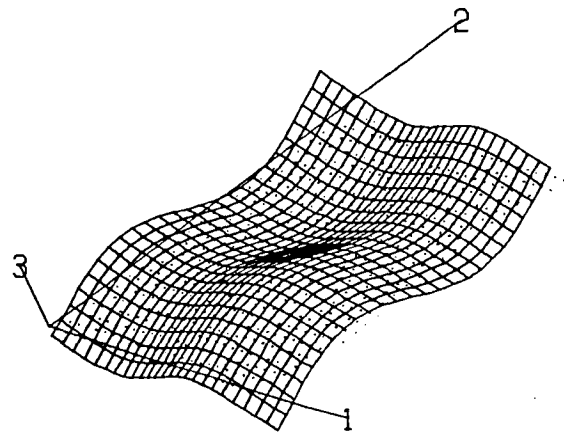
Mode 6 (0.0397 Hz)
