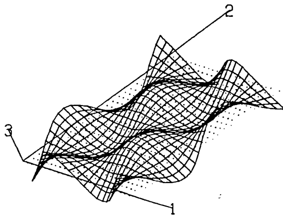
Mode 17 (0.0993 Hz)
