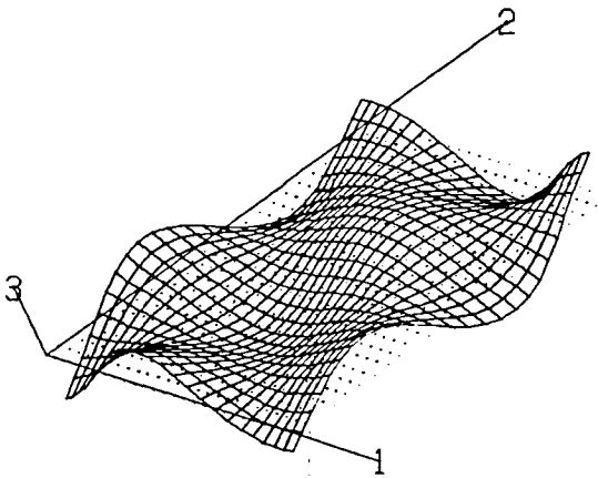
Mode 11 (0.0685 Hz)
