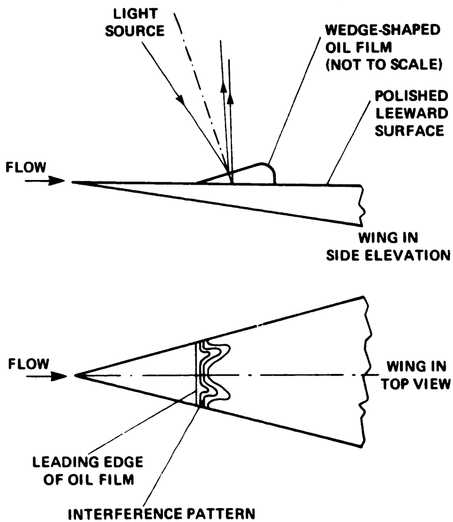
Figure 27.- Schematics of reflection on thin films.
